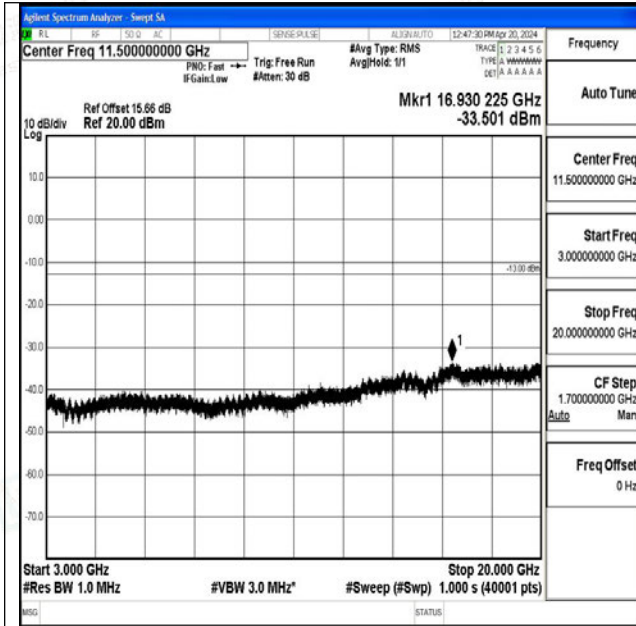
Band25_15MHz_QPSK_26615_1RB#0_3000~20000_30 00~20000
