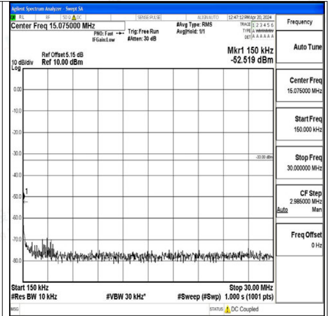
Band25_15MHz_QPSK_26615_1RB#0_0.15~30_0.15~3 0
