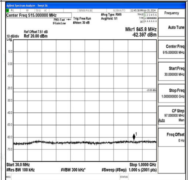
Band25_15MHz_16QAM_26115_1RB#0_30~1000_30~1 000
