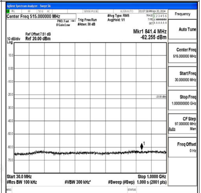
Band25_20MHz_16QAM_26365_1RB#0_30~1000_30~1 000
