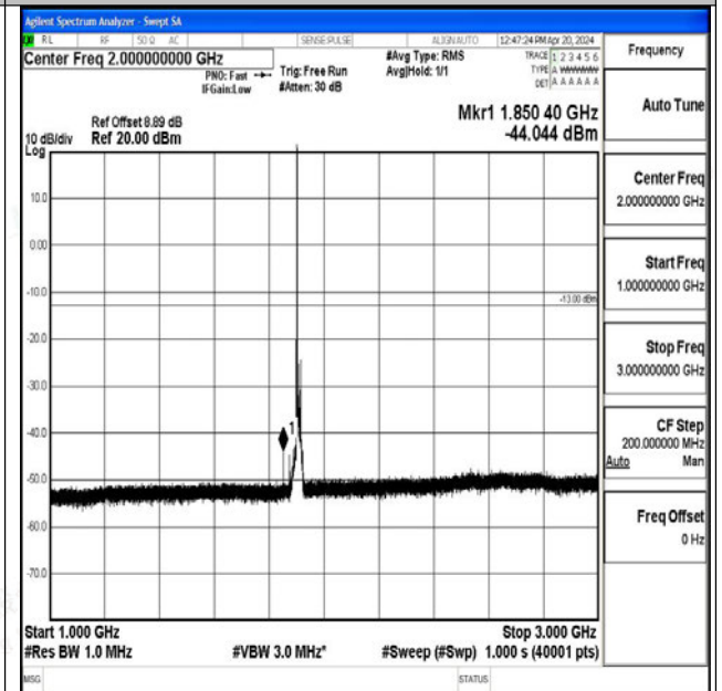
Band25_15MHz_QPSK_26615_1RB#0_1000~3000_100 0~3000
