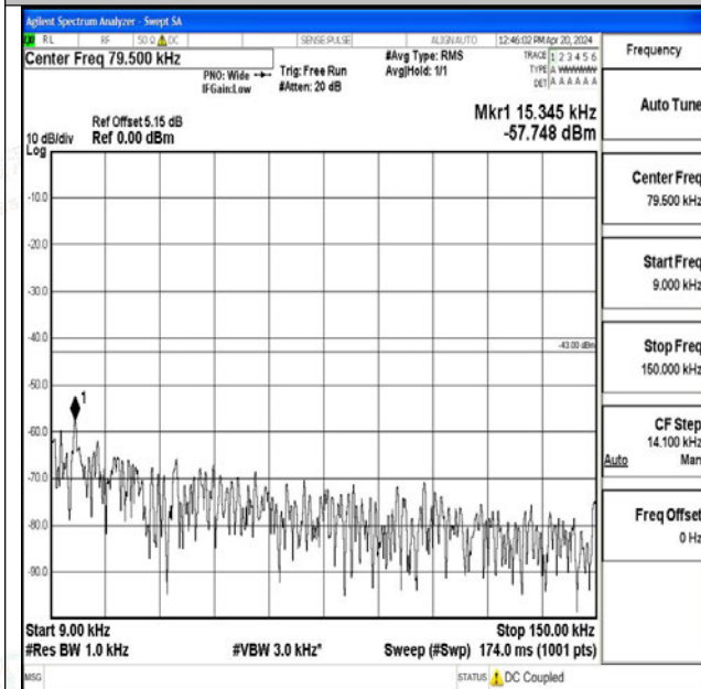
Band25_15MHz_QPSK_26365_1RB#0_0.009~0.15_0.009~0.15
