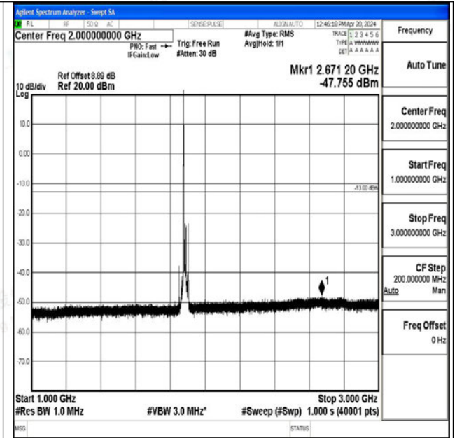
Band25_15MHz_QPSK_26365_1RB#0_1000~3000_1000~3000
