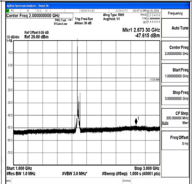
Band25_20MHz_QPSK_26365_1RB#0_1000~3000_100 0~3000
