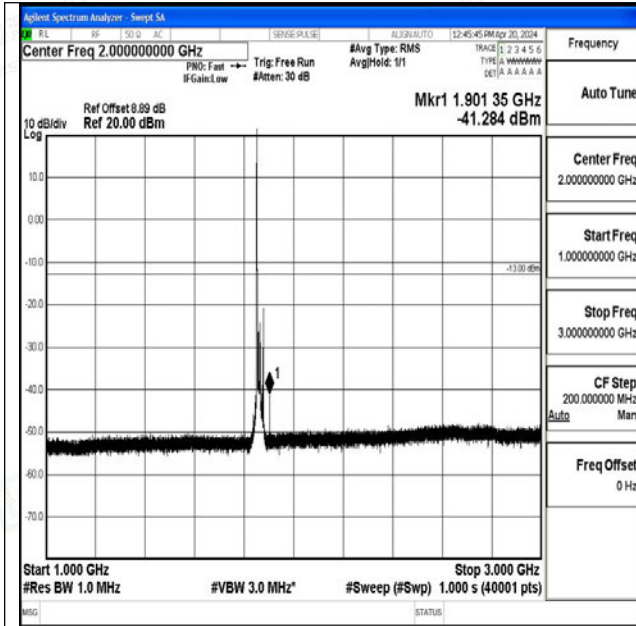
Band25_15MHz_16QAM_26115_1RB#0_1000~3000_1000~3000
