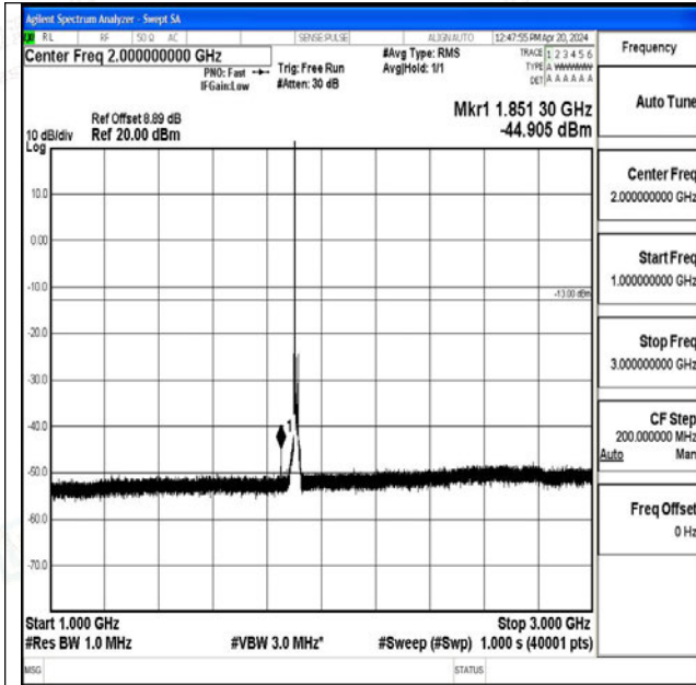
Band25_15MHz_16QAM_26615_1RB#0_1000~3000_1000~3000
