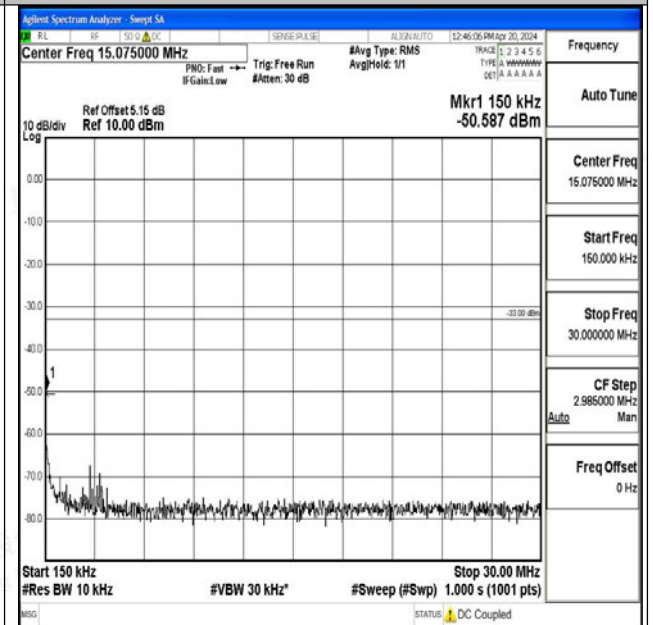
Band25_15MHz_QPSK_26365_1RB#0_0.15~30_0.15~30
