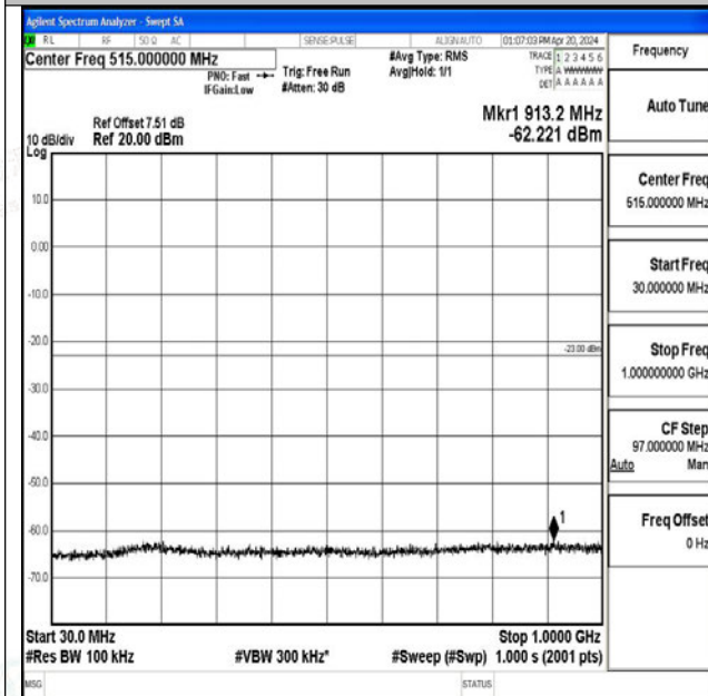
Band25_20MHz_QPSK_26365_1RB#0_30~1000_30~10 00
