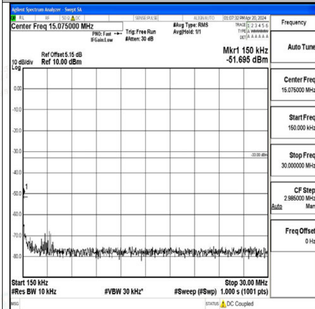
Band25_20MHz_16QAM_26365_1RB#0_0.15~30_0.15~ 30
