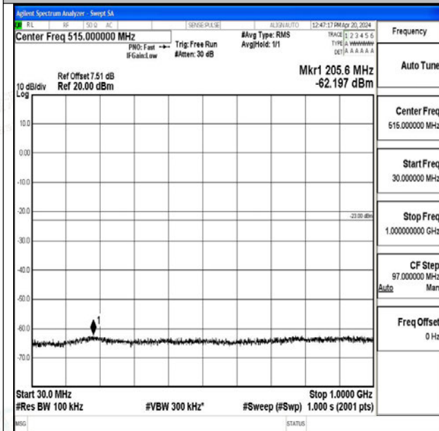
Band25_15MHz_QPSK_26615_1RB#0_30~1000_30~10 00
