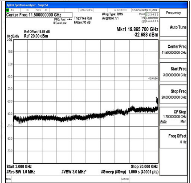
Band25_15MHz_16QAM_26115_1RB#0_3000~20000_3000~20000
