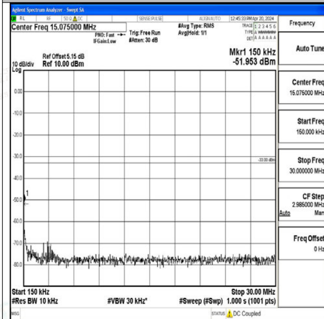
Band25_15MHz_16QAM_26115_1RB#0_0.15~30_0.15~ 30
