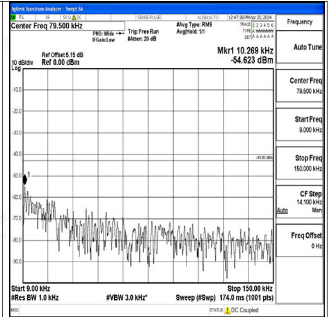
Band25_15MHz_16QAM_26615_1RB#0_0.009~0.15_0. 009~0.15
