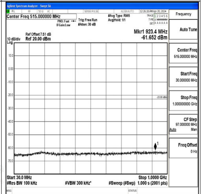
Band25_10MHz_16QAM_26365_1RB#0_30~1000_30~1 000
