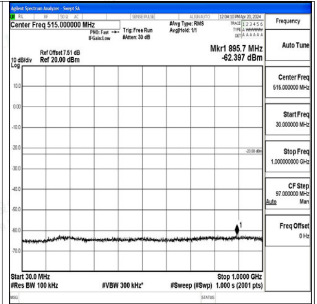
Band25_5MHz_16QAM_26365_1RB#0_30~1000_30~10
