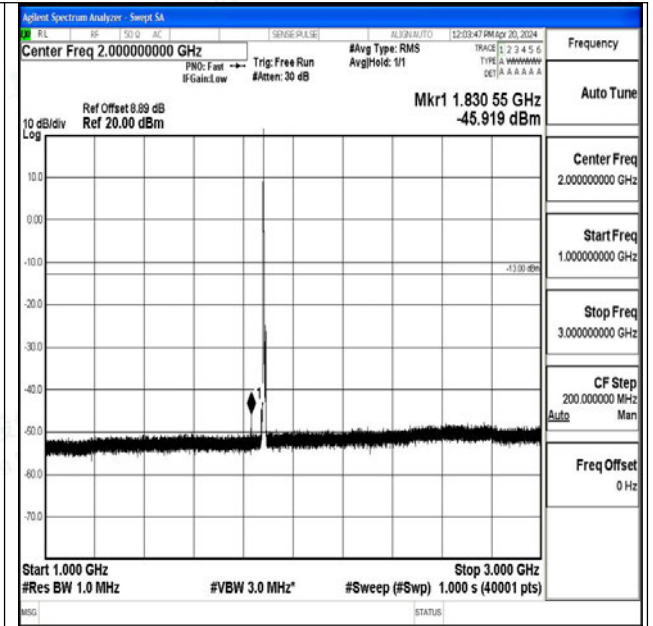
Band25_5MHz_QPSK_26365_1RB#0_1000~3000_1000
