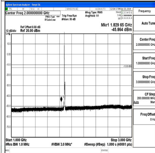
Band25_5MHz_16QAM_26365_1RB#0_1000~3000_1000~3000
