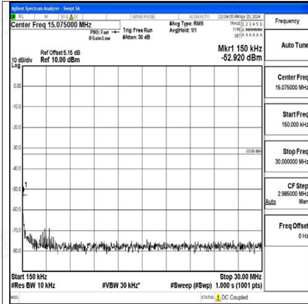
Band25_5MHz_16QAM_26365_1RB#0_0.15~30_0.15~3
