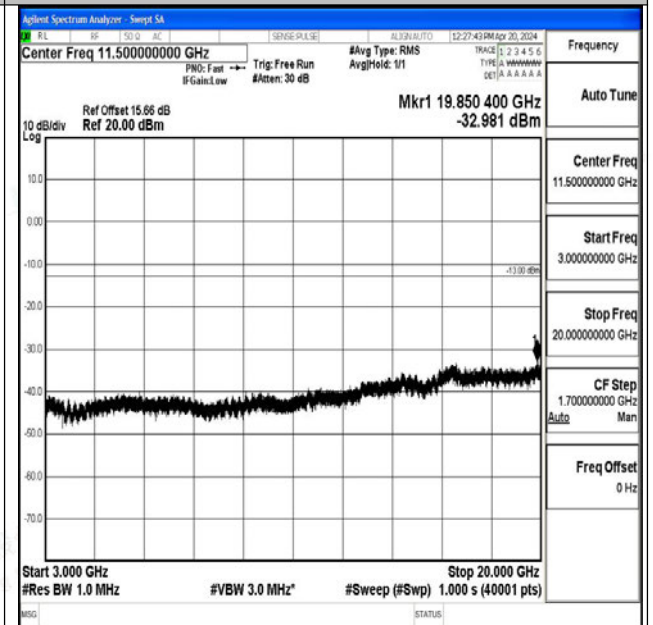
Band25_10MHz_16QAM_26640_1RB#0_3000~20000_3000~20000
