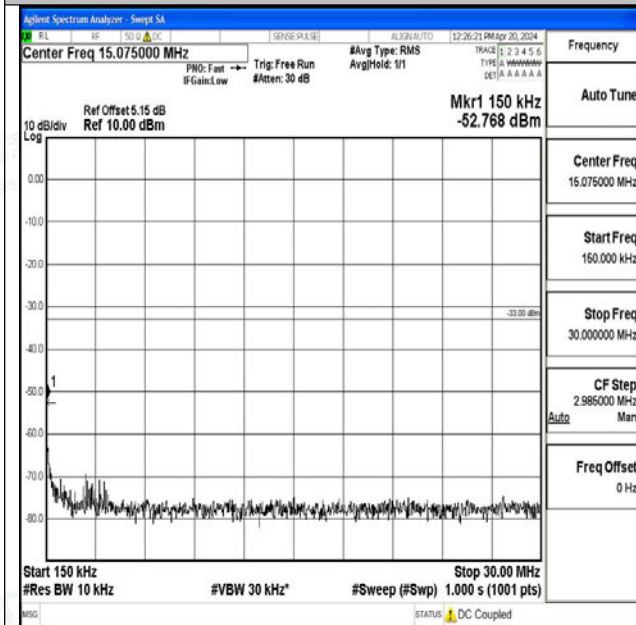
Band25_10MHz_16QAM_26365_1RB#0_0.15~30_0.15~ 30
