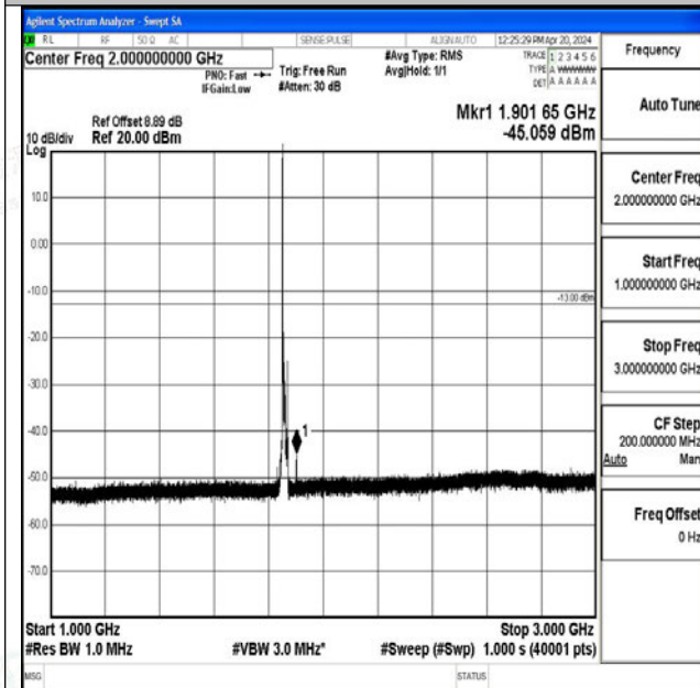
Band25_10MHz_16QAM_26090_1RB#0_1000~3000_1000~3000
