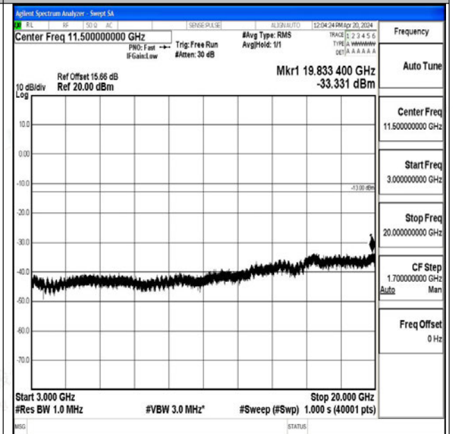
Band25_5MHz_16QAM_26365_1RB#0_3000~20000_3000~20000
