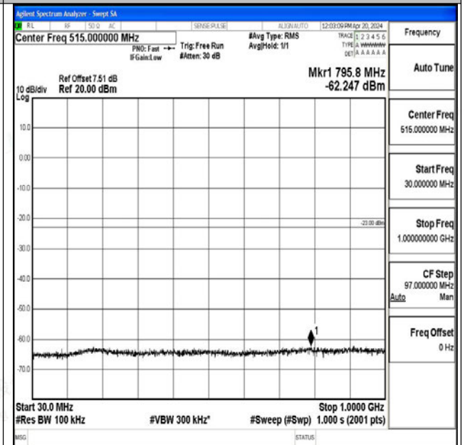
Band25_5MHz_16QAM_26065_1RB#0_30~1000_30~10 00
