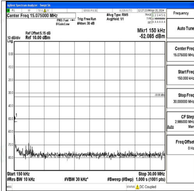
Band25_10MHz_16QAM_26640_1RB#0_0.15~30_0.15~30
