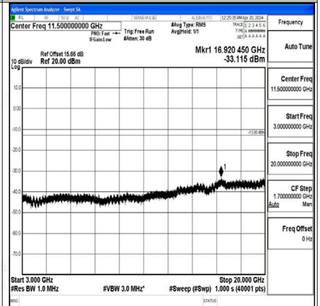
Band25_10MHz_16QAM_26090_1RB#0_3000~20000_3000~20000
