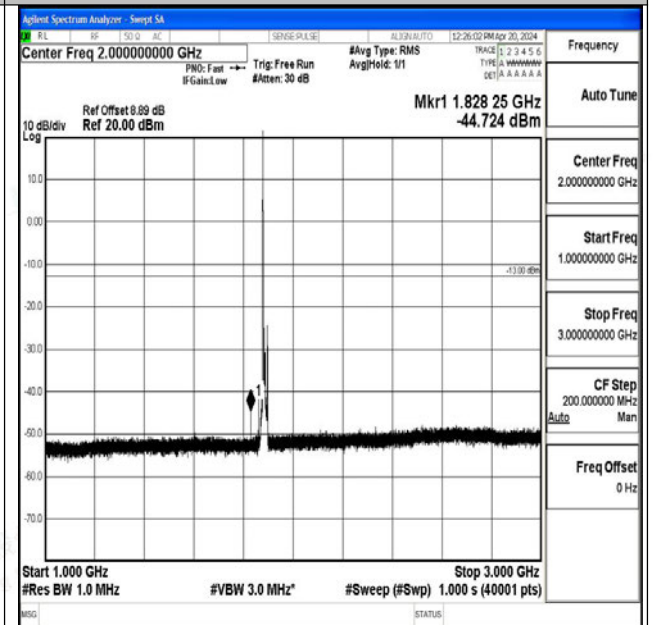
Band25_10MHz_QPSK_26365_1RB#0_1000~3000_100 0~3000
