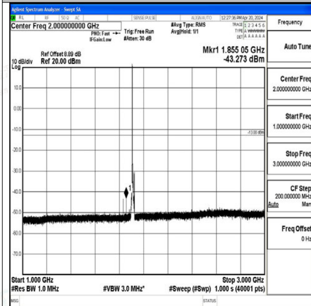
Band25_10MHz_16QAM_26640_1RB#0_1000~3000_1000~3000
