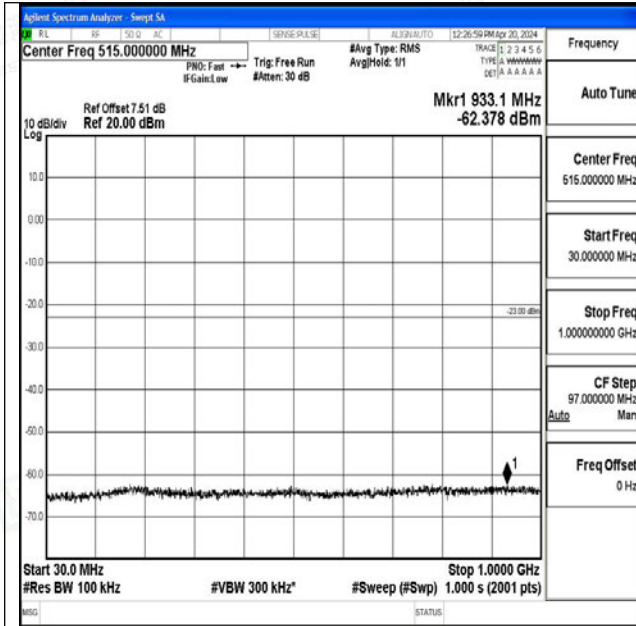
Band25_10MHz_QPSK_26640_1RB#0_30~1000_30~1000
