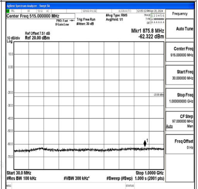
Band25_5MHz_16QAM_26665_1RB#0_30~1000_30~10 00
