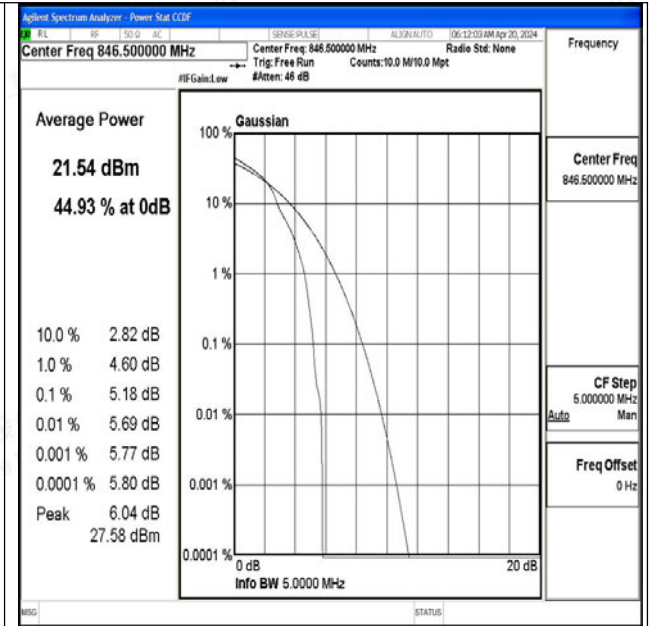
Band5-5MHz-16QAM-20625-1RB#0-PASS
