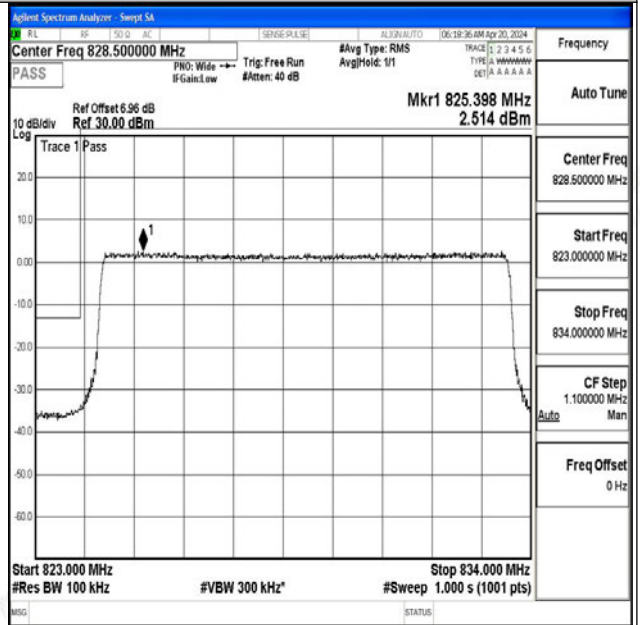
Band5_10MHz_16QAM_20450_50RB#0
