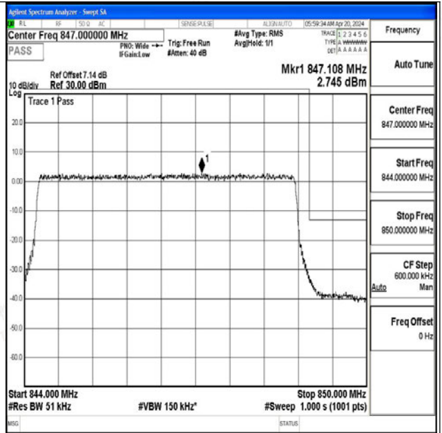
Band5_5MHz_16QAM_20625_25RB#0
