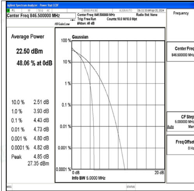
Band5-5MHz-QPSK-20625-1RB#0-PASS
