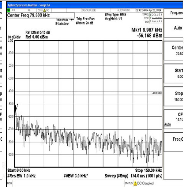
Band2_15MHz_16QAM_18900_1RB#0_0.009~0.15_0.009~0.15
