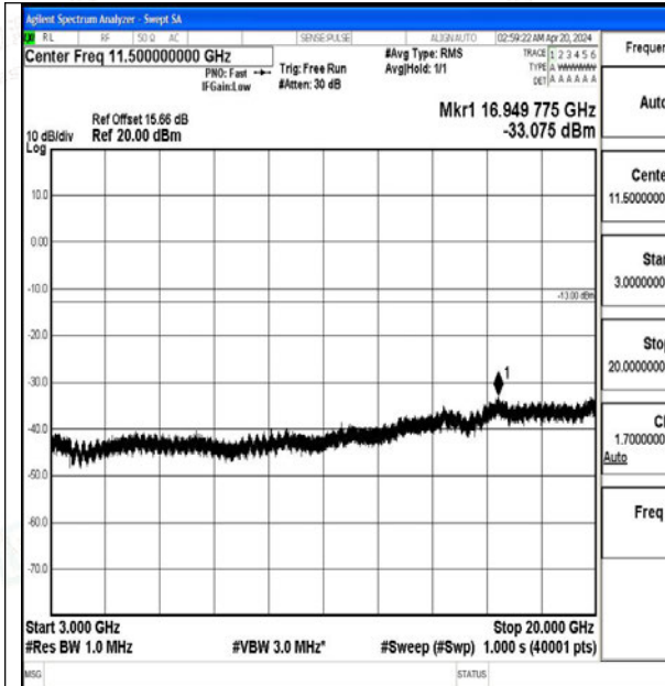
Band2_20MHz_QPSK_18900_1RB#0_3000~20000_3000~20000
