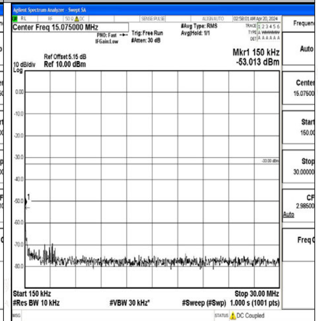
Band2_20MHz_QPSK_18700_1RB#0_0.15~30.0_0.15~30
