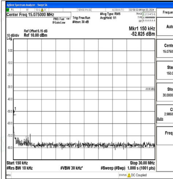
Band2_20MHz_16QAM_18700_1RB#0_0.15~30_0.1 5~30
