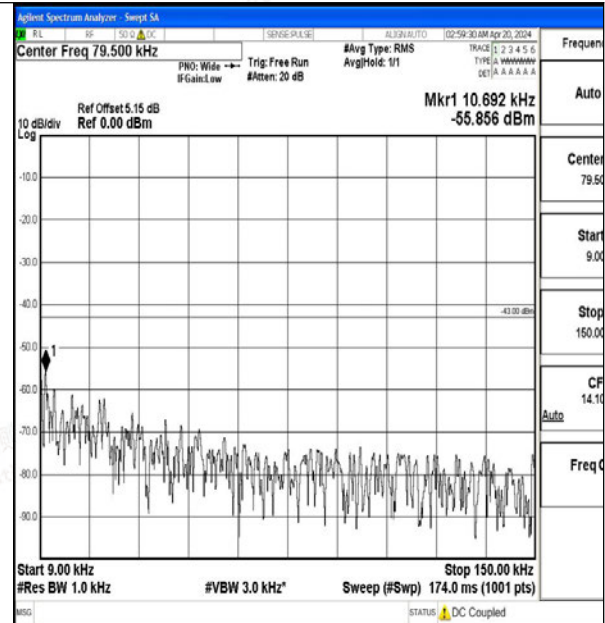
Band2_20MHz_16QAM_18900_1RB#0_0.009~0.15_0.009~0.15
