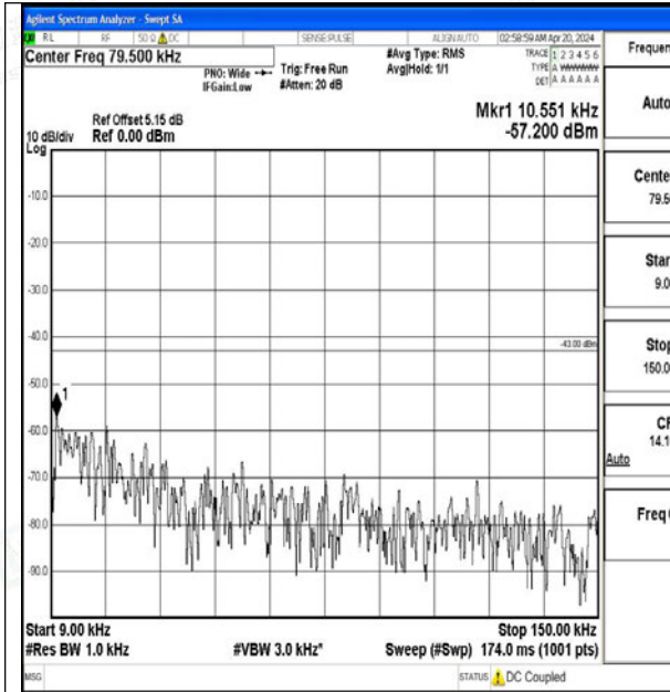
Band2_20MHz_QPSK_18900_1RB#0_0.009~0.15_0.009~0.15
