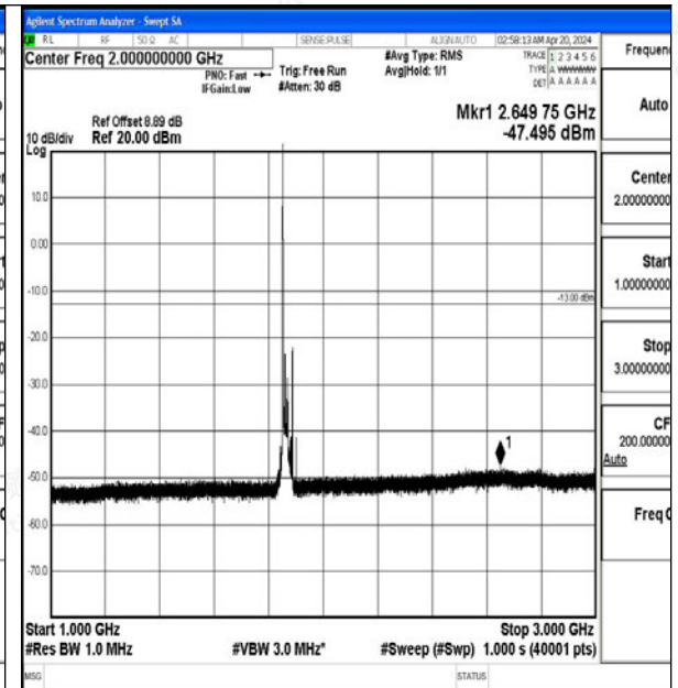
Band2_20MHz_QPSK_18700_1RB#0_1000~3000_1000~3000
