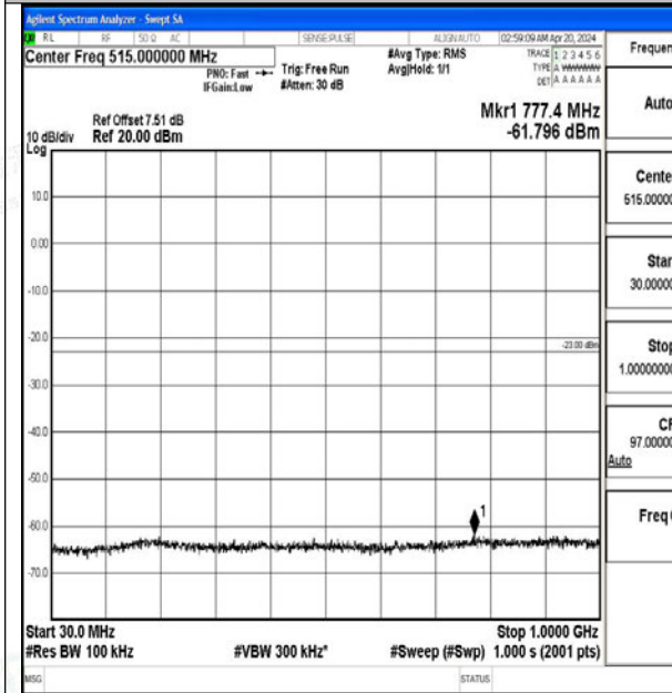
Band2_20MHz_QPSK_18900_1RB#0_30~1000_30~1000
