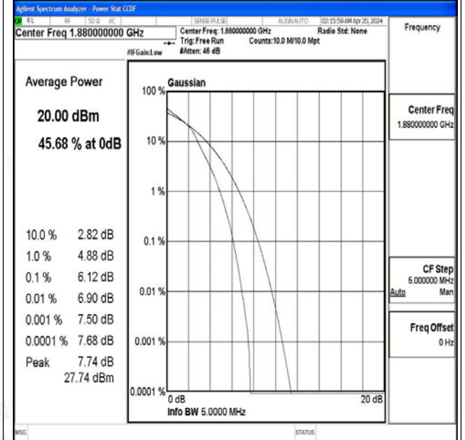
Band2-5MHz-16QAM-18900-25RB#0-PASS
