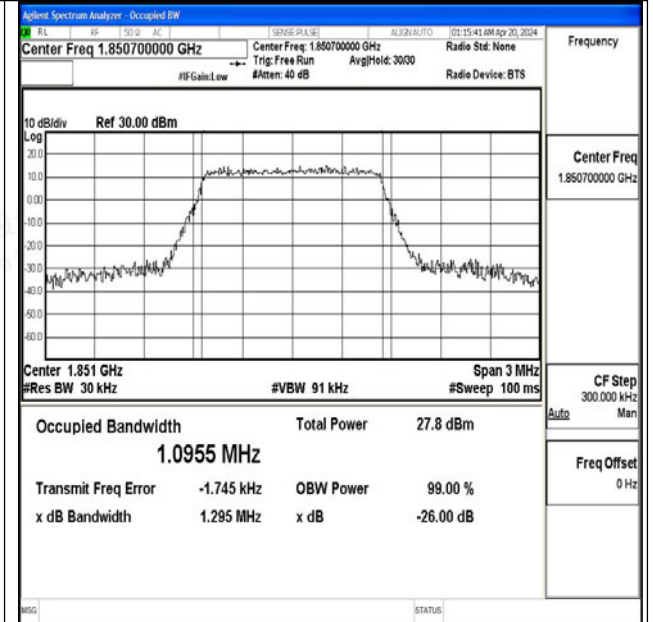
Band2-1.4MHz-16QAM-18607-6RB#0-PASS
