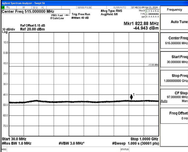
30 MHz – 1000 MHz
