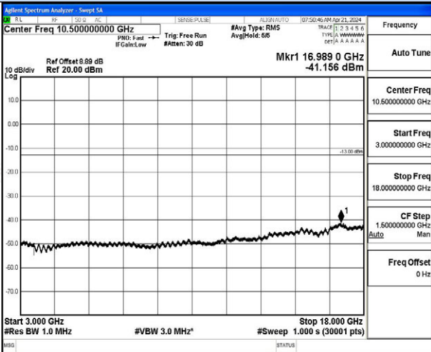
3 GHz – 18 GHz
