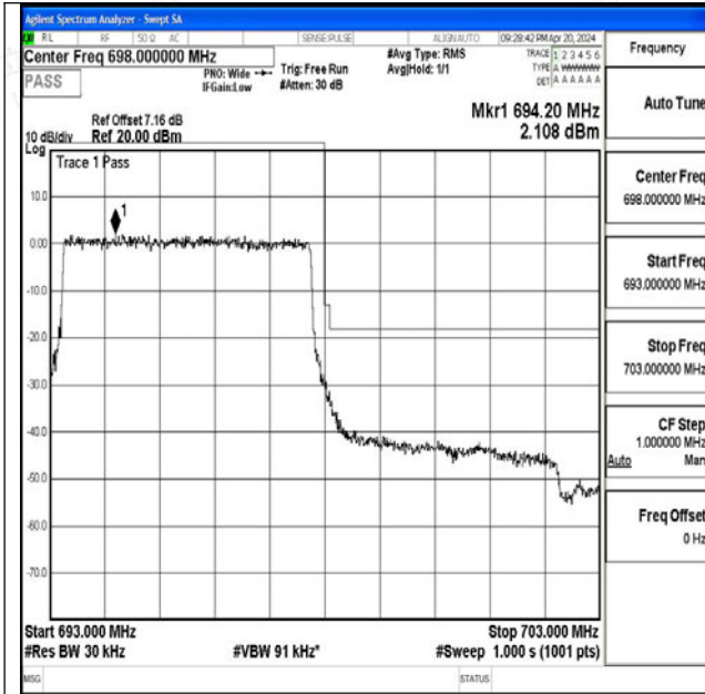
Band71_5MHz_QPSK_133447_25RB#0
