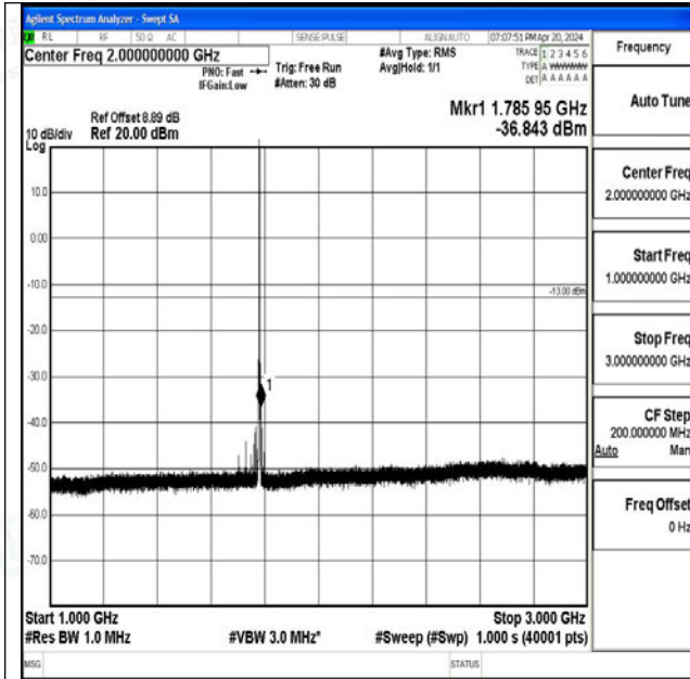
Band66_1.4MHz_16QAM_132665_1RB#0_1000~3000_1000~3000
