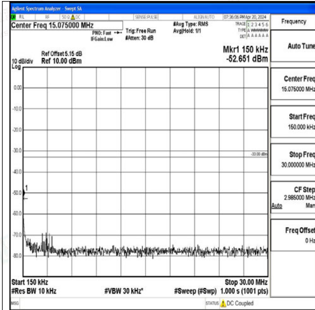
Band66_3MHz_16QAM_131987_1RB#0_0.15~30_0.15~30
