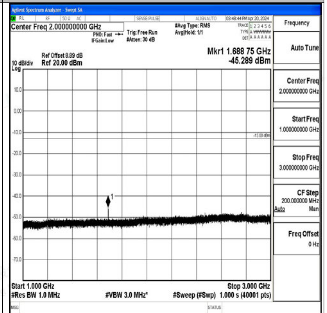
Band26_5MHz_QPSK_27015_1RB#0_1000~3000_1000~3000
