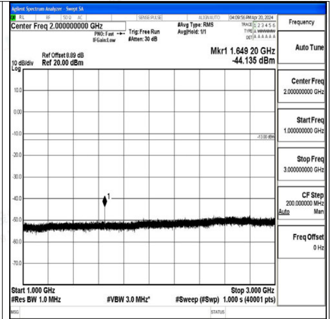
Band26_10MHz_QPSK_26840_1RB#0_1000~3000_1000~3000
