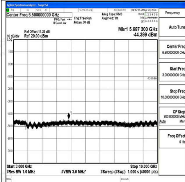
Band26_10MHz_QPSK_26990_1RB#0_3000~10000_3000~10000
