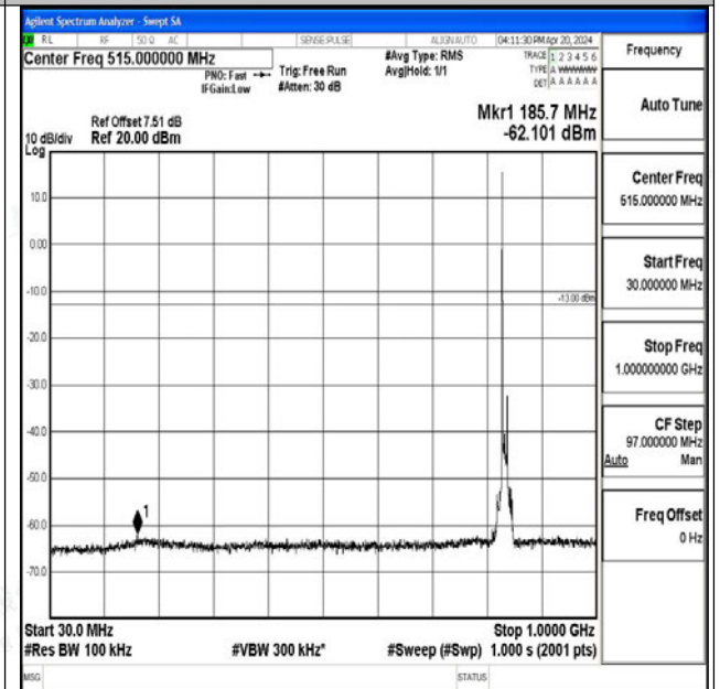
Band26_10MHz_16QAM_26915_1RB#0_30~1000_30~1000 000
