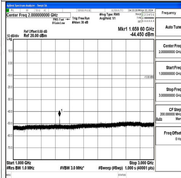
Band26_15MHz_16QAM_26915_1RB#0_1000~3000_1000~3000
