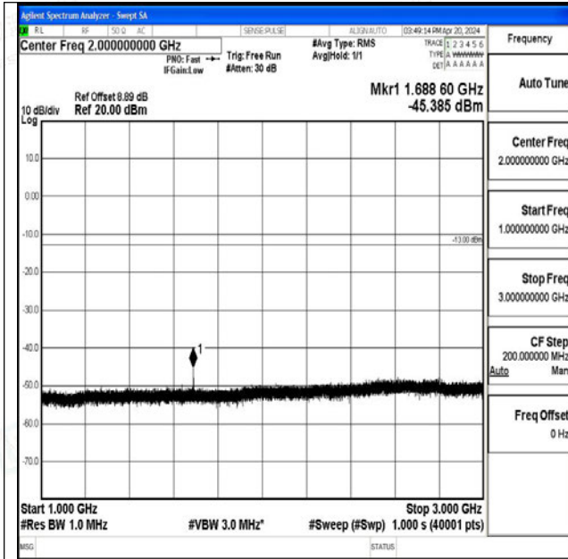
Band26_5MHz_16QAM_27015_1RB#0_1000~3000_100 0~3000
