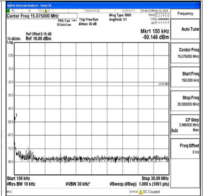
Band26_5MHz_QPSK_27015_1RB#0_0.15~30_0.15~30
