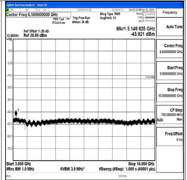
Band26_15MHz_16QAM_26865_1RB#0_3000~10000_3000~10000
