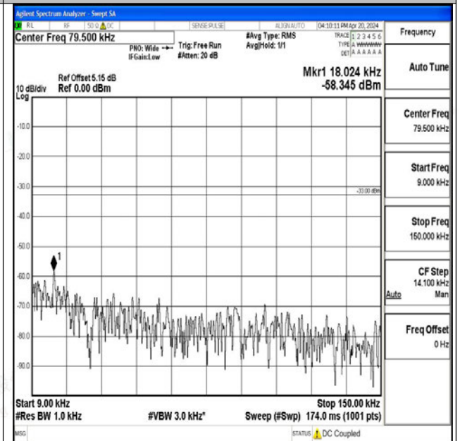
Band26_10MHz_16QAM_26840_1RB#0_0.009~0.15_0.009~0.15
