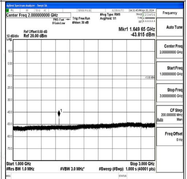
Band26_15MHz_QPSK_26865_1RB#0_1000~3000_100 0~3000
