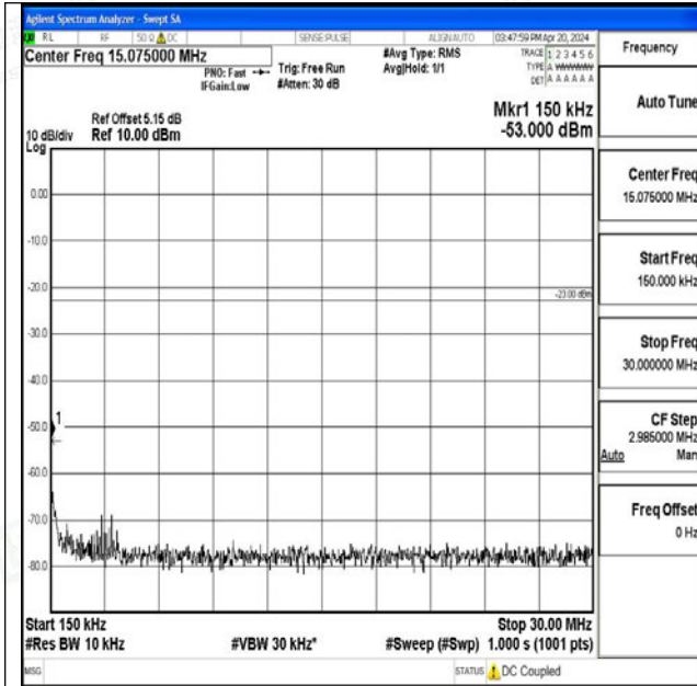
Band26_5MHz_16QAM_26915_1RB#0_0.15~30_0.15~3
