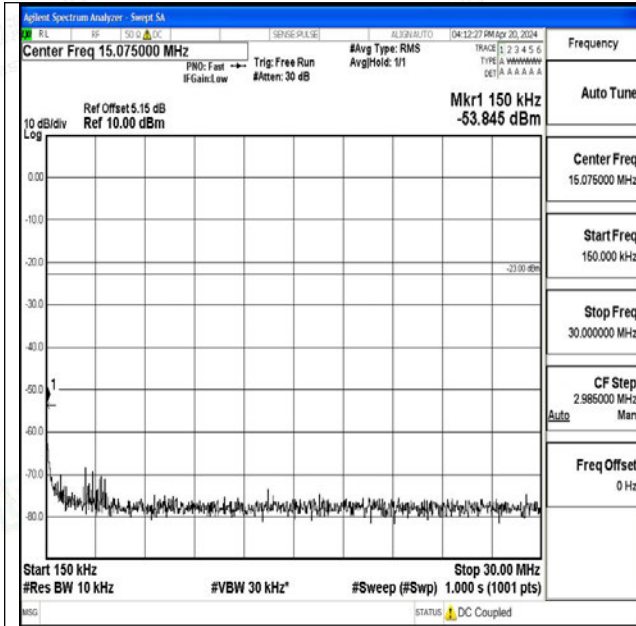
Band26_10MHz_16QAM_26990_1RB#0_0.15~30_0.15~30
