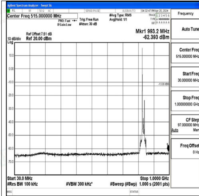
Band26_15MHz_QPSK_26915_1RB#0_30~1000_30~1000
