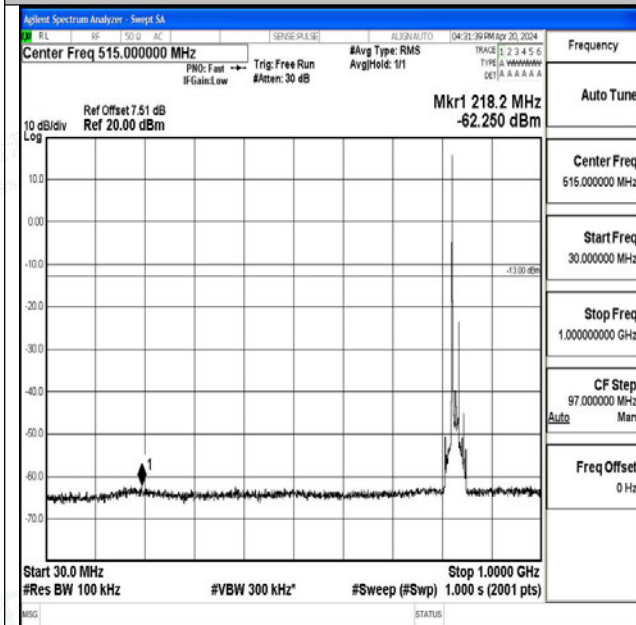
Band26_15MHz_QPSK_26865_1RB#0_30~1000_30~10 00
