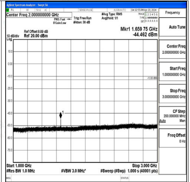
Band26_15MHz_QPSK_26915_1RB#0_1000~3000_1000~3000
