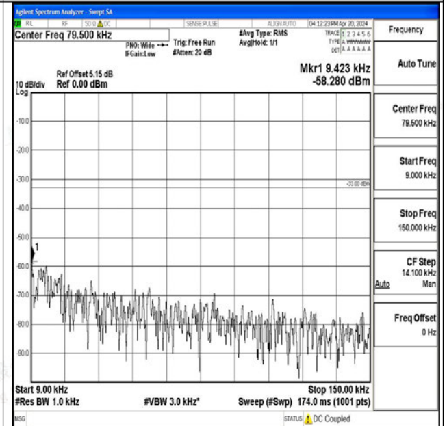
Band26_10MHz_16QAM_26990_1RB#0_0.009~0.15_0.009~0.15
