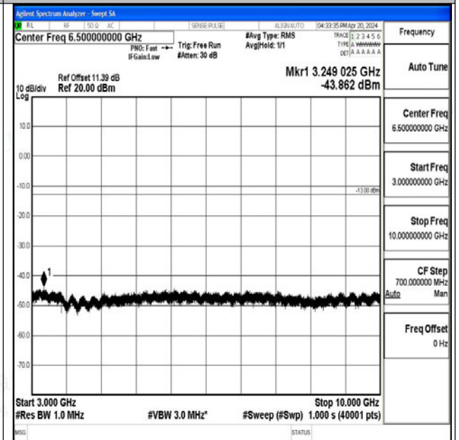
Band26_15MHz_16QAM_26915_1RB#0_3000~10000_3000~10000
