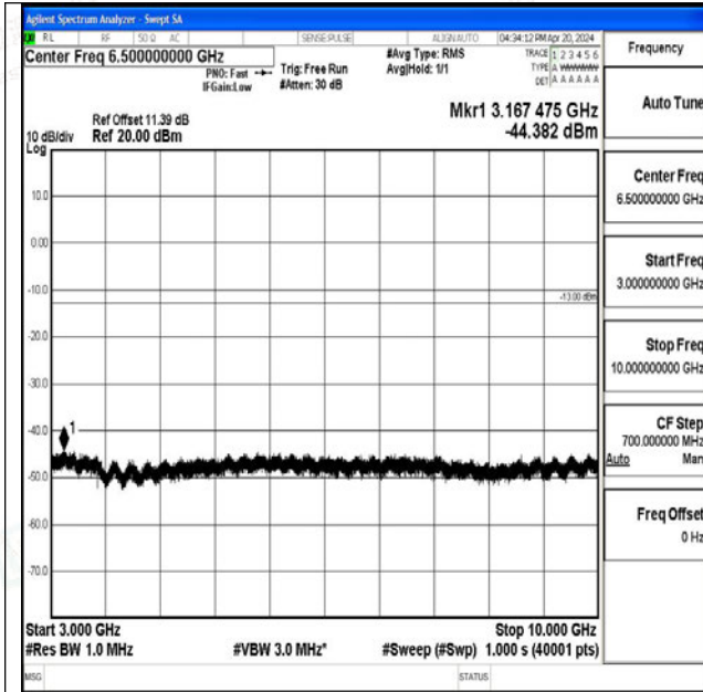
Band26_15MHz_QPSK_26965_1RB#0_3000~10000_30 00~10000
