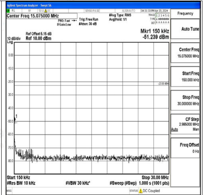
Band26_15MHz_QPSK_26865_1RB#0_0.15~30_0.15~3 0
