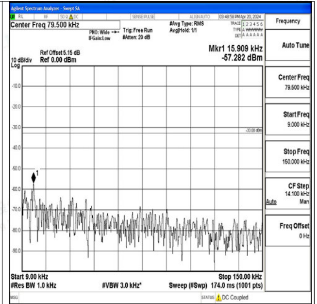
Band26_5MHz_16QAM_27015_1RB#0_0.009~0.15_0.0 09~0.15
