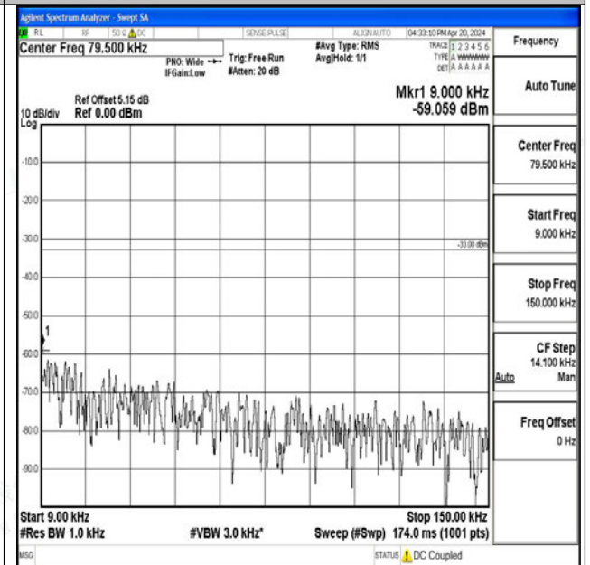
Band26_15MHz_16QAM_26915_1RB#0_0.009~0.15_0.009~0.15
