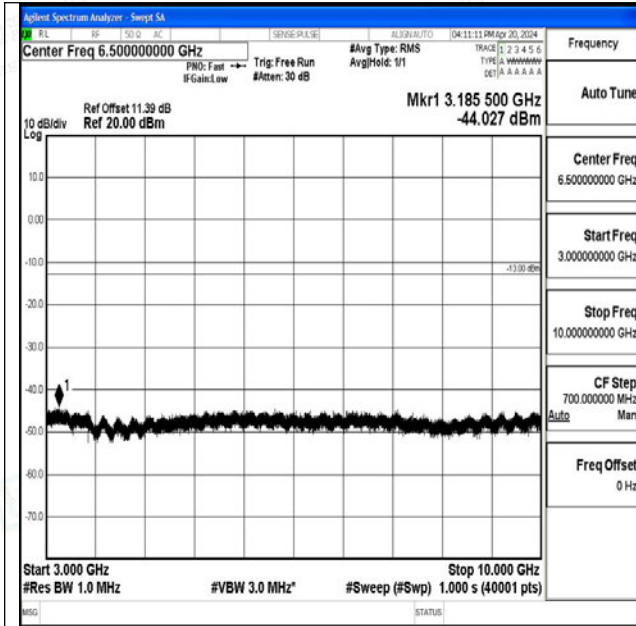
Band26_10MHz_QPSK_26915_1RB#0_3000~10000_30 00~10000
