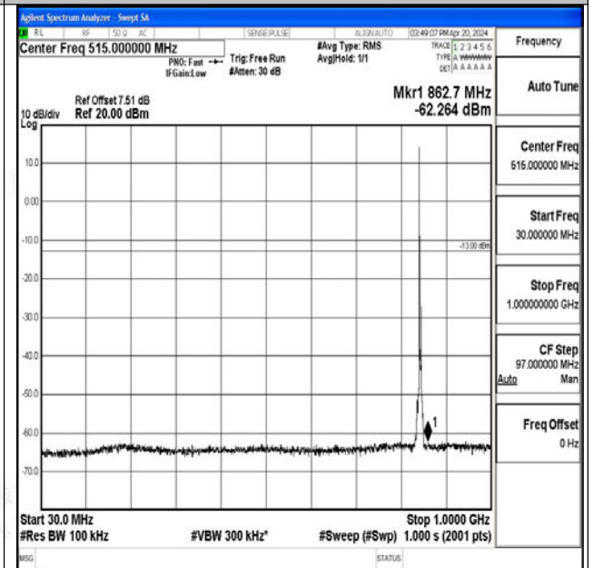
Band26_5MHz_16QAM_27015_1RB#0_30~1000_30~10 00
