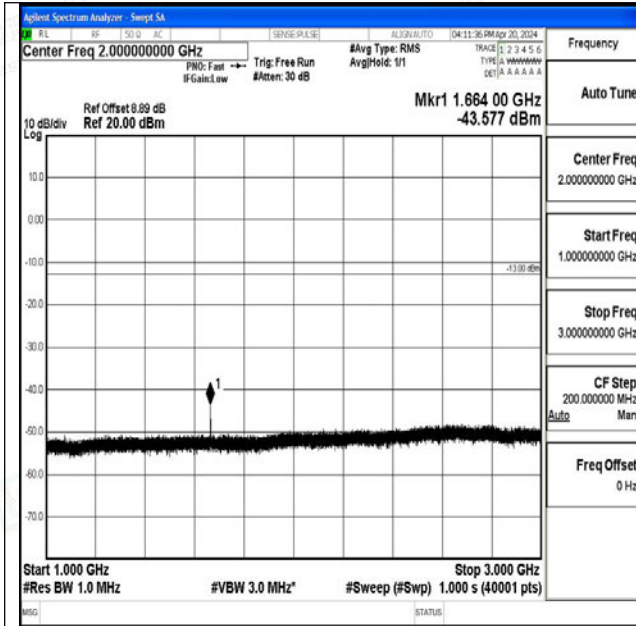
Band26_10MHz_16QAM_26915_1RB#0_1000~3000_1000~3000
