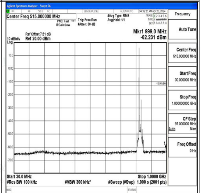
Band26_15MHz_16QAM_26865_1RB#0_30~1000_30~1000
