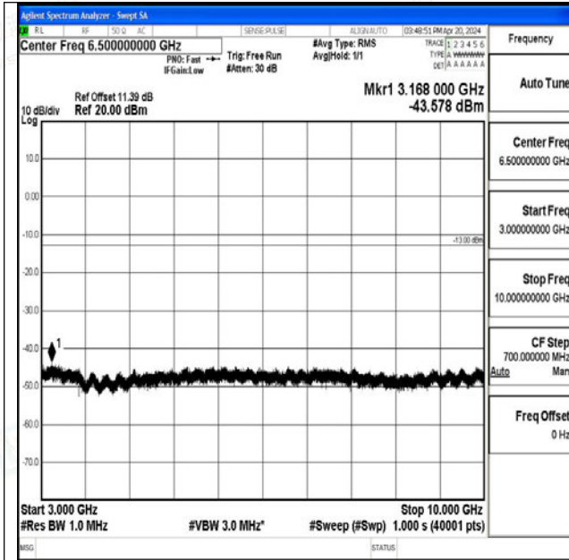
Band26_5MHz_QPSK_27015_1RB#0_3000~10000_300 0~10000
