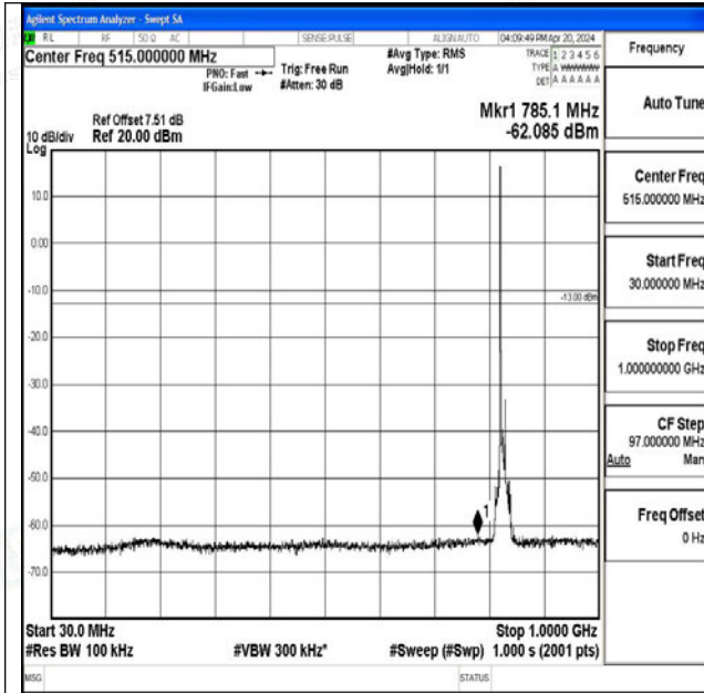
Band26_10MHz_QPSK_26840_1RB#0_30~1000_30~1000
