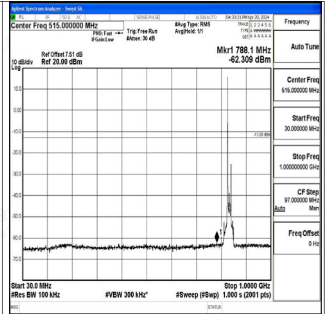
Band26_15MHz_16QAM_26915_1RB#0_30~1000_30~1000
