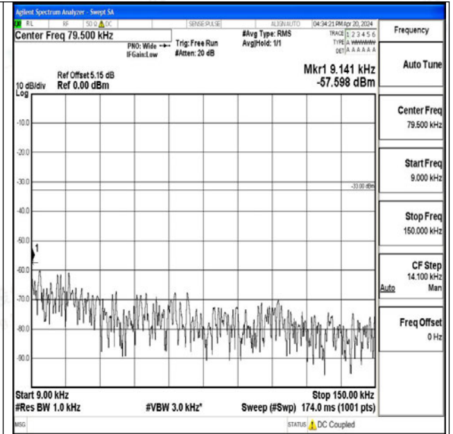
Band26_15MHz_16QAM_26965_1RB#0_0.009~0.15_0. 009~0.15
