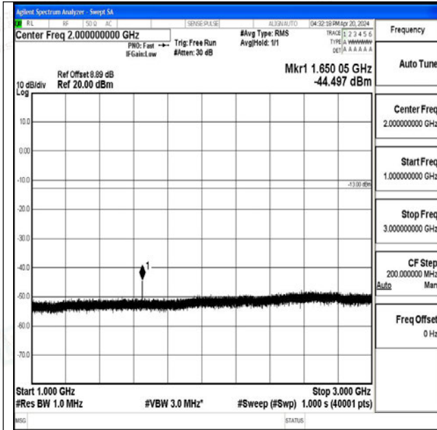
Band26_15MHz_16QAM_26865_1RB#0_1000~3000_1000~3000
