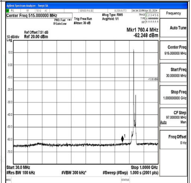
Band26_15MHz_16QAM_26965_1RB#0_30~1000_30~1000 000
