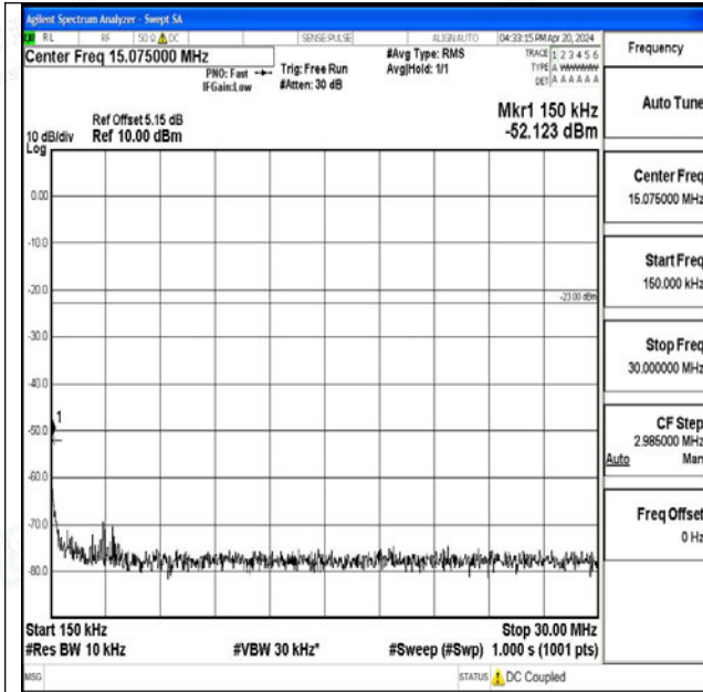
Band26_15MHz_16QAM_26915_1RB#0_0.15~30_0.15~30
