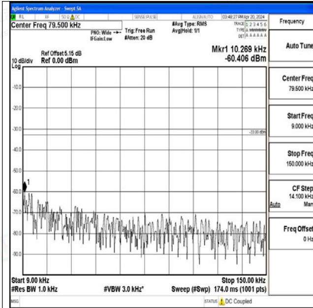
Band26_5MHz_QPSK_27015_1RB#0_0.009~0.15_0.009~0.15
