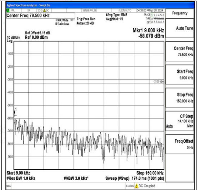
Band26_15MHz_16QAM_26865_1RB#0_0.009~0.15_0.009~0.15
