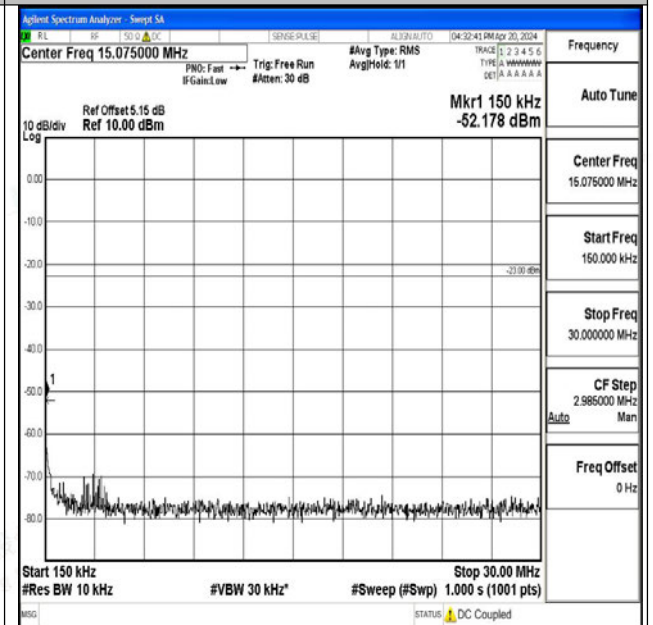
Band26_15MHz_QPSK_26915_1RB#0_0.15~30_0.15~30
