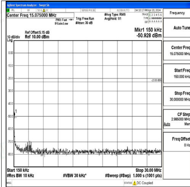
Band26_10MHz_16QAM_26840_1RB#0_0.15~30_0.15~30
