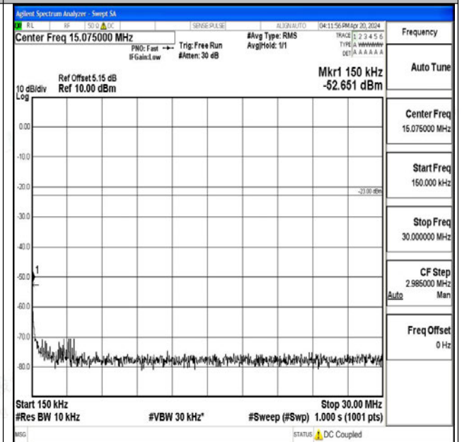
Band26_10MHz_QPSK_26990_1RB#0_0.15~30_0.15~30
