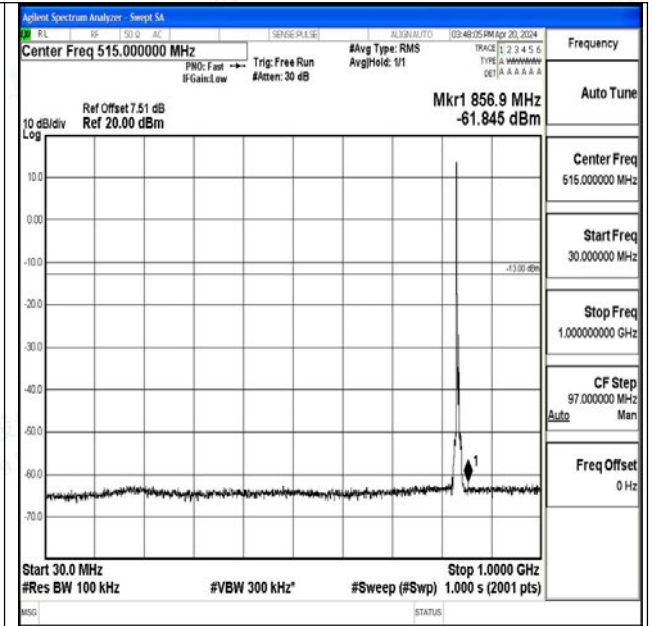
Band26_5MHz_16QAM_26915_1RB#0_30~1000_30~10
