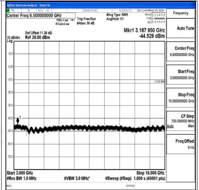
Band26_10MHz_16QAM_26915_1RB#0_3000~10000_3000~10000
