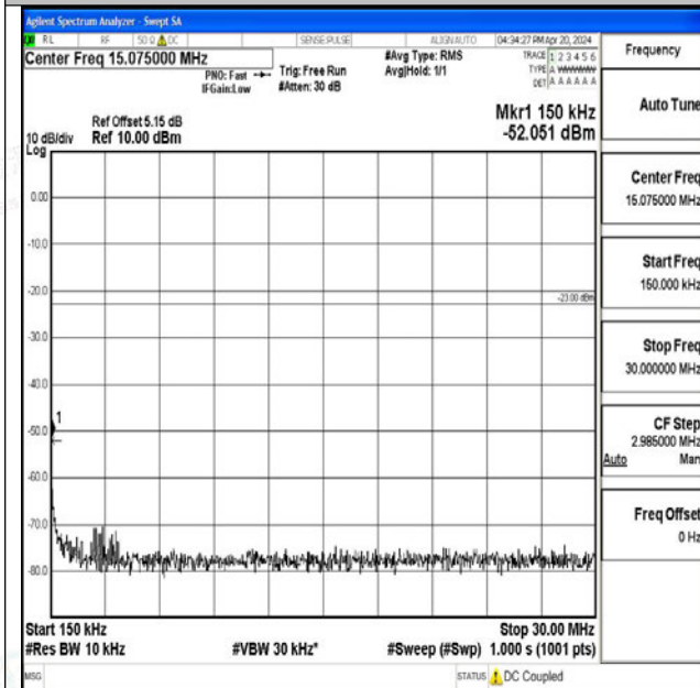
Band26_15MHz_16QAM_26965_1RB#0_0.15~30_0.15~30 30
