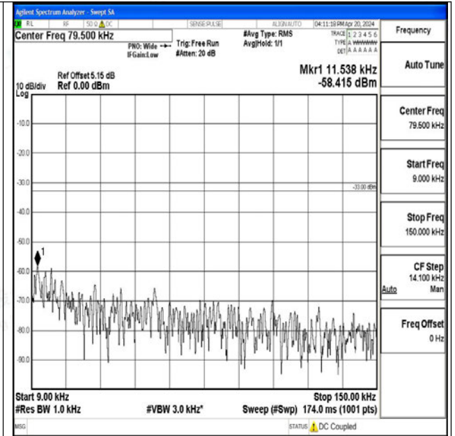
Band26_10MHz_16QAM_26915_1RB#0_0.009~0.15_0. 009~0.15
