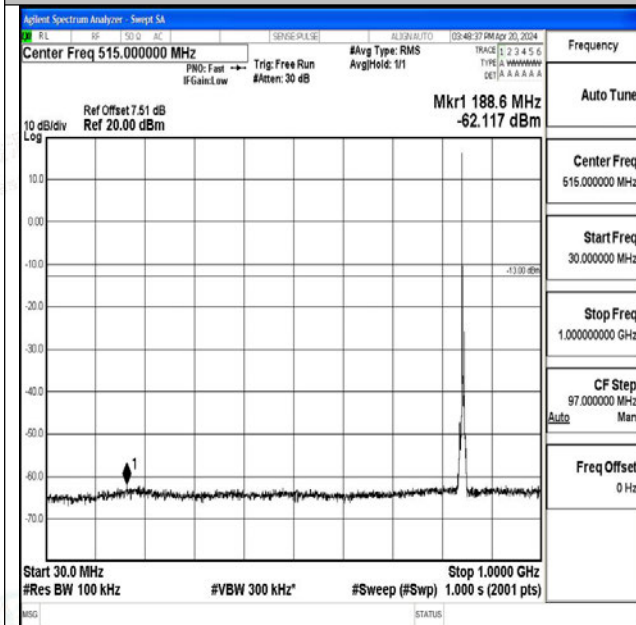
Band26_5MHz_QPSK_27015_1RB#0_30~1000_30~1000
