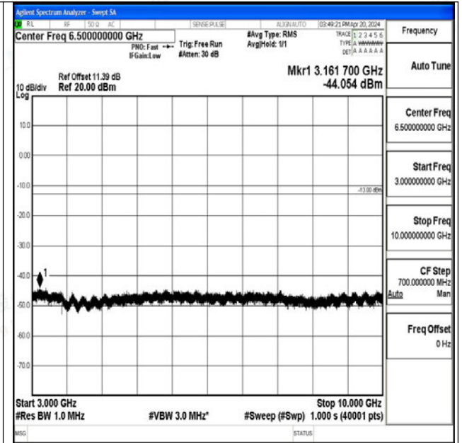
Band26_5MHz_16QAM_27015_1RB#0_3000~10000_30 00~10000
