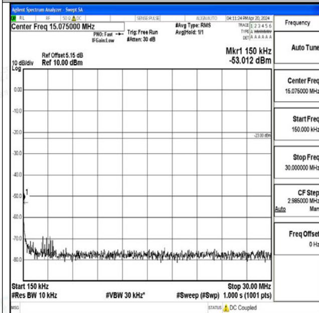
Band26_10MHz_16QAM_26915_1RB#0_0.15~30_0.15~30 30
