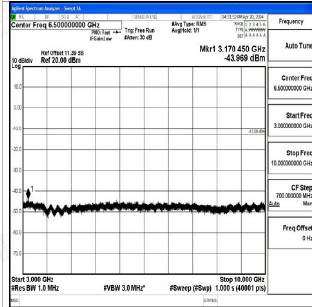
Band26_15MHz_QPSK_26865_1RB#0_3000~10000_3000~10000
