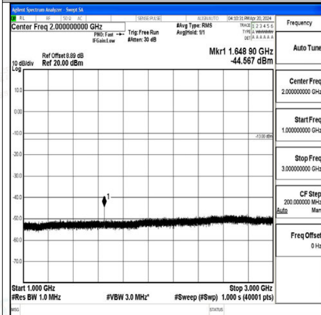
Band26_10MHz_16QAM_26840_1RB#0_1000~3000_1000~3000
