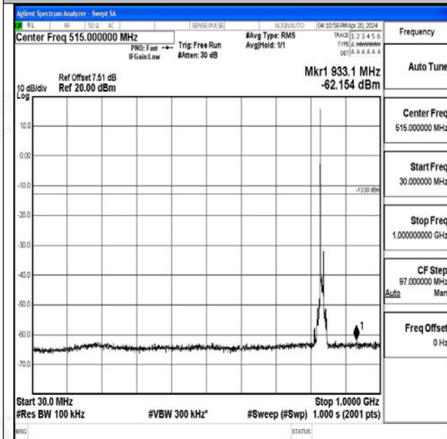
Band26_10MHz_QPSK_26915_1RB#0_30~1000_30~10 00
