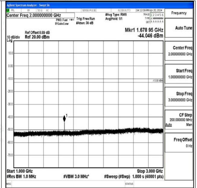
Band26_10MHz_QPSK_26990_1RB#0_1000~3000_1000~3000
