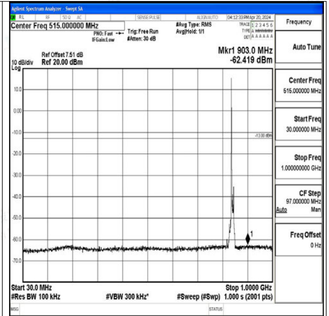
Band26_10MHz_16QAM_26990_1RB#0_30~1000_30~1000
