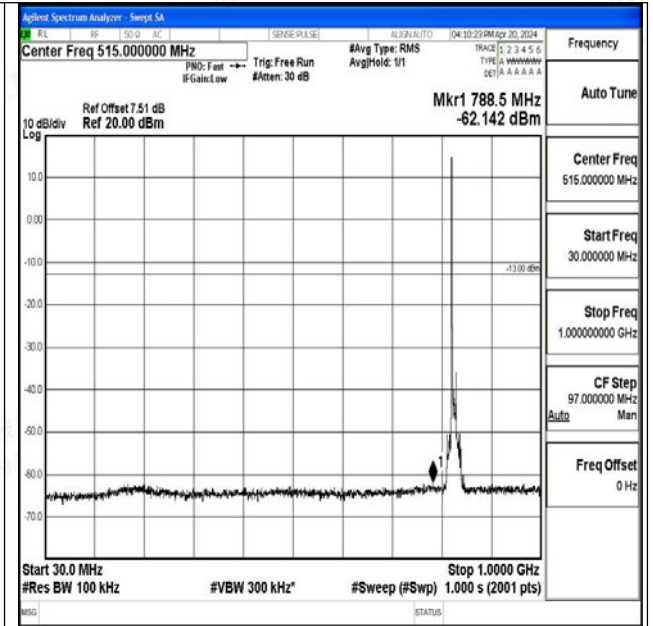
Band26_10MHz_16QAM_26840_1RB#0_30~1000_30~1000
