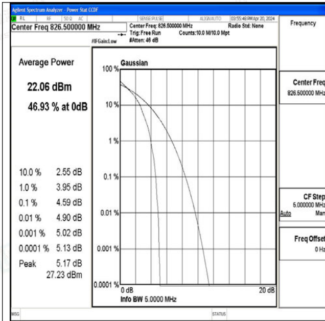
26(824-849)-5MHz-QPSK-26815-1RB#0-PASS
