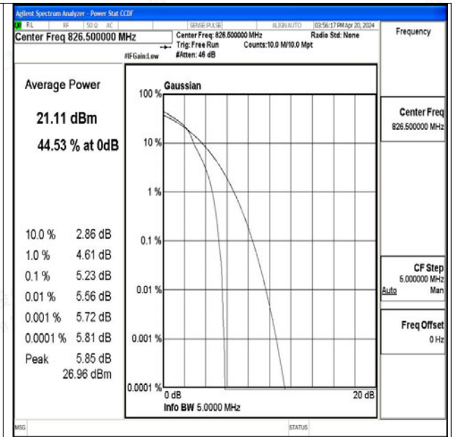
26(824-849)-5MHz-16QAM-26815-1RB#0-PASS
