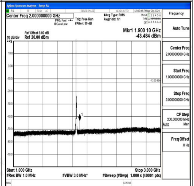
Band25_5MHz_QPSK_26065_1RB#0_1000~3000_1000~3000
