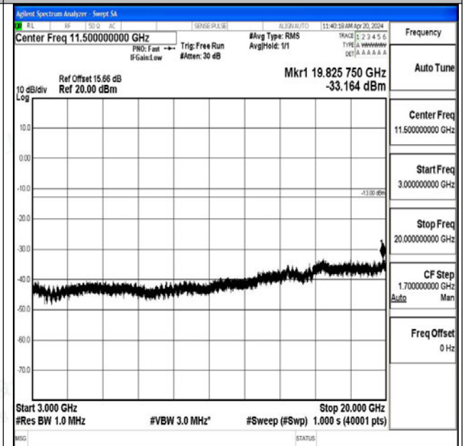
Band25_3MHz_16QAM_26055_1RB#0_3000~20000_3000~20000
