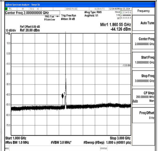
Band25_5MHz_QPSK_26665_1RB#0_1000~3000_1000~3000
