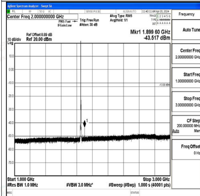
Band25_3MHz_16QAM_26055_1RB#0_1000~3000_1000~3000
