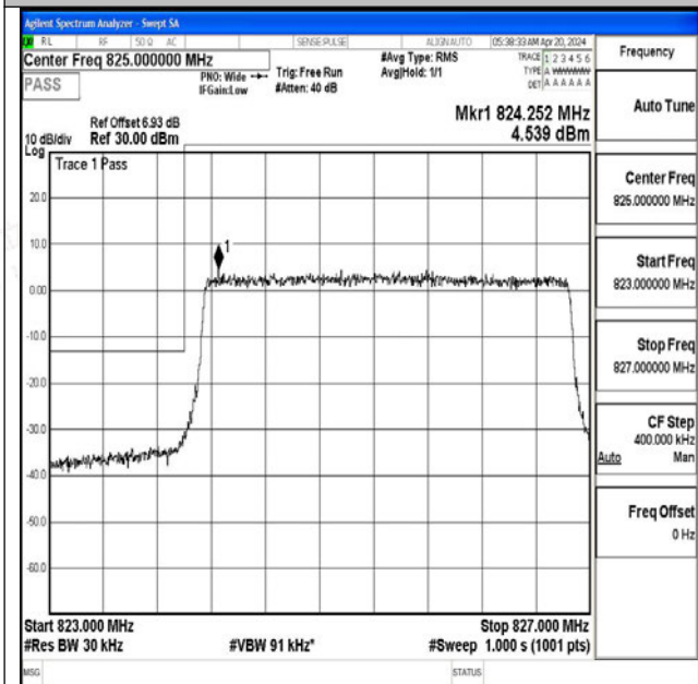
Band5_3MHz_QPSK_20415_15RB#0
