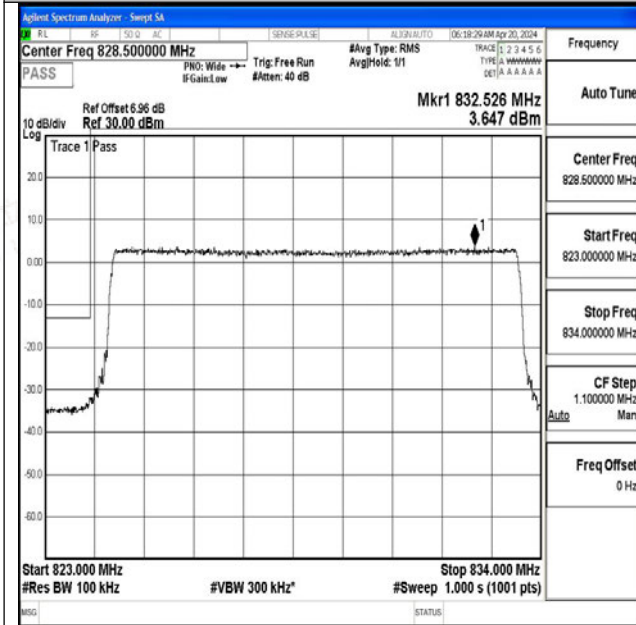
Band5_10MHz_QPSK_20450_50RB#0
