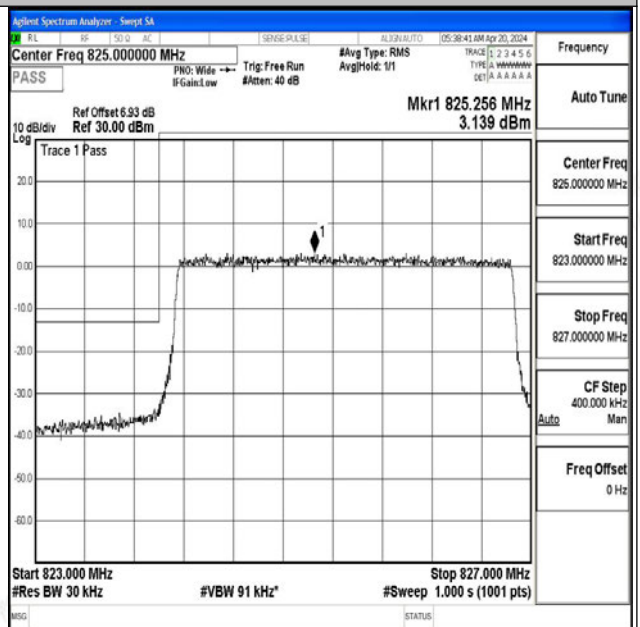
Band5_3MHz_16QAM_20415_15RB#0
