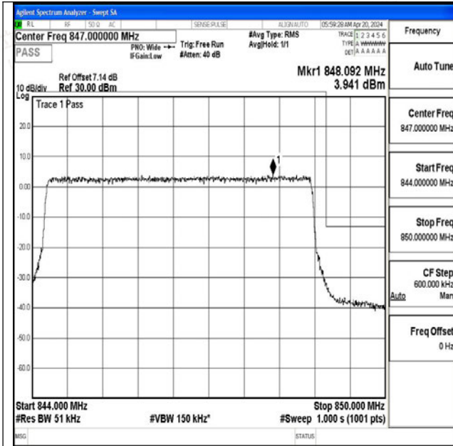
Band5_5MHz_QPSK_20625_25RB#0
