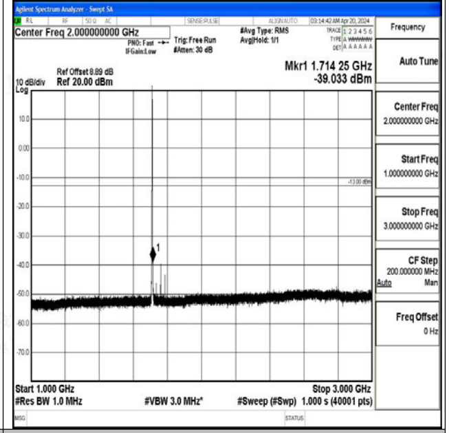
Band4_1.4MHz_QPSK_19957_1RB#0_1000~3000_1000 ~3000
