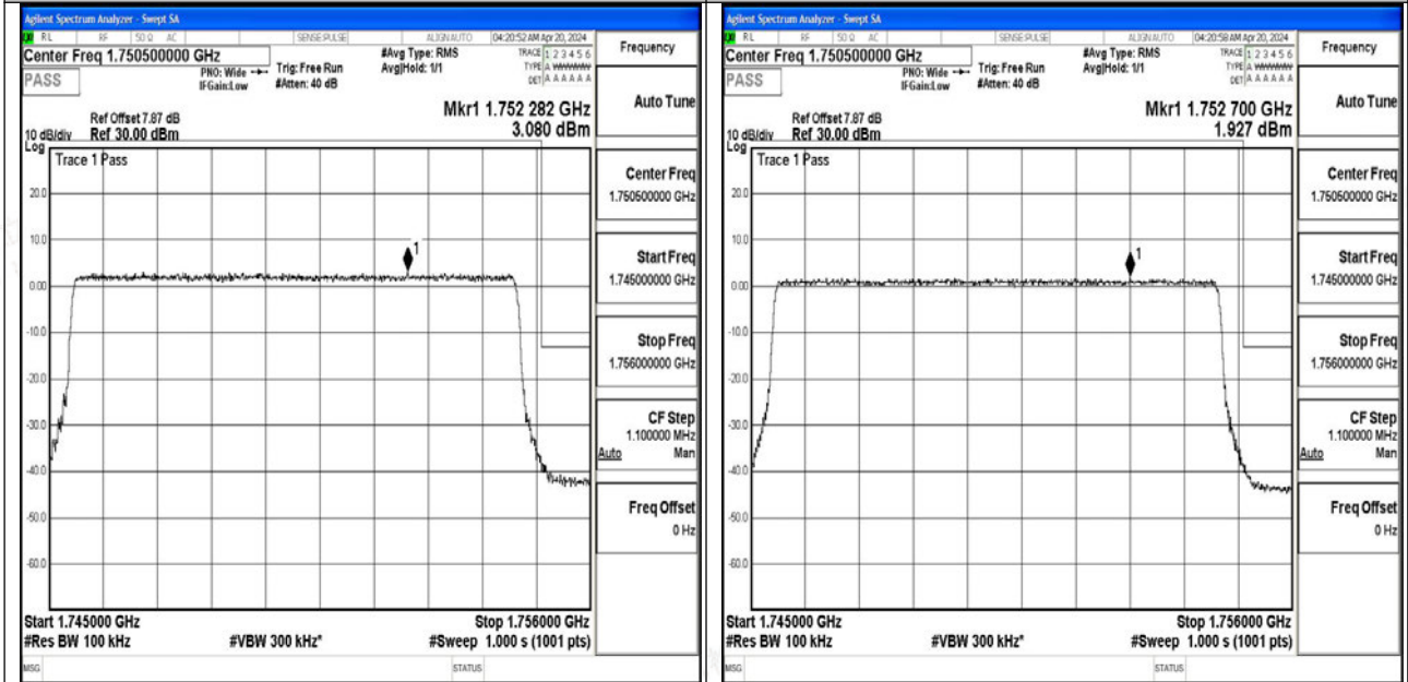
Band4_10MHz_QPSK_20350_50RB#0
