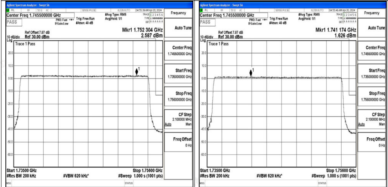
Band4_20MHz_QPSK_20300_100RB#0
