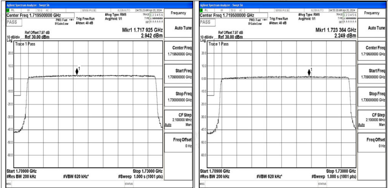
Band4_20MHz_QPSK_20050_100RB#0
