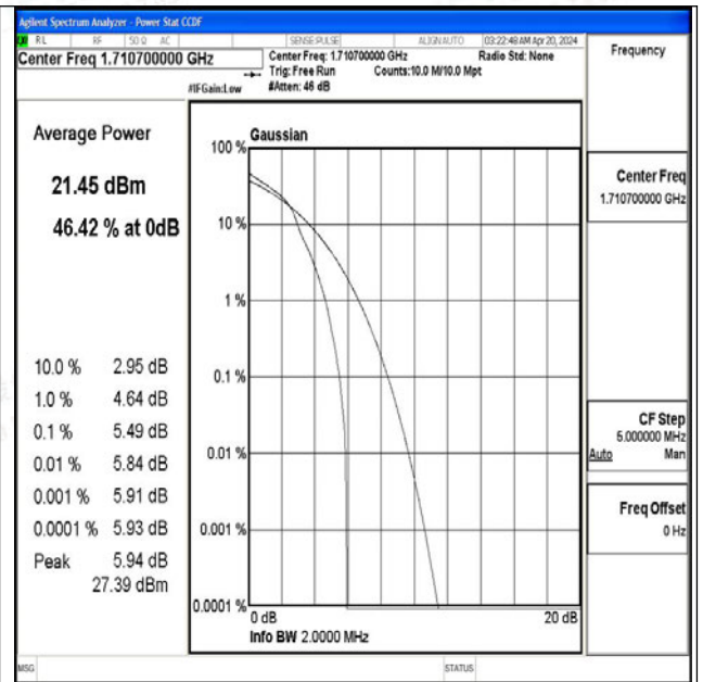
Band4-1.4MHz-16QAM-19957-1RB#0-PASS
