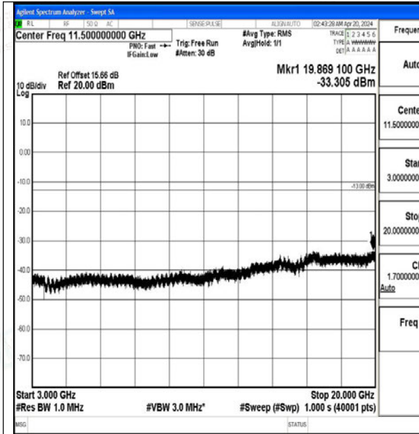
Band2_15MHz_QPSK_19125_1RB#0_3000~20000_3000~20000
