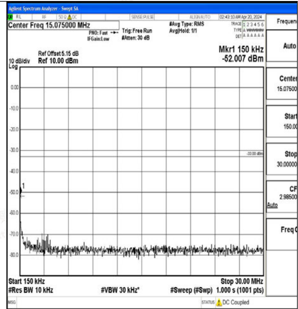
Band2_15MHz_QPSK_19125_1RB#0_0.15~30_0.15~30
