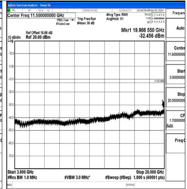
Band2_15MHz_16QAM_19125_1RB#0_3000~20000_3000~20000
