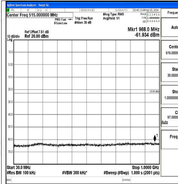
Band2_15MHz_QPSK_18900_1RB#0_30~1000_30~1000
