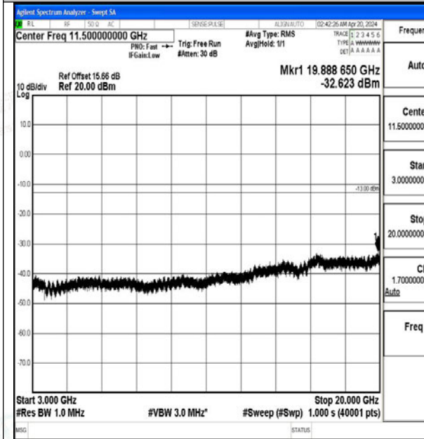
Band2_15MHz_QPSK_18900_1RB#0_3000~20000_3000~20000
