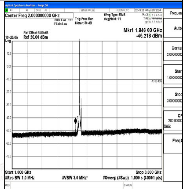
Band2_15MHz_QPSK_19125_1RB#0_1000~3000_1000~3000
