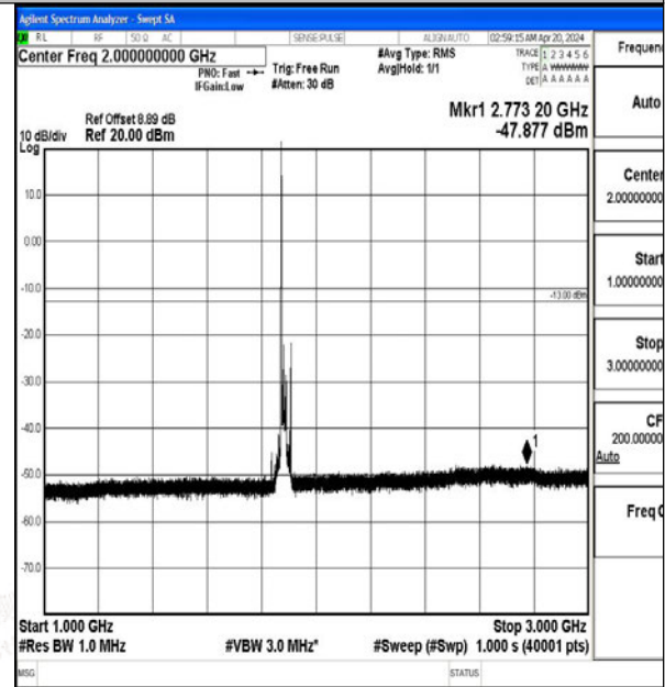
Band2_20MHz_QPSK_18900_1RB#0_1000~3000_1000~3000
