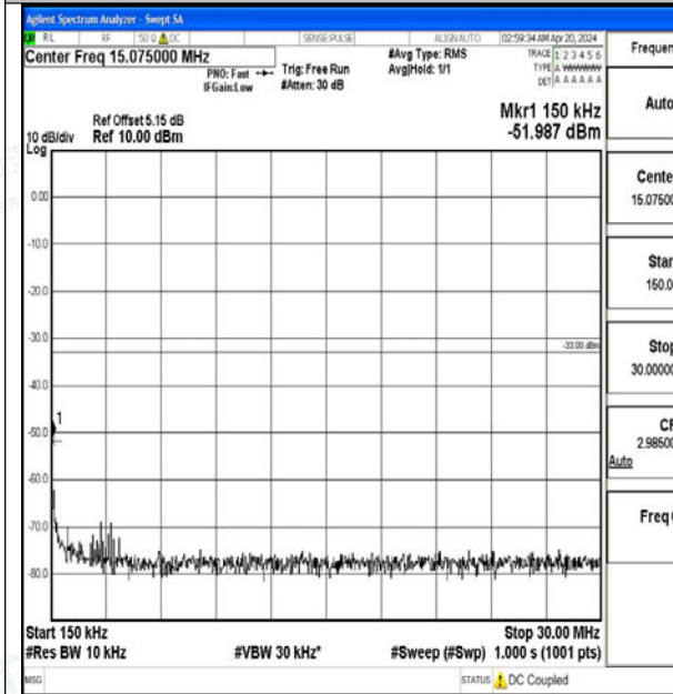
Band2_20MHz_16QAM_18900_1RB#0_0.15~30_0.15~30
