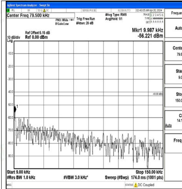
Band2_15MHz_QPSK_19125_1RB#0_0.009~0.15_0.009~0.15
