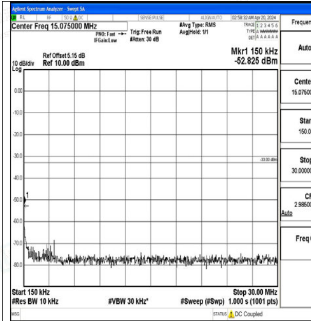
Band2_20MHz_16QAM_18700_1RB#0_0.15~30_0.1 5~30
