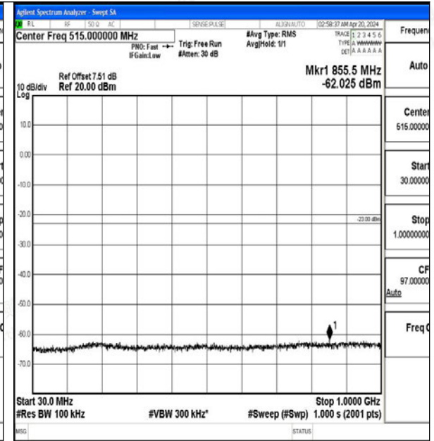
Band2_20MHz_16QAM_18700_1RB#0_30~1000_30 ~1000
