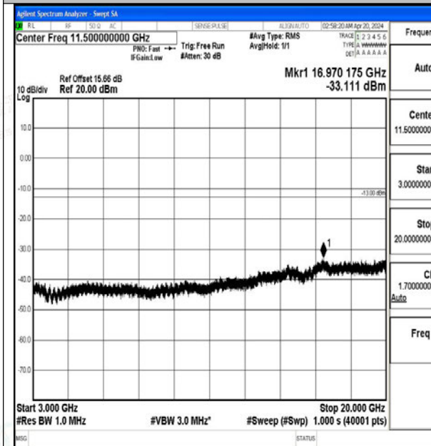
Band2_20MHz_QPSK_18700_1RB#0_3000~20000_3000~20000
