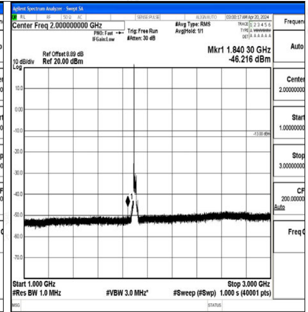
Band2_20MHz_QPSK_19100_1RB#0_1000~3000_1000~3000
