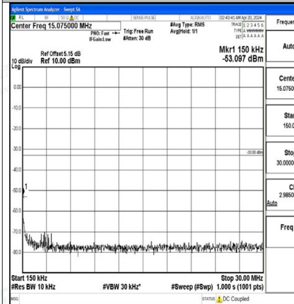
Band2_15MHz_16QAM_19125_1RB#0_0.15~30_0.1_5~30
