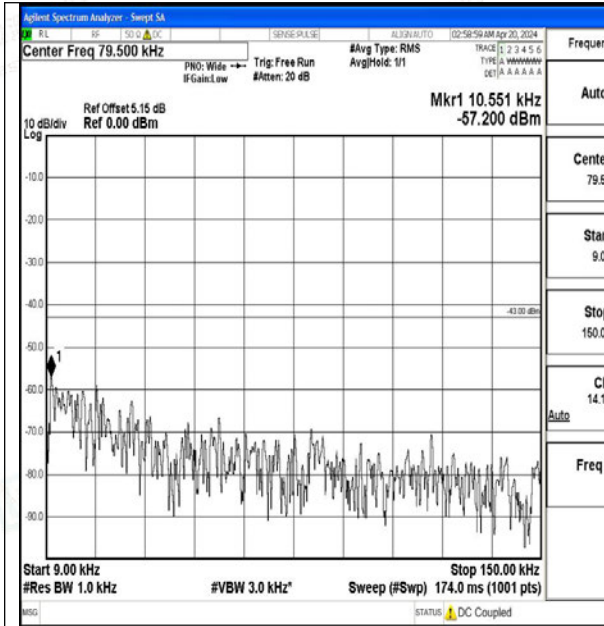
Band2_20MHz_QPSK_18900_1RB#0_0.009~0.15_0.009~0.15
