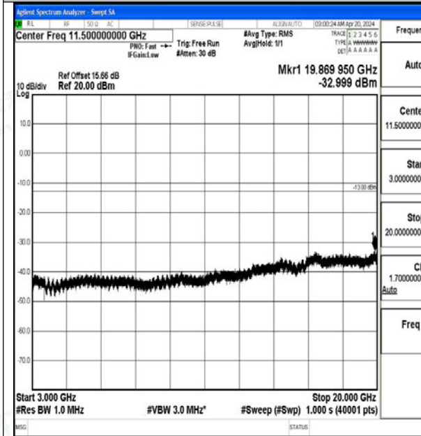
Band2_20MHz_QPSK_19100_1RB#0_3000~20000_3000~20000
