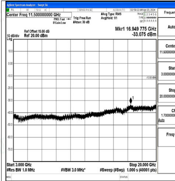
Band2_20MHz_QPSK_18900_1RB#0_3000~20000_3000~20000
