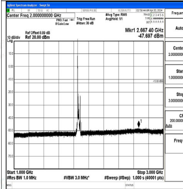
Band2_20MHz_16QAM_18700_1RB#0_1000~3000_ 1000~3000
