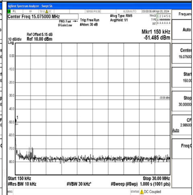
Band2_20MHz_QPSK_19100_1RB#0_0.15~30_0.15~30
