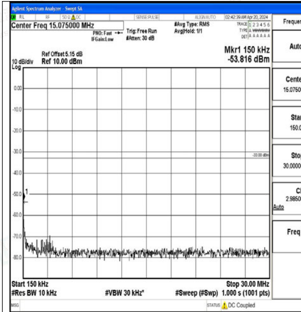
Band2_15MHz_16QAM_18900_1RB#0_0.15~30_0.1 5~30
