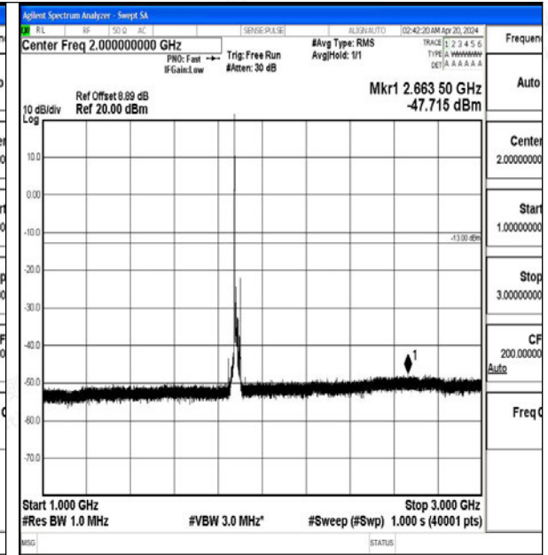
Band2_15MHz_QPSK_18900_1RB#0_1000~3000_1000~3000
