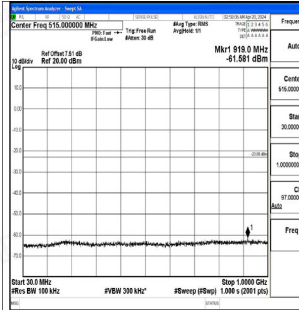
Band2_20MHz_QPSK_18700_1RB#0_30~1000_30~1000
