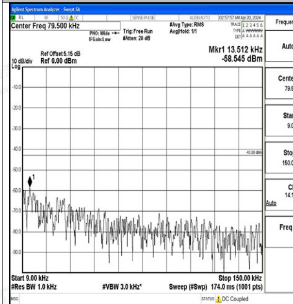
Band2_20MHz_QPSK_18700_1RB#0_0.009~0.15_0.009~0.15
