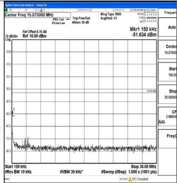
Band2_20MHz_QPSK_18900_1RB#0_0.15~30_0.15~30
