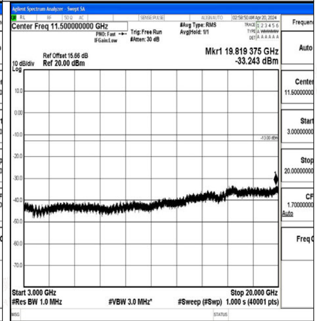
Band2_20MHz_16QAM_18700_1RB#0_3000~20000 _3000~20000
