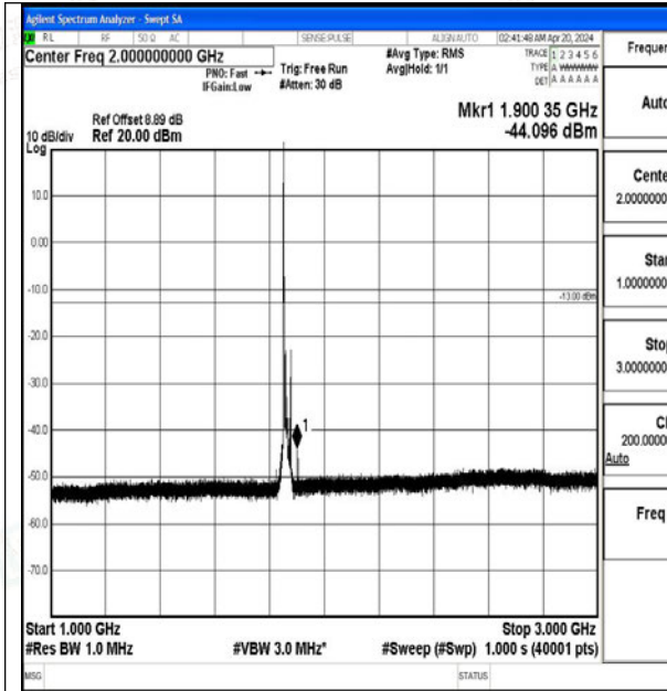
Band2_15MHz_16QAM_18675_1RB#0_1000~3000_1000~3000
