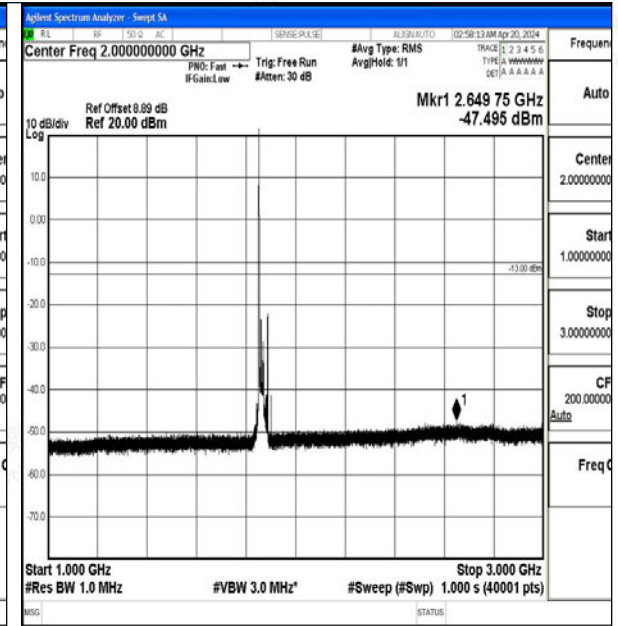
Band2_20MHz_QPSK_18700_1RB#0_1000~3000_1000~3000
