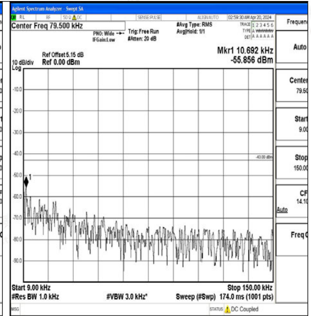
Band2_20MHz_16QAM_18900_1RB#0_0.009~0.15_0.009~0.15
