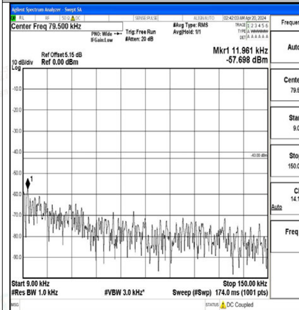
Band2_15MHz_QPSK_18900_1RB#0_0.009~0.15_0.009~0.15
