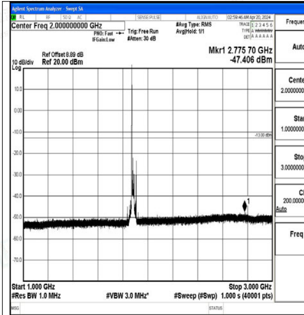
Band2_20MHz_16QAM_18900_1RB#0_1000~3000_1000~3000
