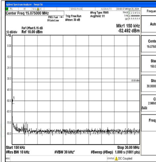
Band2_20MHz_16QAM_19100_1RB#0_0.15~30_0.1 5~30
