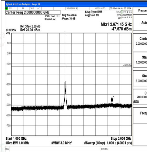
Band2_20MHz_16QAM_19100_1RB#0_1000~3000_1000~3000
