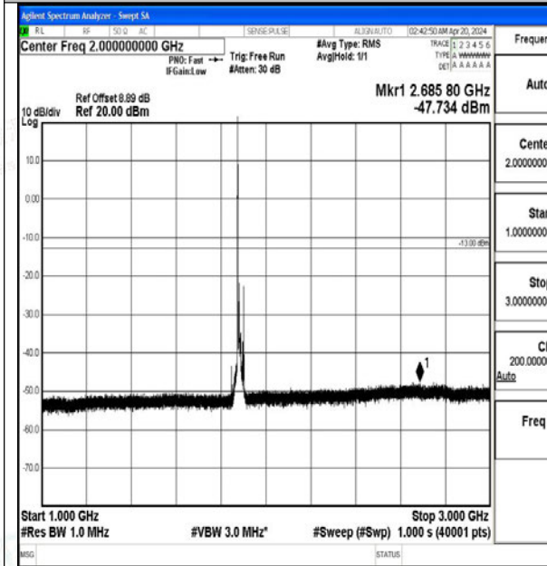
Band2_15MHz_16QAM_18900_1RB#0_1000~3000_ 1000~3000
