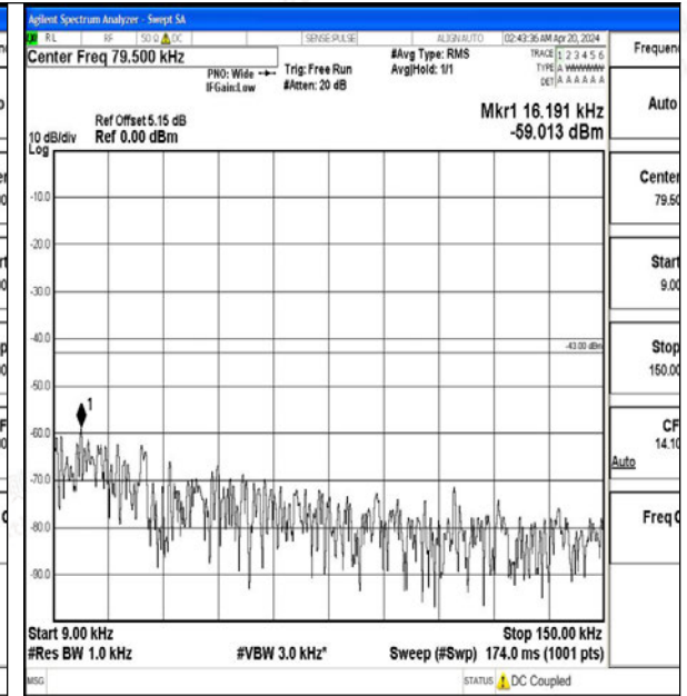
Band2_15MHz_16QAM_19125_1RB#0_0.009~0.15_0.009~0.15
