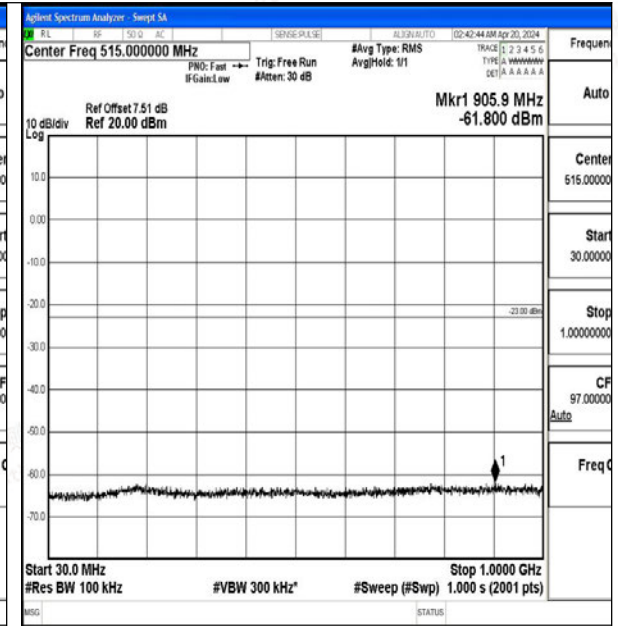
Band2_15MHz_16QAM_18900_1RB#0_30~1000_30 ~1000
