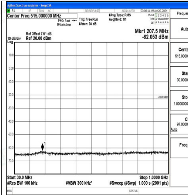
Band2_20MHz_QPSK_19100_1RB#0_30~1000_30~1000
