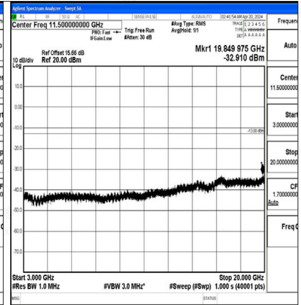
Band2_15MHz_16QAM_18675_1RB#0_3000~20000_3000~20000
