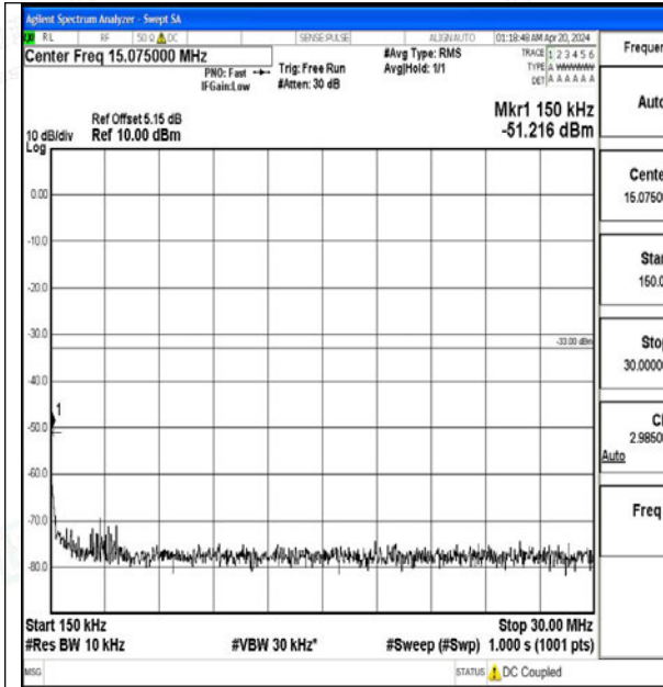
Band2_1.4MHz_16QAM_18900_1RB#0_0.15~30_0.1 5~30
