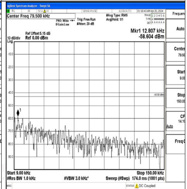
Band2_1.4MHz_16QAM_18900_1RB#0_0.009~0.15_0.009~0.15
