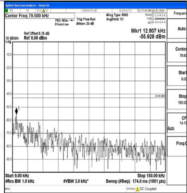
Band2_1.4MHz_16QAM_18607_1RB#0_0.009~0.15_0.009~0.15
