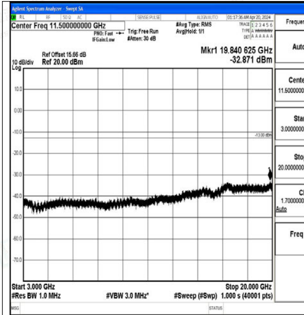
Band2_1.4MHz_QPSK_18607_1RB#0_3000~20000_3000~20000
