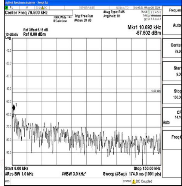
Band2_3MHz_16QAM_18615_1RB#0_0.009~0.15_0.009~0.15
