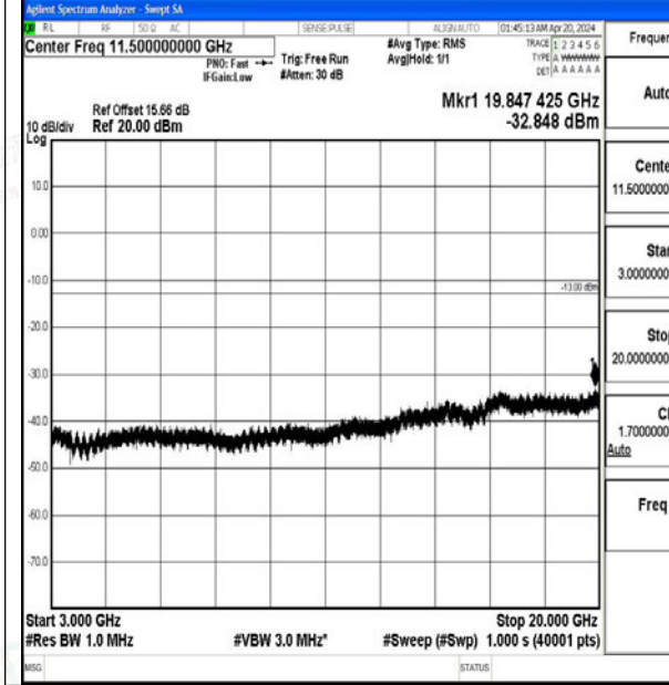
Band2_3MHz_QPSK_18615_1RB#0_3000~20000_3000~20000
