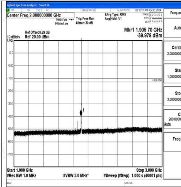
Band2_1.4MHz_16QAM_19193_1RB#0_1000~3000_1000~3000
