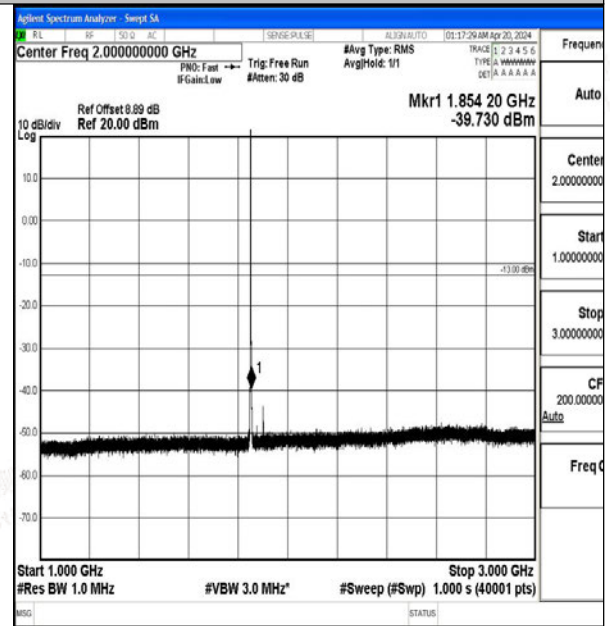
Band2_1.4MHz_QPSK_18607_1RB#0_1000~3000_1000~3000
