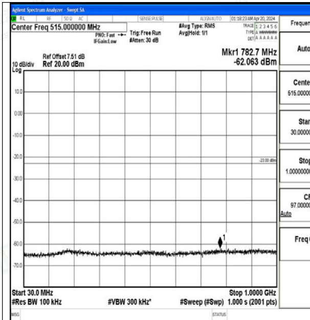
Band2_1.4MHz_QPSK_18900_1RB#0_30~1000_30~1000
