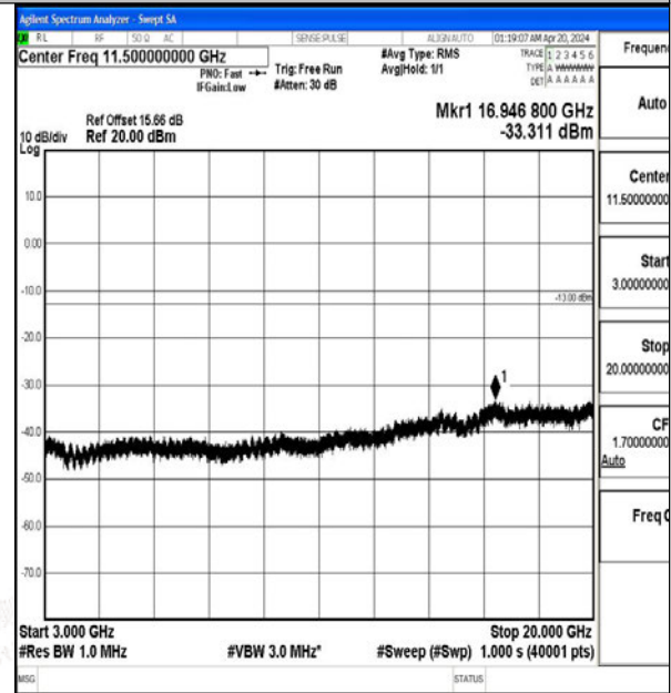
Band2_1.4MHz_16QAM_18900_1RB#0_3000~20000 _3000~20000
