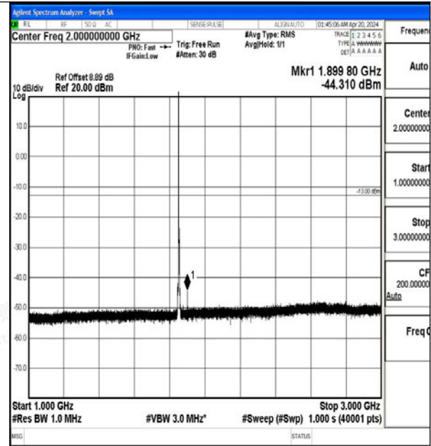
Band2_3MHz_QPSK_18615_1RB#0_1000~3000_1000~3000
