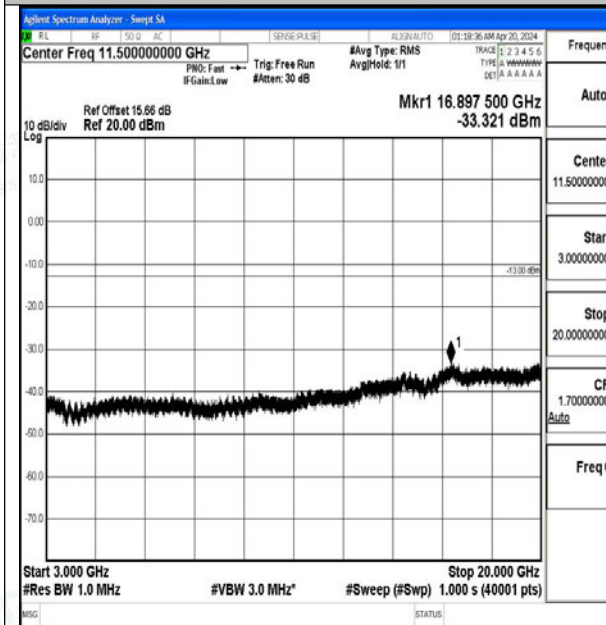
Band2_1.4MHz_QPSK_18900_1RB#0_3000~20000_3000~20000
