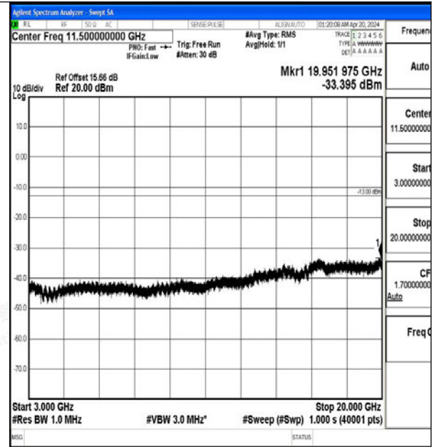
Band2_1.4MHz_16QAM_19193_1RB#0_3000~20000_3000~20000
