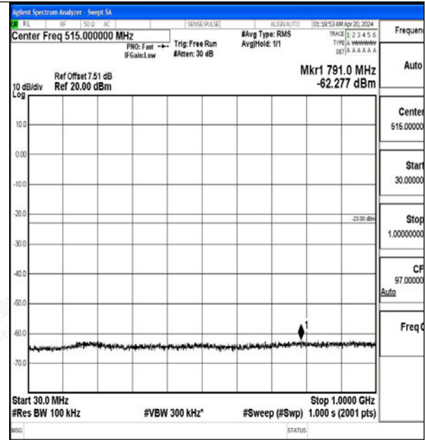
Band2_1.4MHz_16QAM_18900_1RB#0_30~1000_30 ~1000
