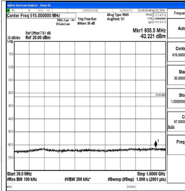
Band2_3MHz_QPSK_18615_1RB#0_30~1000_30~1000
