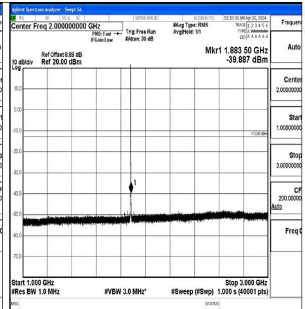
Band2_1.4MHz_QPSK_18900_1RB#0_1000~3000_1000~3000
