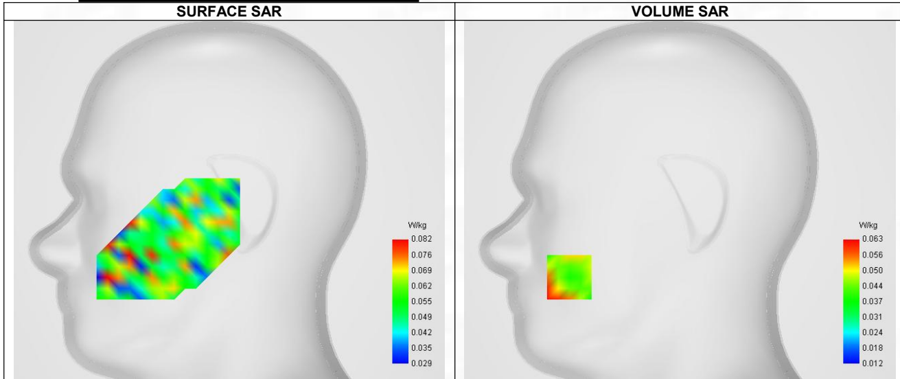
Maximum location: X=-80.00, Y=-56.00 ; SAR Peak: 0.14 W/kg
