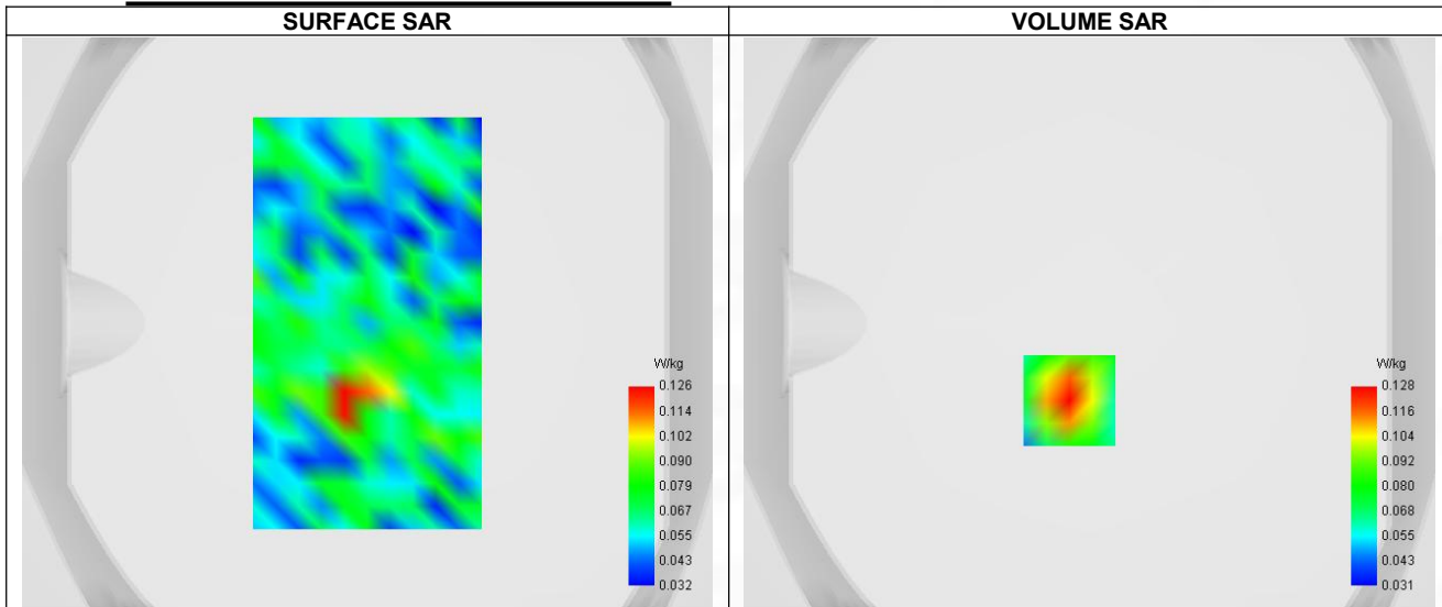
Maximum location: X=-7.00, Y=-27.00 ; SAR Peak: 0.22 W/kg
