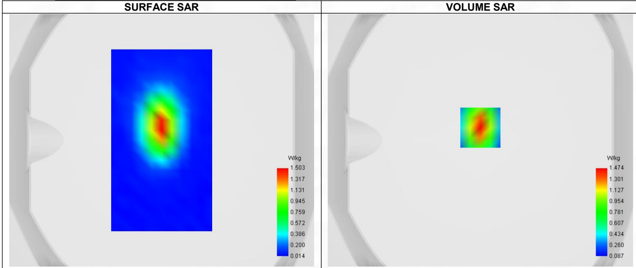
Maximum location: X=0.00, Y=10.00 ; SAR Peak: 2.17 W/kg
