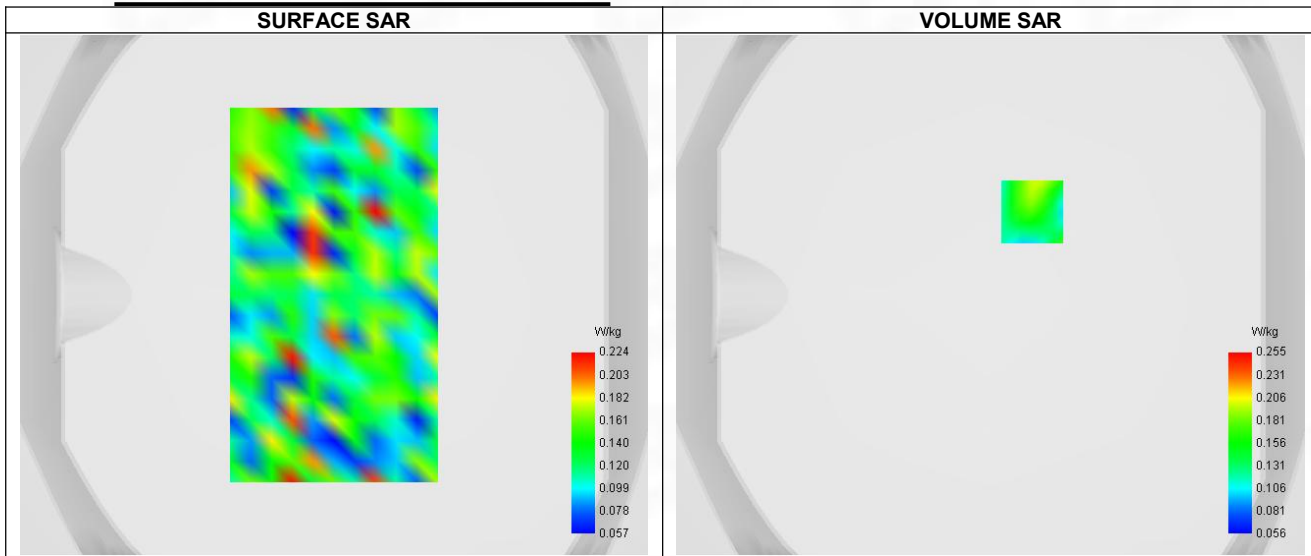
Maximum location: X=16.00, Y=32.00 ; SAR Peak: 0.26 W/kg
