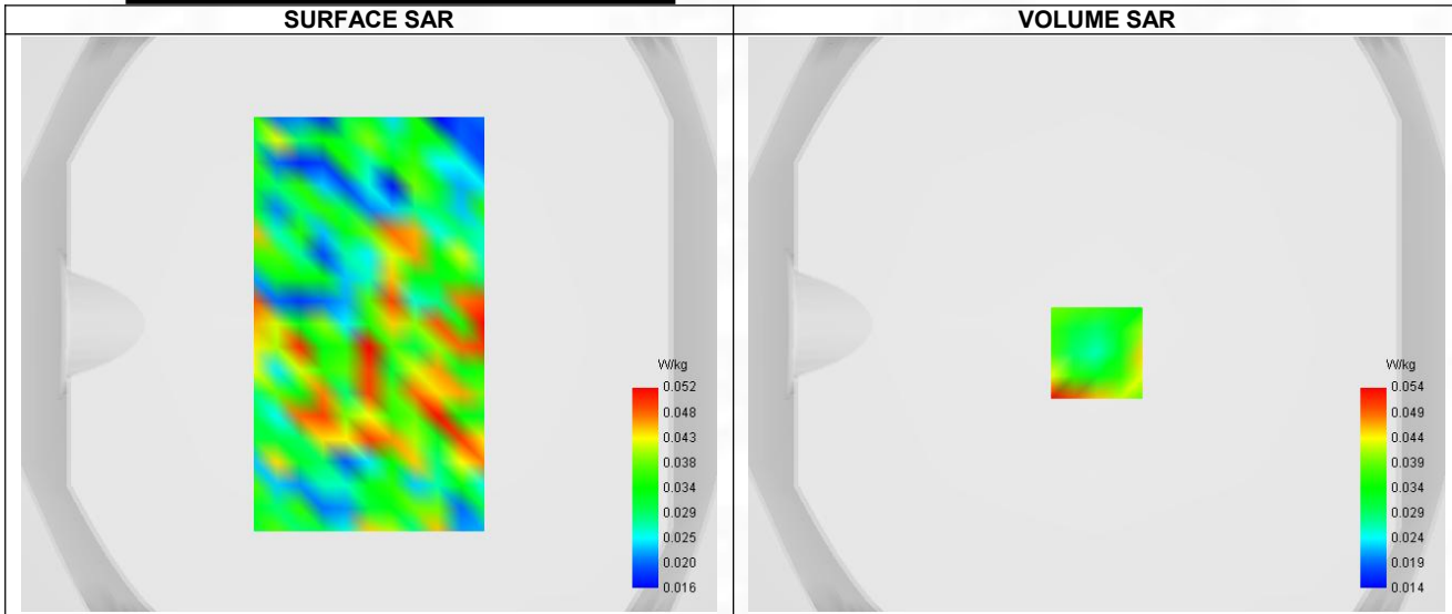
Maximum location: X=0.00, Y=-10.00 ; SAR Peak: 0.07 W/kg
