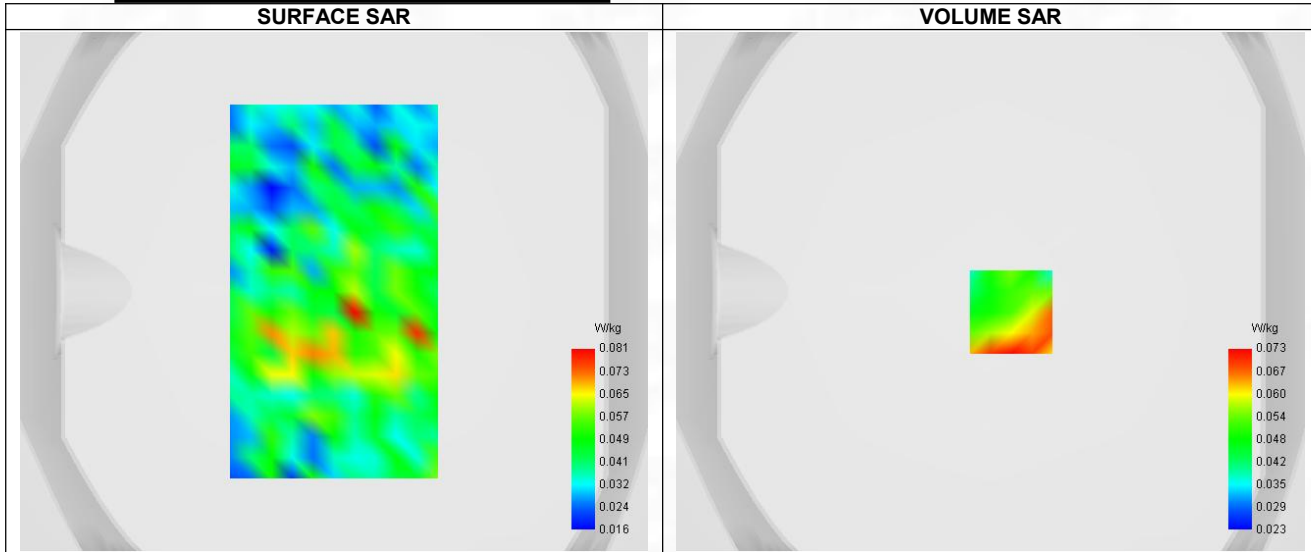
Maximum location: X=8.00, Y=-8.00 ; SAR Peak: 0.13 W/kg
