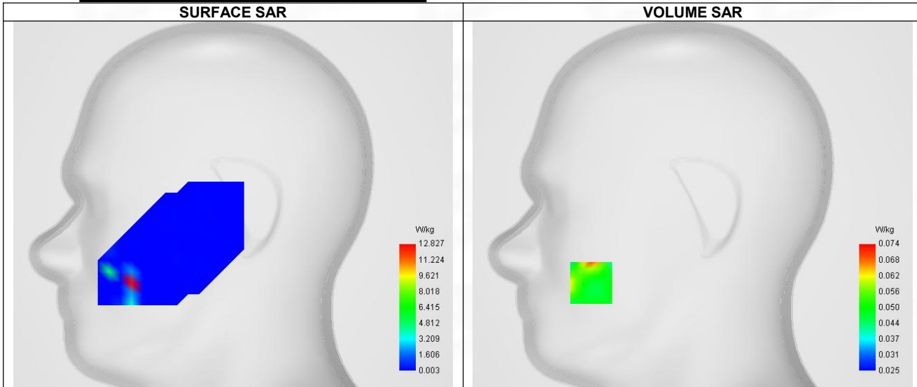
Maximum location: X=-72.00, Y=-56.00 ; SAR Peak: 0.09 W/kg
