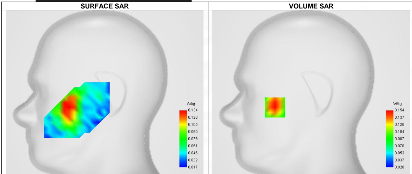
Maximum location: X=-57.00, Y=-24.00 ; SAR Peak: 0.21 W/kg
