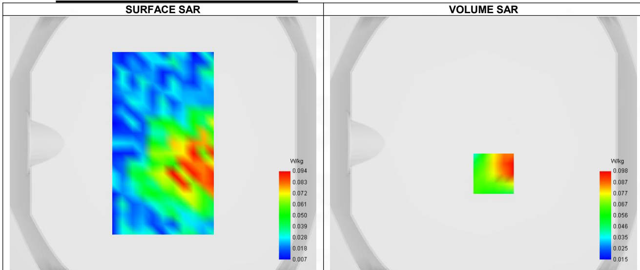
Maximum location: X=8.00, Y=-24.00 ; SAR Peak: 0.18 W/kg
