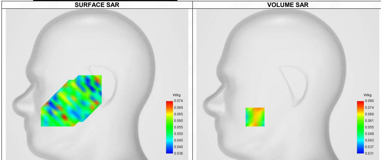
Maximum location: X=-56.00, Y=-56.00 ; SAR Peak: 0.12 W/kg
