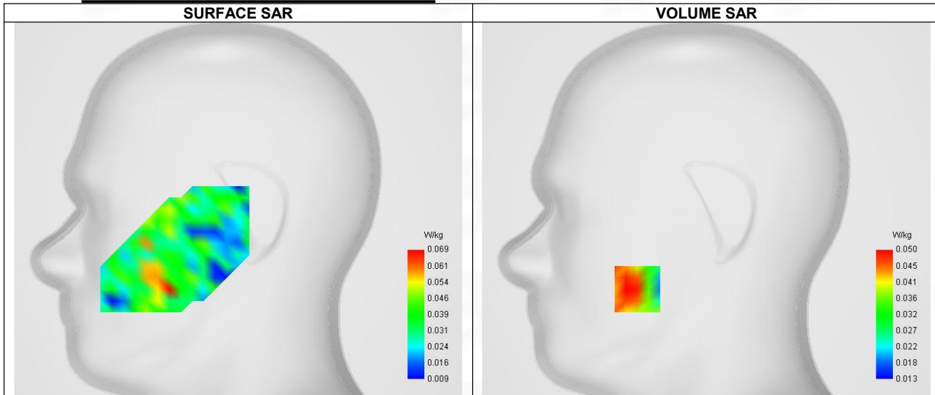
Maximum location: X=-48.00, Y=-56.00 ; SAR Peak: 0.08 W/kg
