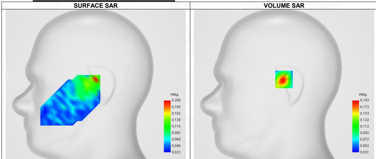
Maximum location: X=0.00, Y=8.00 ; SAR Peak: 0.32 W/kg
