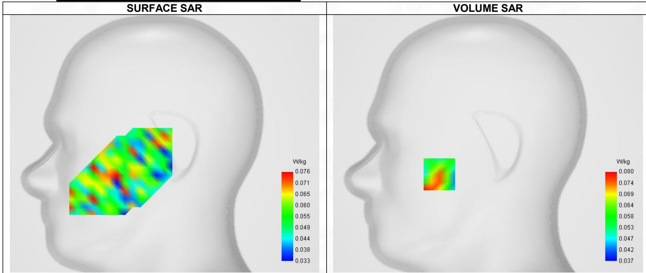
Maximum location: X=-49.00, Y=-31.00 ; SAR Peak: 0.10 W/kg
