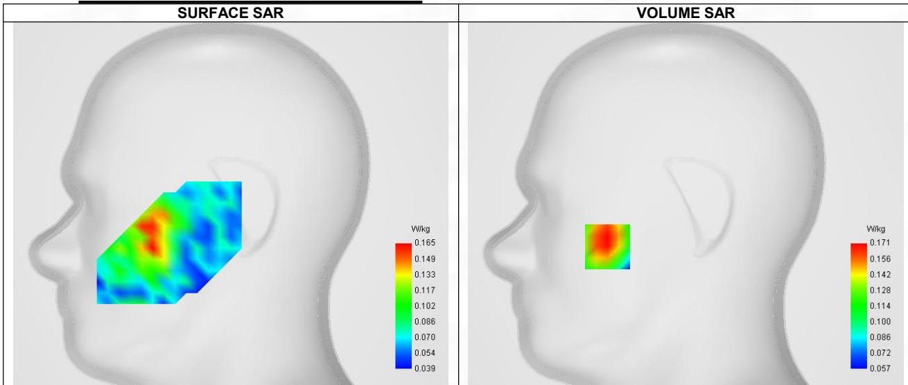
Maximum location: X=-56.00, Y=-31.00 ; SAR Peak: 0.25 W/kg
