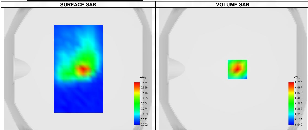
Maximum location: X=8.00, Y=-1.00 ; SAR Peak: 1.24 W/kg
