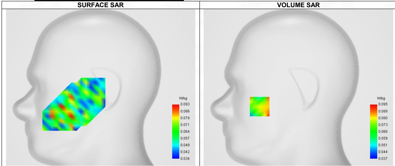
Maximum location: X=-64.00, Y=-32.00 ; SAR Peak: 0.14 W/kg
