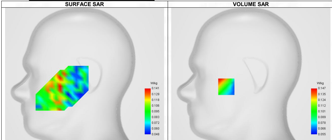
Maximum location: X=-48.00, Y=-25.00 ; SAR Peak: 0.24 W/kg
