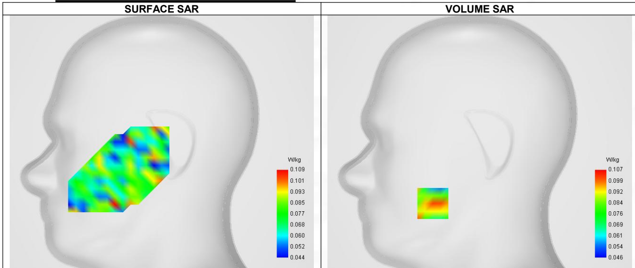
Maximum location: X=-48.00, Y=-63.00 ; SAR Peak: 0.15 W/kg
