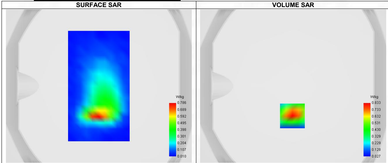
Maximum location: X=-1.00, Y=-39.00 ; SAR Peak: 1.51 W/kg
