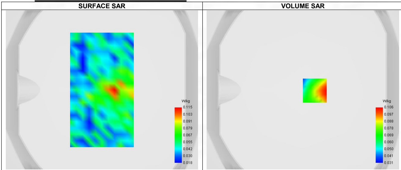
Maximum location: X=15.00, Y=-1.00 ; SAR Peak: 0.20 W/kg
