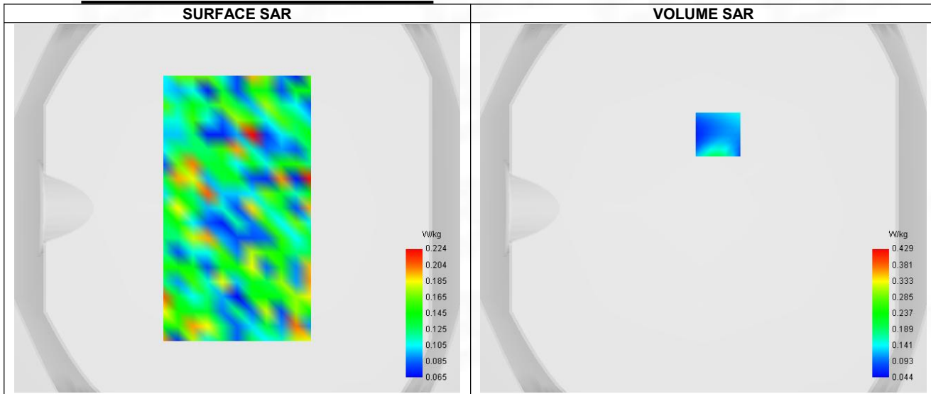
Maximum location: X=8.00, Y=40.00 ; SAR Peak: 0.24 W/kg
