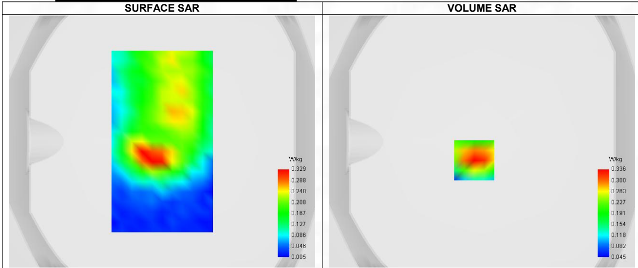
Maximum location: X=-6.00, Y=-15.00 ; SAR Peak: 0.48 W/kg
