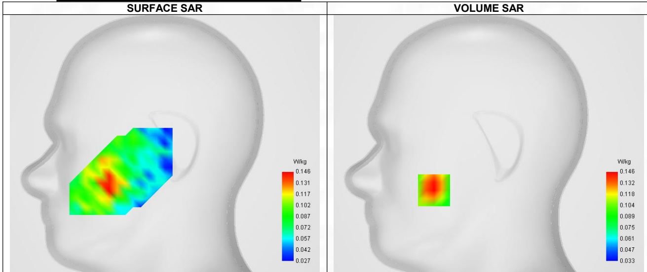
Maximum location: X=-55.00, Y=-47.00 ; SAR Peak: 0.21 W/kg
