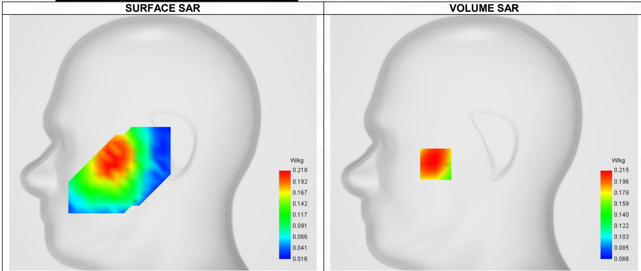
Maximum location: X=-49.00, Y=-22.00 ; SAR Peak: 0.26 W/kg
