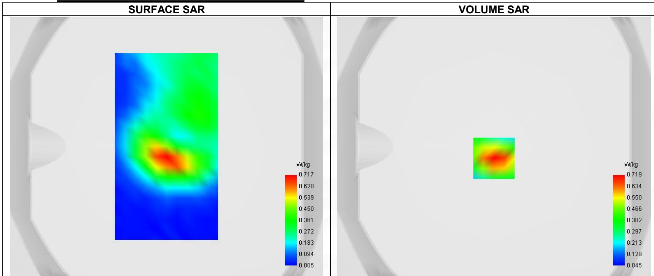
Maximum location: X=0.00, Y=-9.00 ; SAR Peak: 1.06 W/kg
