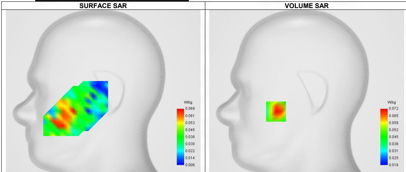
Maximum location: X=-49.00, Y=-33.00 ; SAR Peak: 0.13 W/kg
