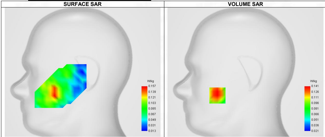
Maximum location: X=-56.00, Y=-47.00 ; SAR Peak: 0.18 W/kg
