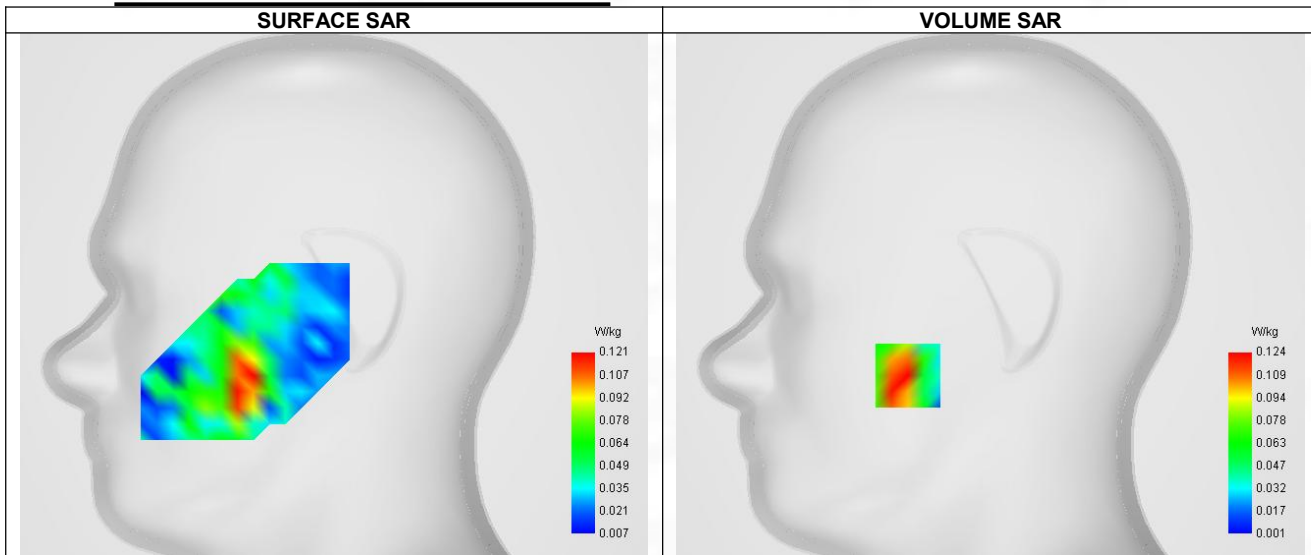
Maximum location: X=-41.00, Y=-40.00 ; SAR Peak: 0.22 W/kg
