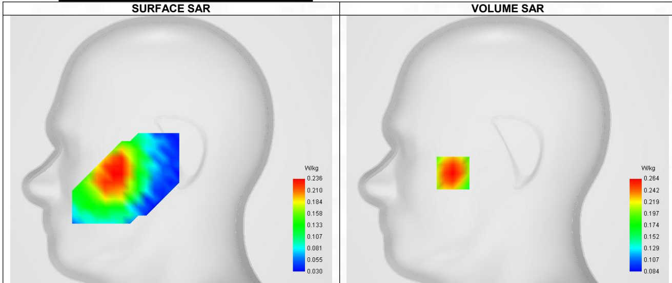
Maximum location: X=-53.00, Y=-23.00 ; SAR Peak: 0.30 W/kg
