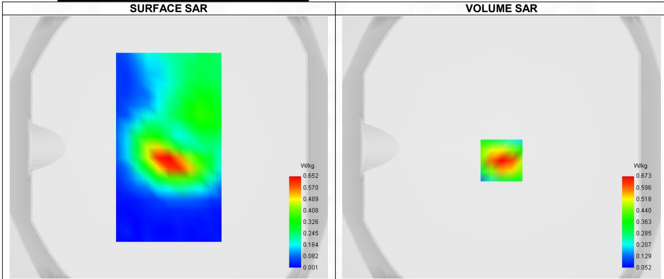
Maximum location: X=0.00, Y=-10.00 ; SAR Peak: 1.03 W/kg
