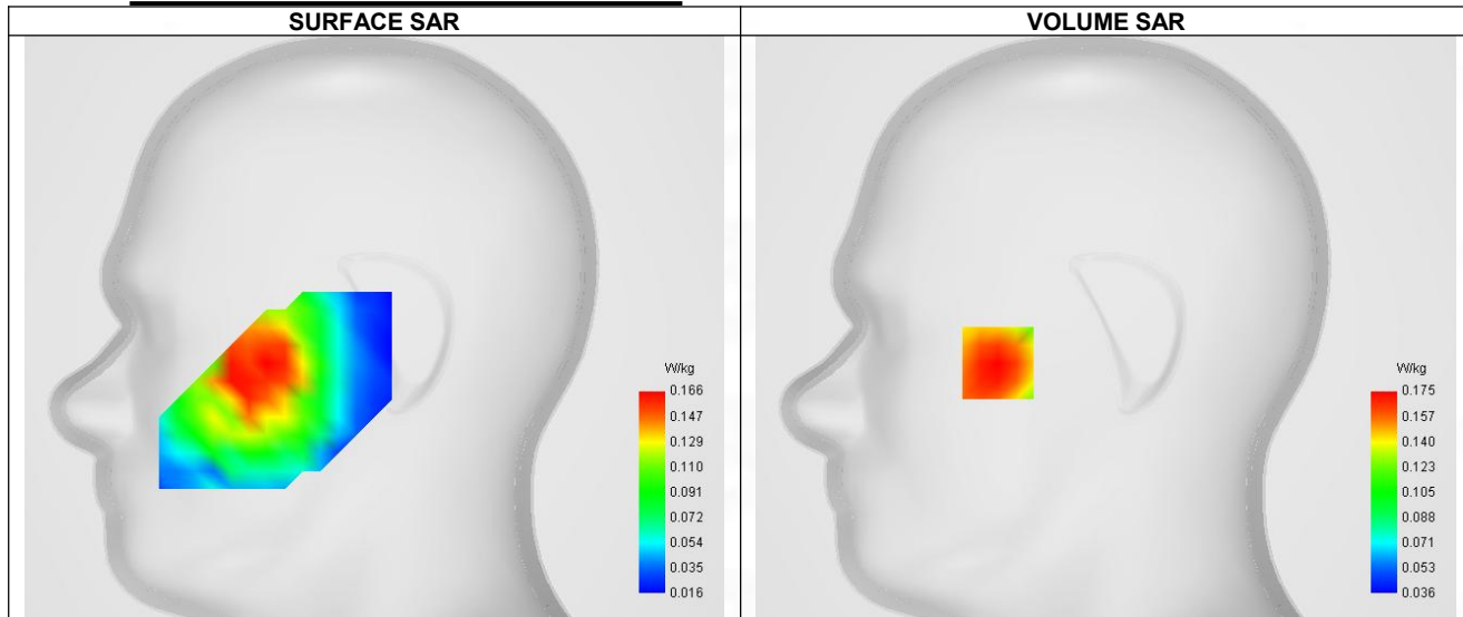
Maximum location: X=-48.00, Y=-16.00 ; SAR Peak: 0.22 W/kg
