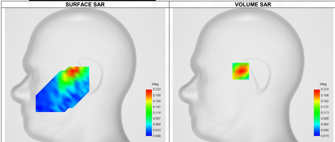
Maximum location: X=-24.00, Y=7.00 ; SAR Peak: 0.35 W/kg
