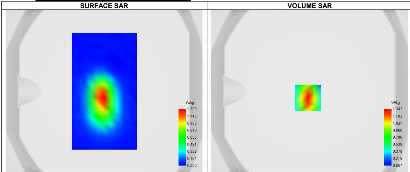
Maximum location: X=-2.00, Y=-8.00 ; SAR Peak: 2.02 W/kg
