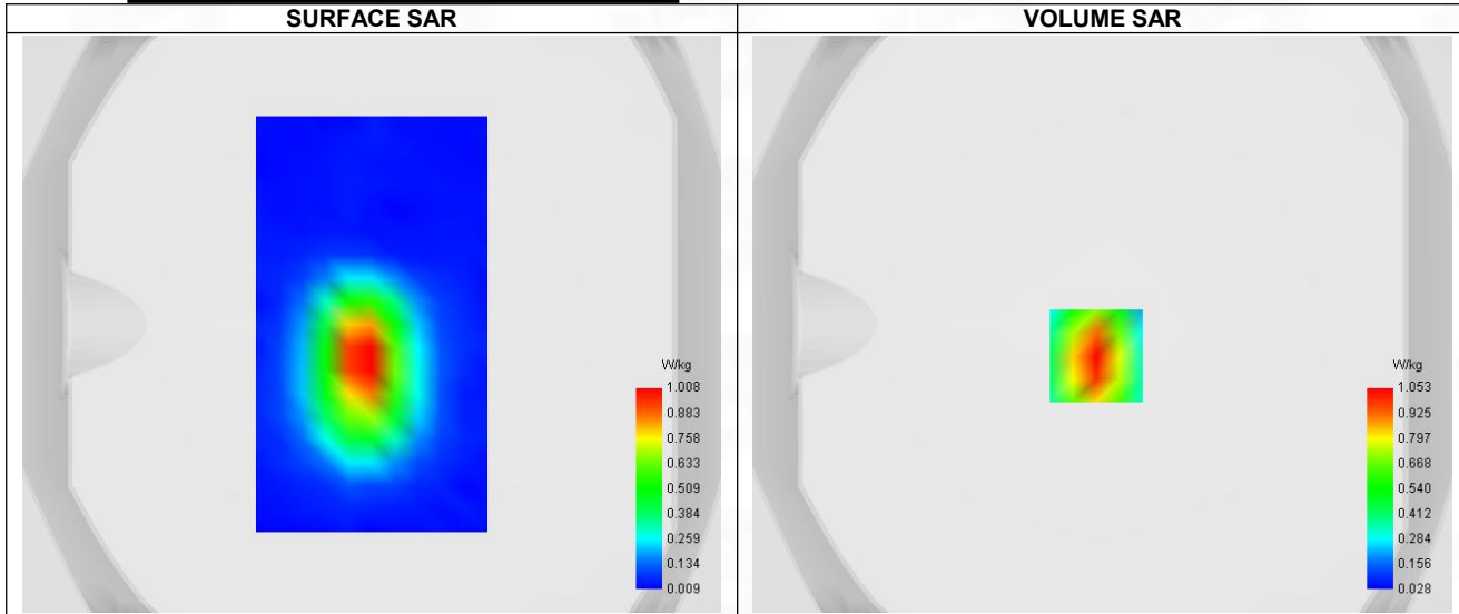
Maximum location: X=-2.00, Y=-11.00 ; SAR Peak: 1.56 W/kg
