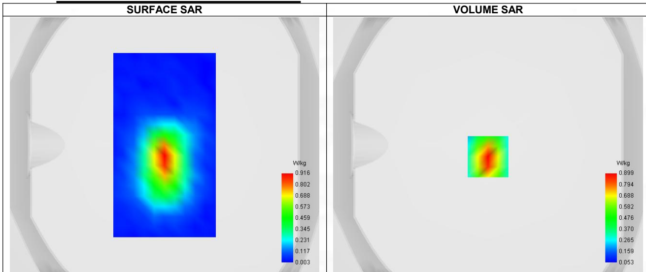
Maximum location: X=0.00, Y=-9.00 ; SAR Peak: 1.34 W/kg
