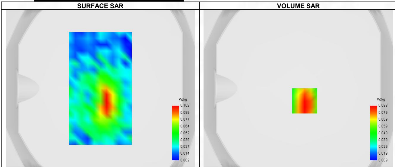
Maximum location: X=8.00, Y=-16.00 ; SAR Peak: 0.15 W/kg
