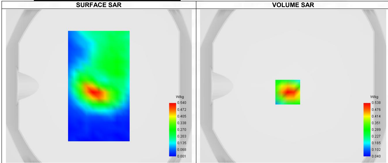
Maximum location: X=-7.00, Y=-8.00 ; SAR Peak: 0.82 W/kg
