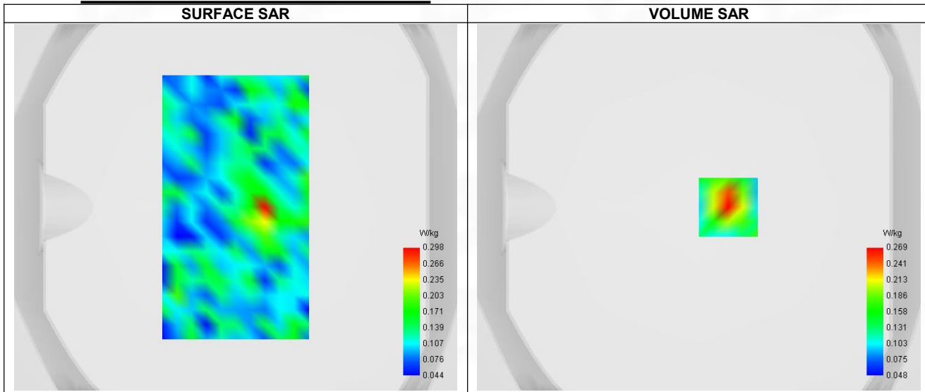
Maximum location: X=16.00, Y=0.00 ; SAR Peak: 0.36 W/kg
