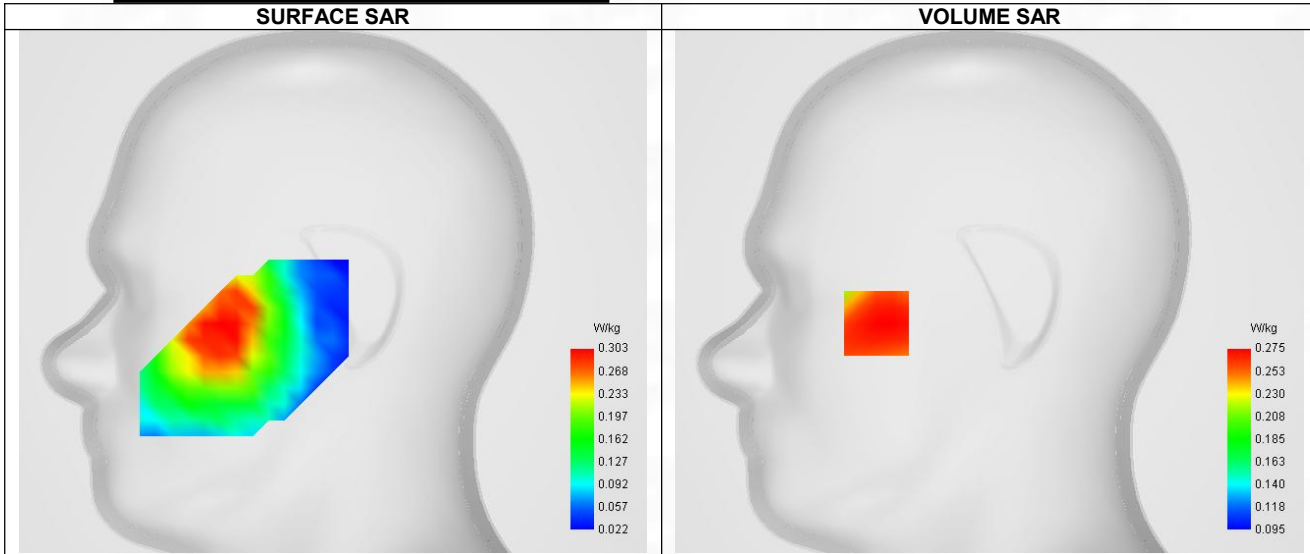
Maximum location: X=-56.00, Y=-16.00 ; SAR Peak: 0.35 W/kg
