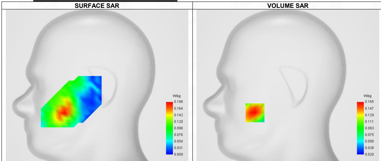
Maximum location: X=-56.00, Y=-47.00 ; SAR Peak: 0.24 W/kg
