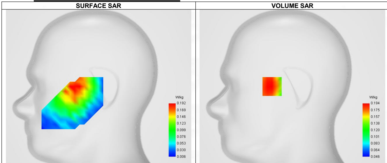
Maximum location: X=-34.00, Y=0.00 ; SAR Peak: 0.25 W/kg
