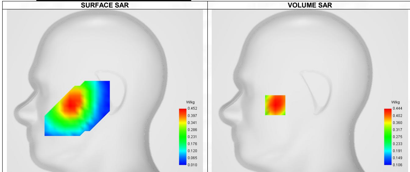
Maximum location: X=-55.00, Y=-23.00 ; SAR Peak: 0.56 W/kg
