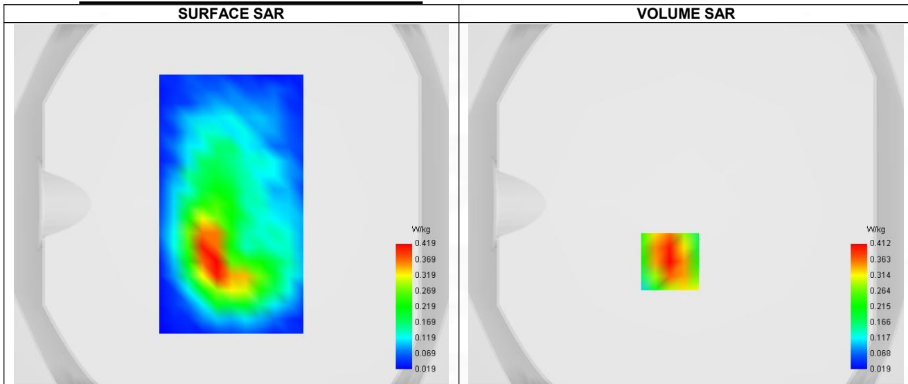
Maximum location: X=-9.00, Y=-32.00 ; SAR Peak: 0.70 W/kg
