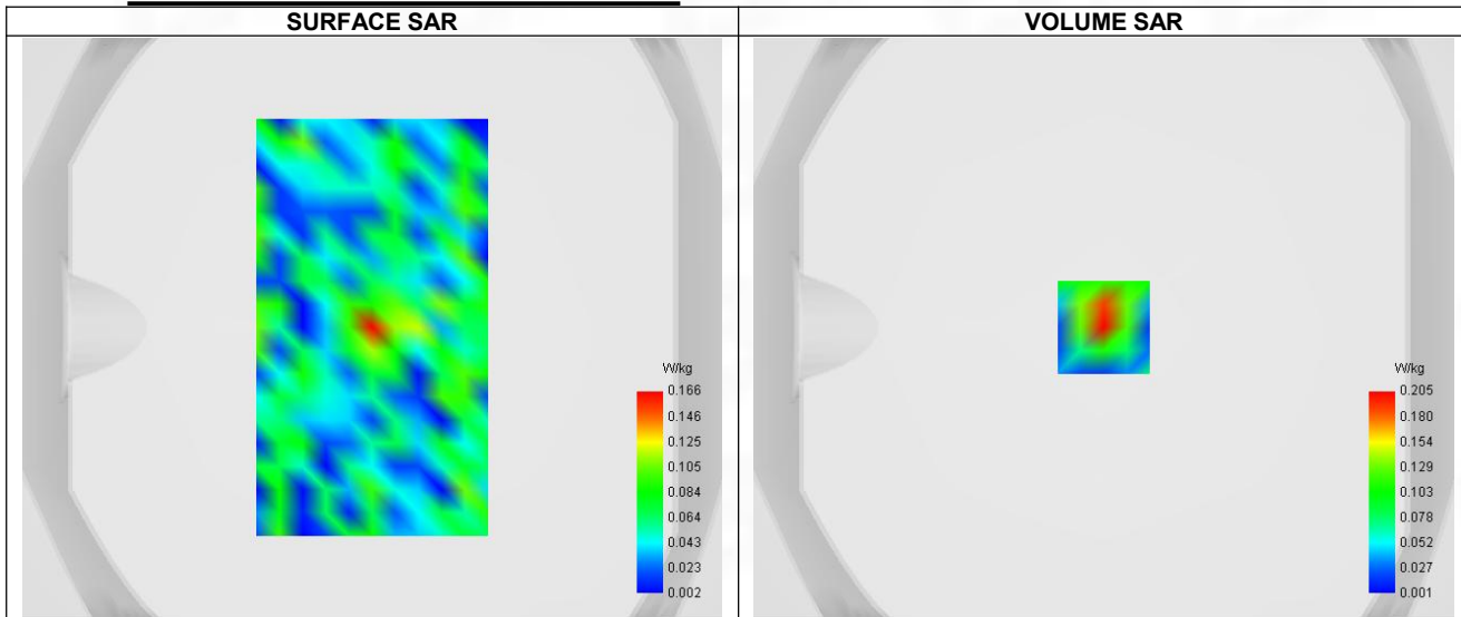
Maximum location: X=0.00, Y=0.00 ; SAR Peak: 0.28 W/kg
