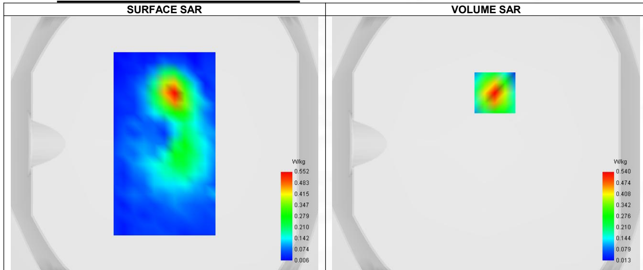
Maximum location: X=7.00, Y=40.00 ; SAR Peak: 0.94 W/kg
