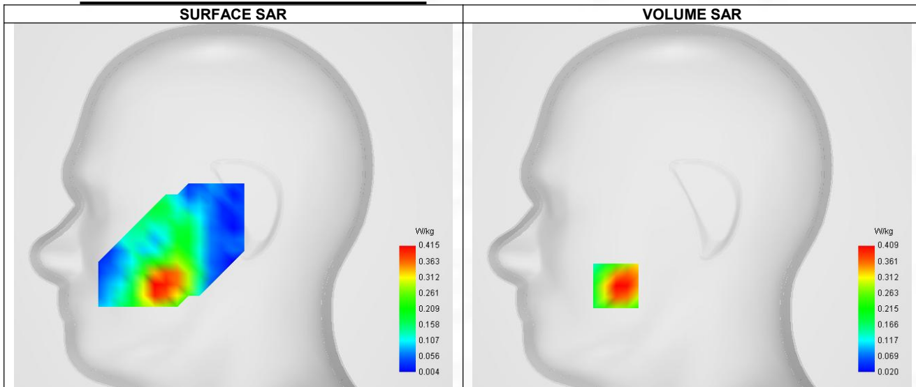
Maximum location: X=-54.00, Y=-57.00 ; SAR Peak: 0.61 W/kg
