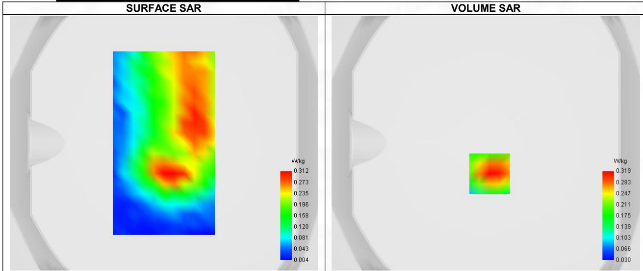
Maximum location: X=3.00, Y=-24.00 ; SAR Peak: 0.46 W/kg
