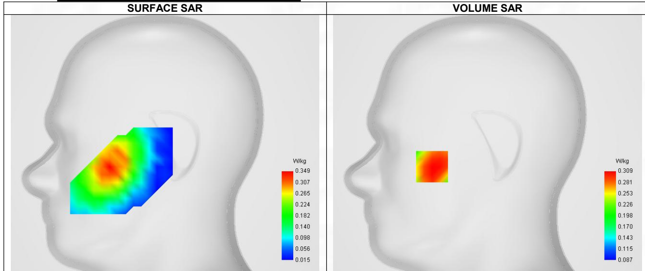
Maximum location: X=-56.00, Y=-24.00 ; SAR Peak: 0.39 W/kg
