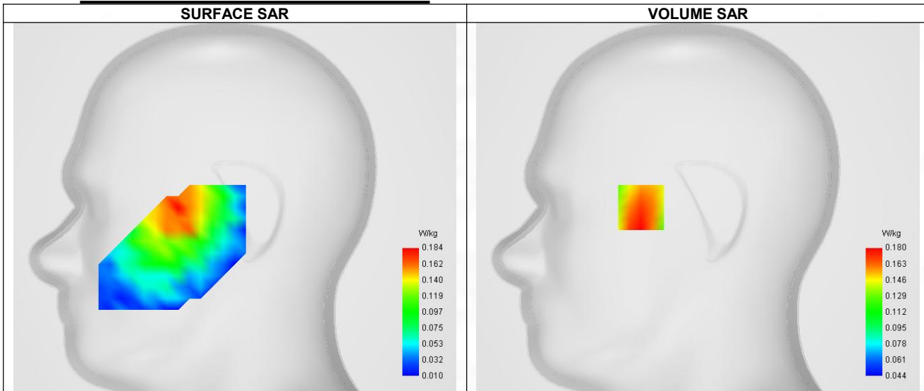
Maximum location: X=-40.00, Y=0.00 ; SAR Peak: 0.23 W/kg
