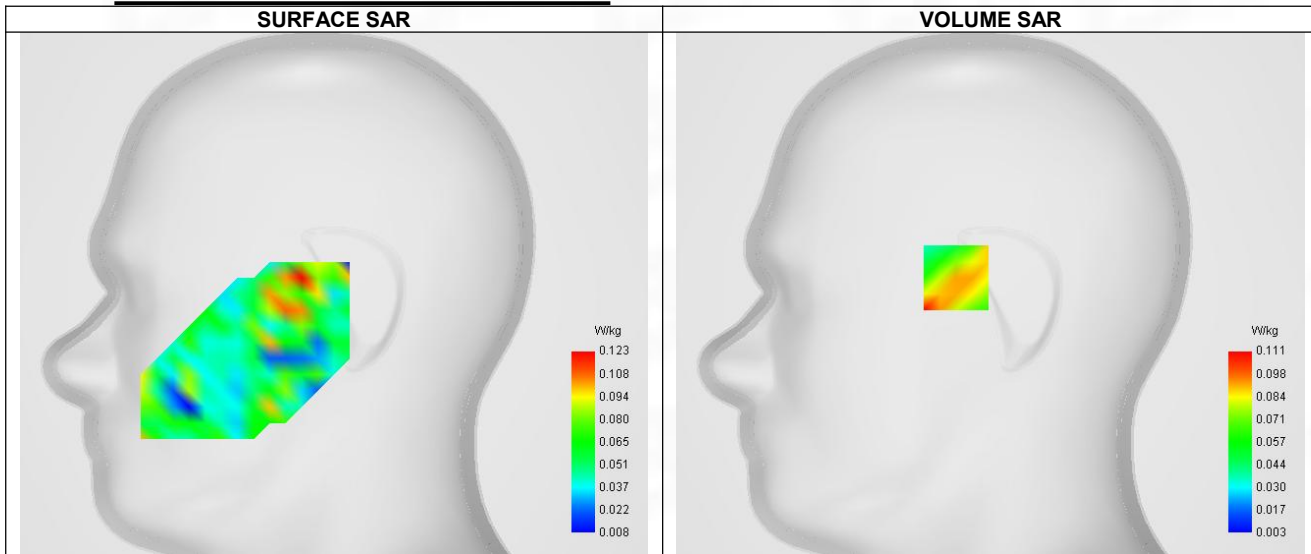
Maximum location: X=-17.00, Y=8.00 ; SAR Peak: 0.18 W/kg
