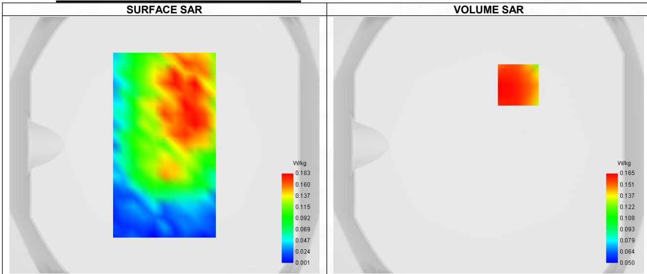
Maximum location: X=23.00, Y=47.00 ; SAR Peak: 0.21 W/kg
