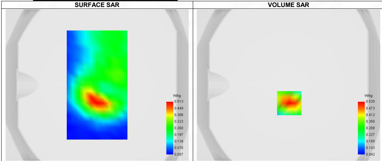
Maximum location: X=1.00, Y=-24.00 ; SAR Peak: 0.79 W/kg
