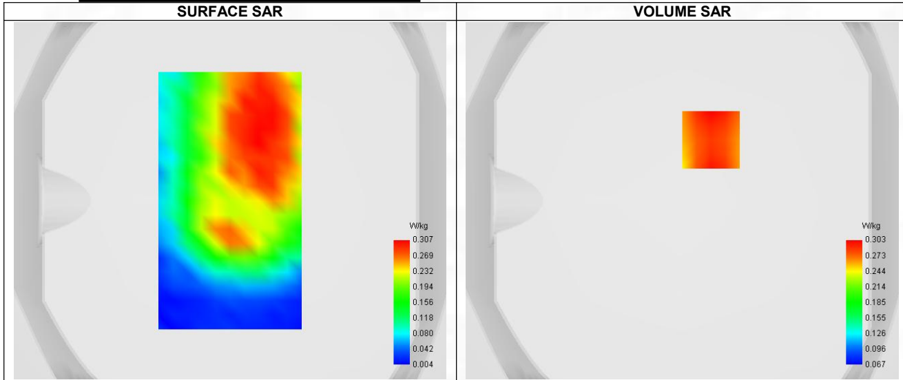
Maximum location: X=16.00, Y=34.00 ; SAR Peak: 0.38 W/kg
