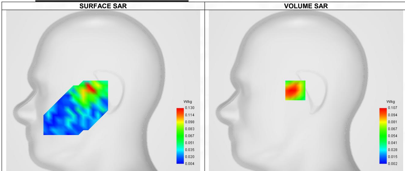
Maximum location: X=-17.00, Y=0.00 ; SAR Peak: 0.14 W/kg
