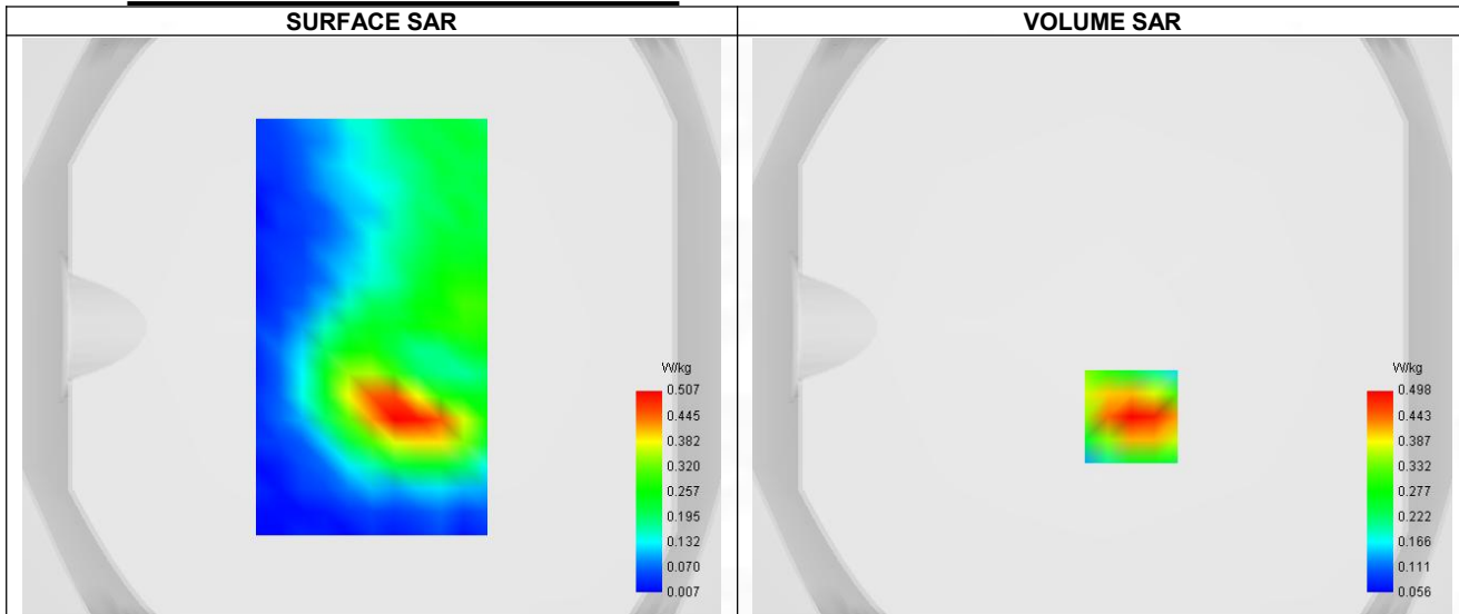
Maximum location: X=10.00, Y=-31.00 ; SAR Peak: 0.69 W/kg
