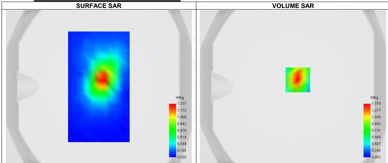
Maximum location: X=6.00, Y=9.00 ; SAR Peak: 2.17 W/kg
