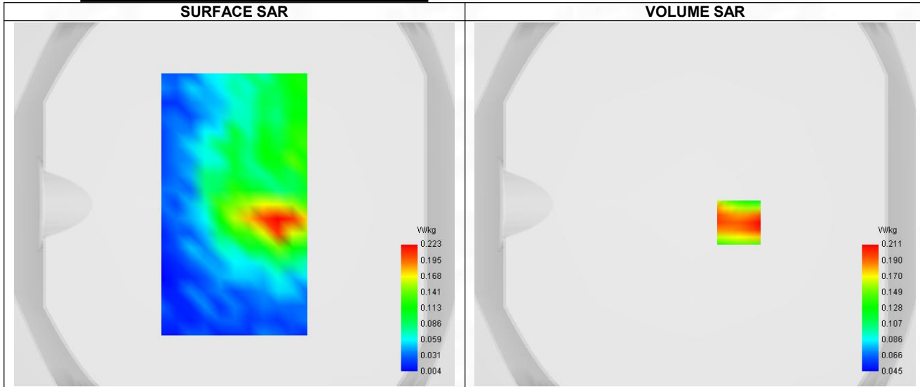
Maximum location: X=24.00, Y=-10.00 ; SAR Peak: 0.34 W/kg
