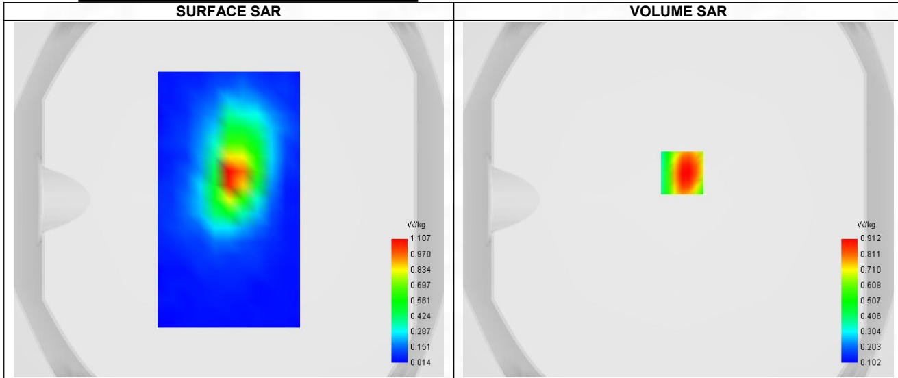
Maximum location: X=2.00, Y=15.00 ; SAR Peak: 1.60 W/kg
