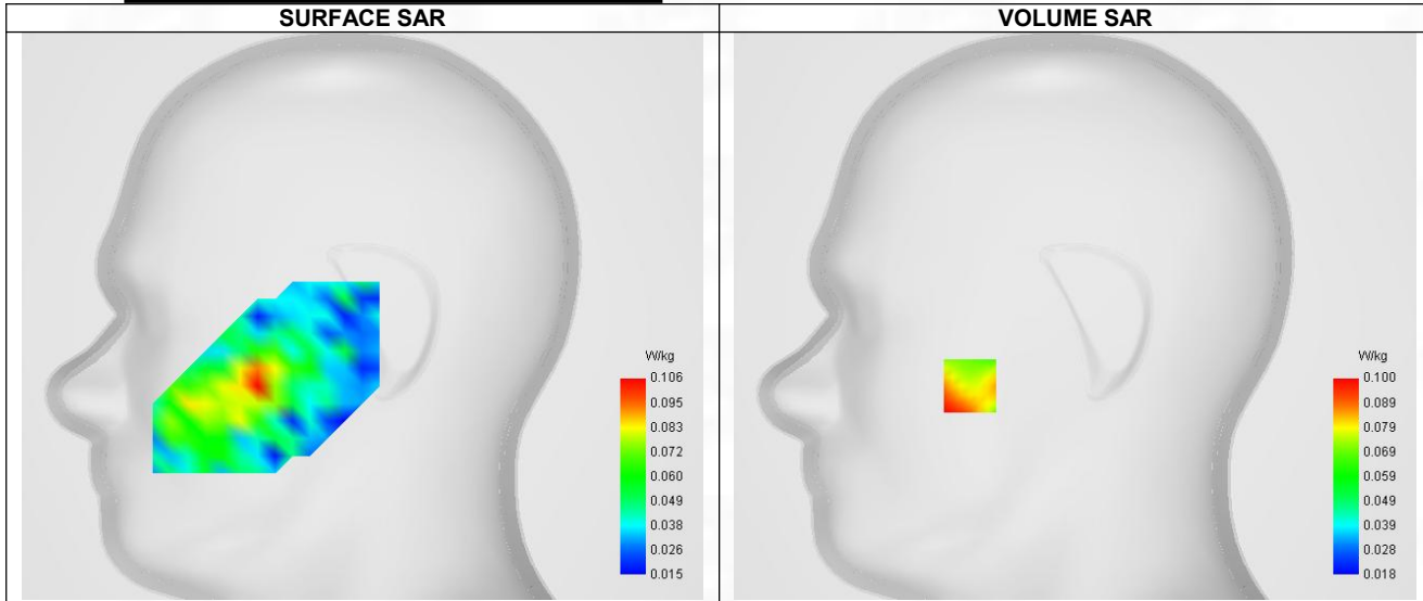
Maximum location: X=-48.00, Y=-32.00 ; SAR Peak: 0.18 W/kg
