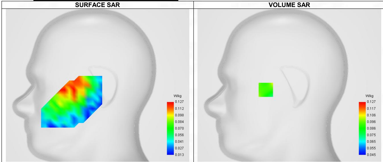
Maximum location: X=-40.00, Y=-8.00 ; SAR Peak: 0.17 W/kg
