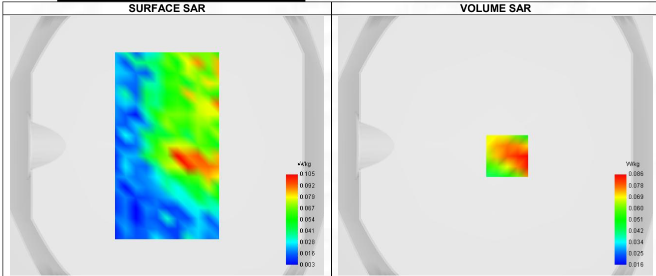
Maximum location: X=9.00, Y=-8.00 ; SAR Peak: 0.16 W/kg
