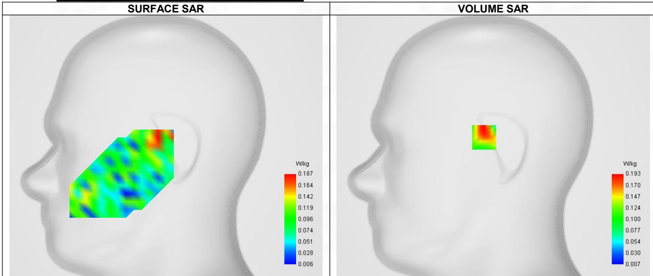
Maximum location: X=-9.00, Y=8.00 ; SAR Peak: 0.56 W/kg
