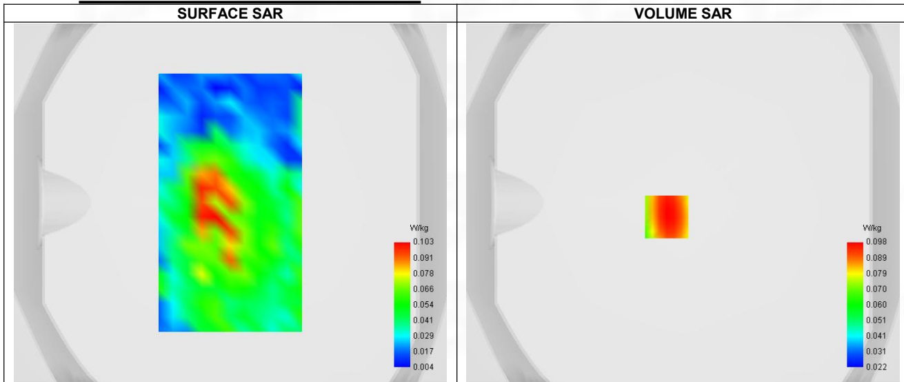
Maximum location: X=-9.00, Y=-8.00 ; SAR Peak: 0.17 W/kg
