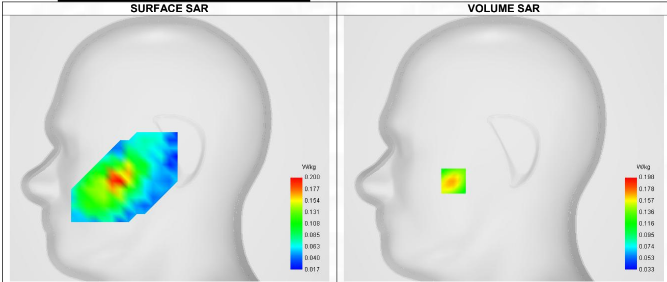
Maximum location: X=-49.00, Y=-32.00 ; SAR Peak: 0.30 W/kg
