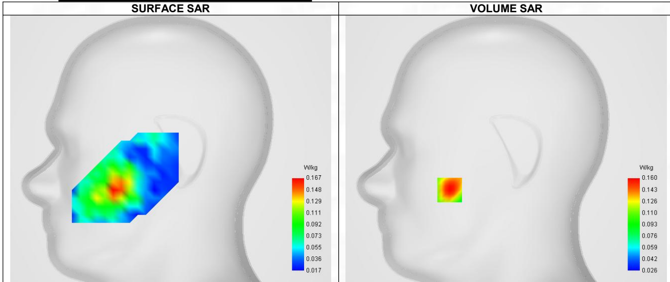
Maximum location: X=-55.00, Y=-40.00 ; SAR Peak: 0.31 W/kg
