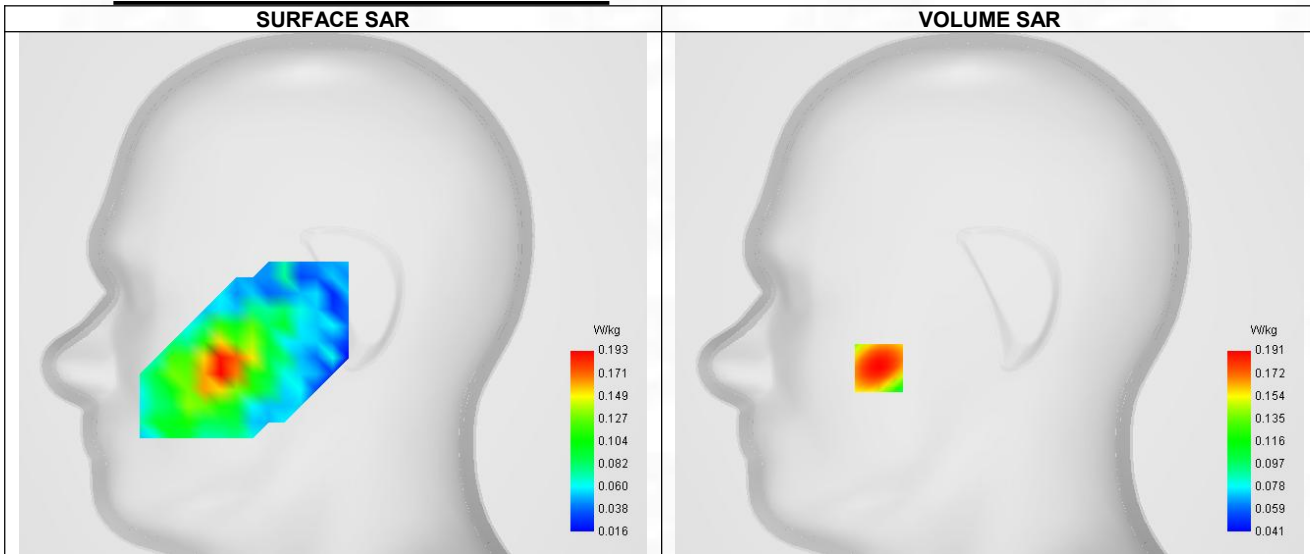
Maximum location: X=-55.00, Y=-37.00 ; SAR Peak: 0.46 W/kg
