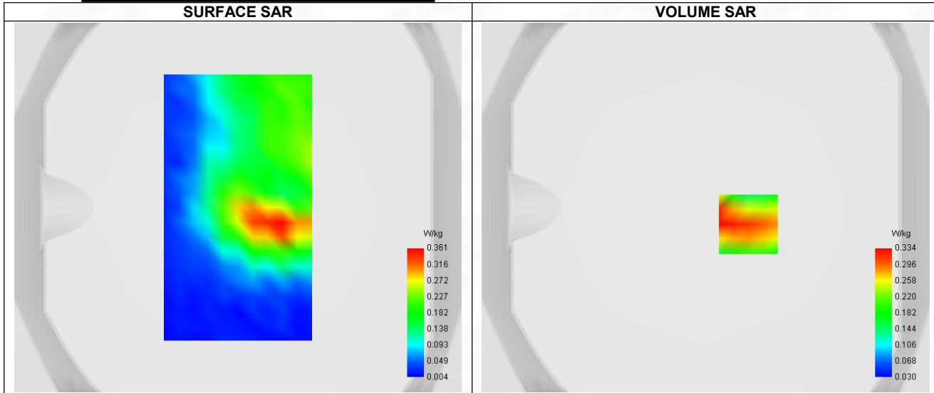
Maximum location: X=23.00, Y=-9.00 ; SAR Peak: 0.53 W/kg
