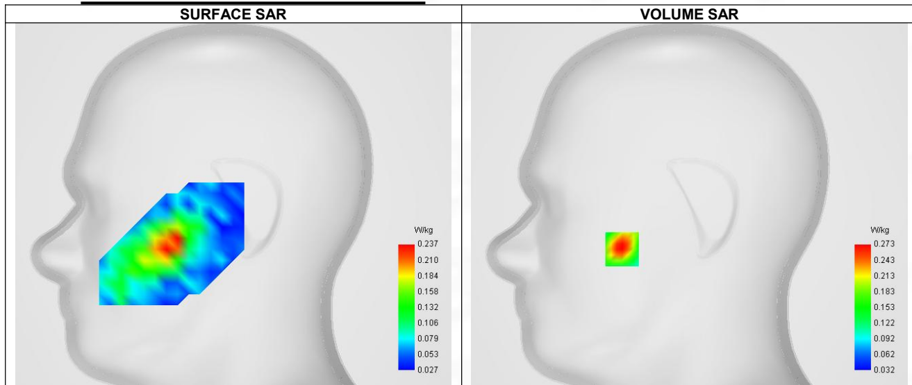
Maximum location: X=-48.00, Y=-32.00 ; SAR Peak: 0.58 W/kg
