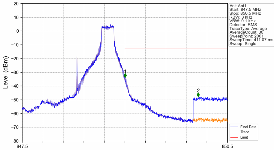
Band5_1.4MHz_16QAM_HCH_848.3MHz_RB_1_5_NTNV
