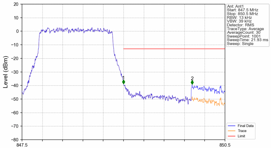
Band5_1.4MHz_16QAM_HCH_848.3MHz_RB_6_0_NTNV
