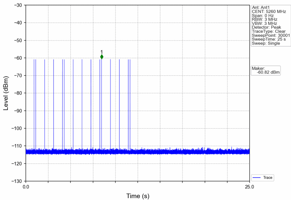
Signal Calibration_802.11a_2A_5260MHz_RadarType5_Trial0
