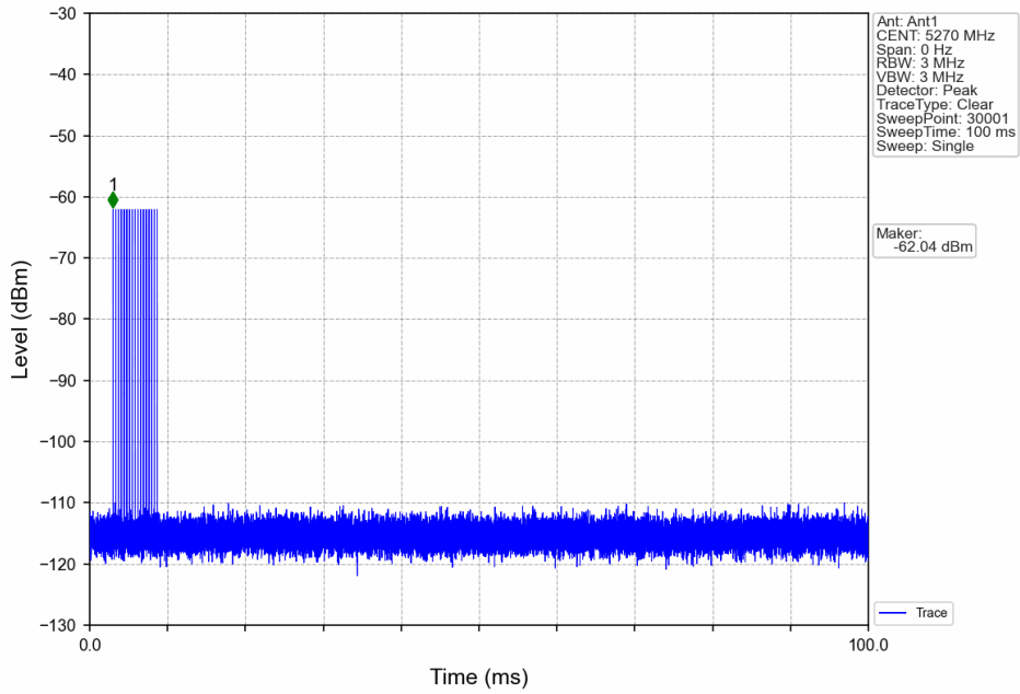
Signal Calibration_802.11n(HT40)_2A_5270MHz_RadarType4_Trial0
