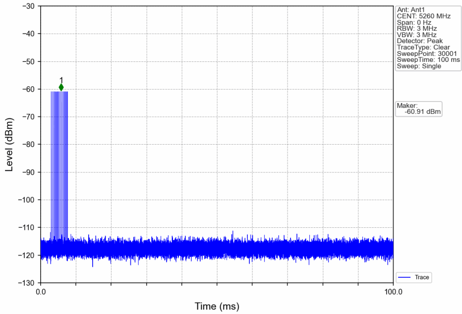
Signal Calibration_802.11a_2A_5260MHz_RadarType5_Trial0
