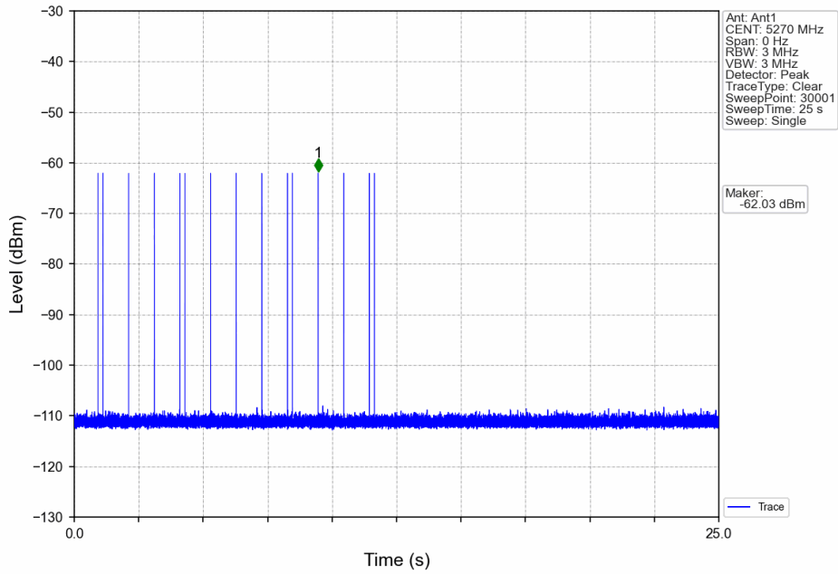
Signal Calibration_802.11n(HT40)_2A_5270MHz_RadarType6_Trial0
