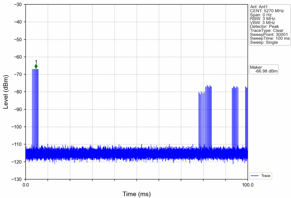
Signal Calibration_802.11n(HT40)_2A_5270MHz_RadarType6_Trial0
