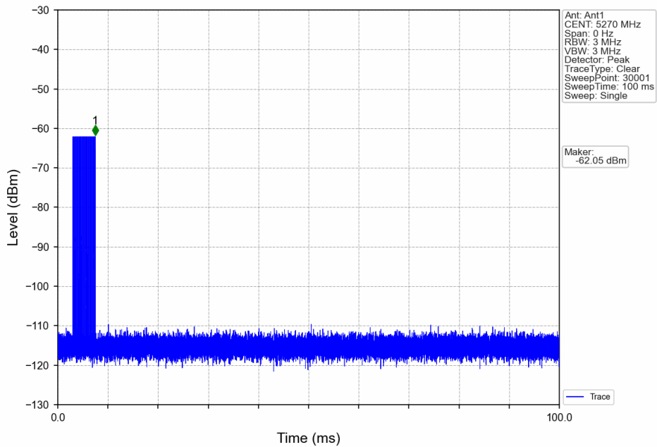
Signal Calibration_802.11n(HT40)_2A_5270MHz_RadarType2_Trial0
