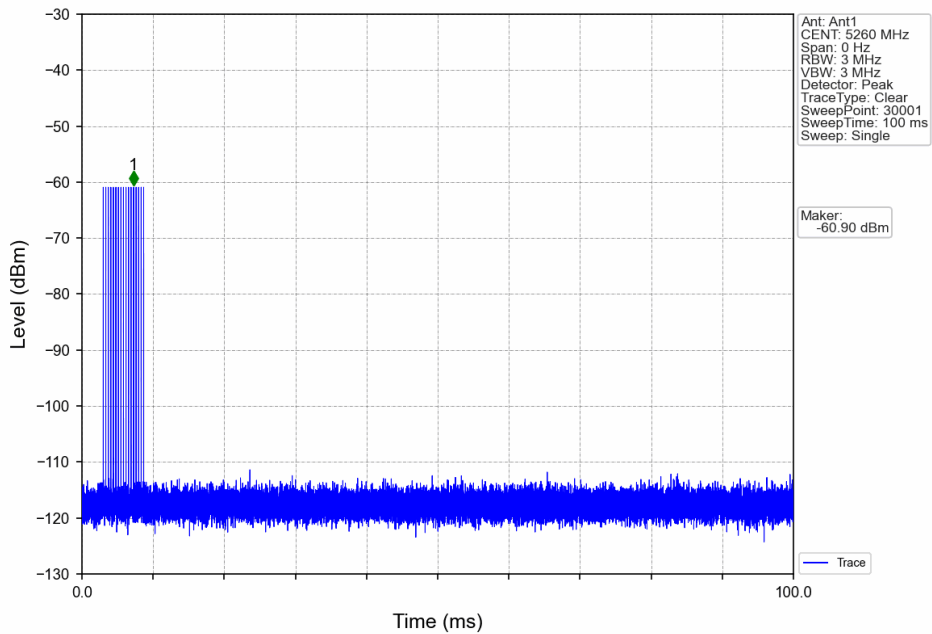
Signal Calibration_802.11a_2A_5260MHz_RadarType3_Trial0
