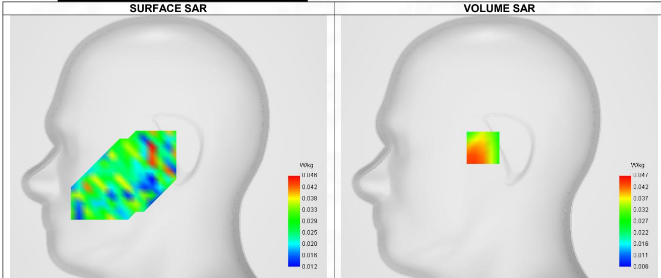
Maximum location: X=-16.00, Y=-1.00 ; SAR Peak: 0.08 W/kg
