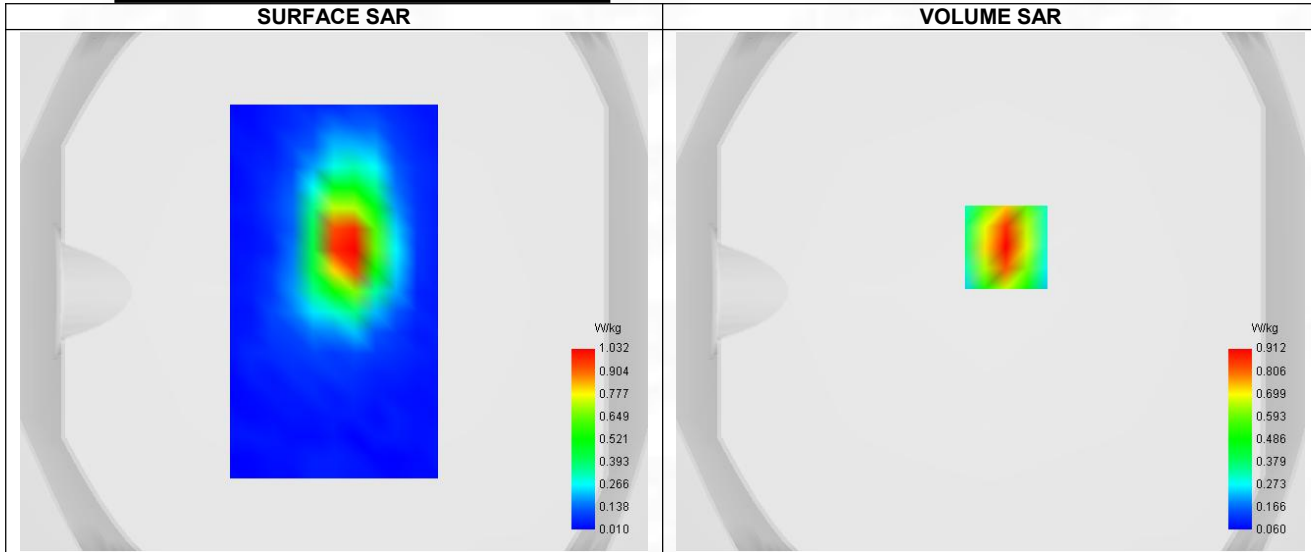
Maximum location: X=6.00, Y=17.00 ; SAR Peak: 1.32 W/kg
