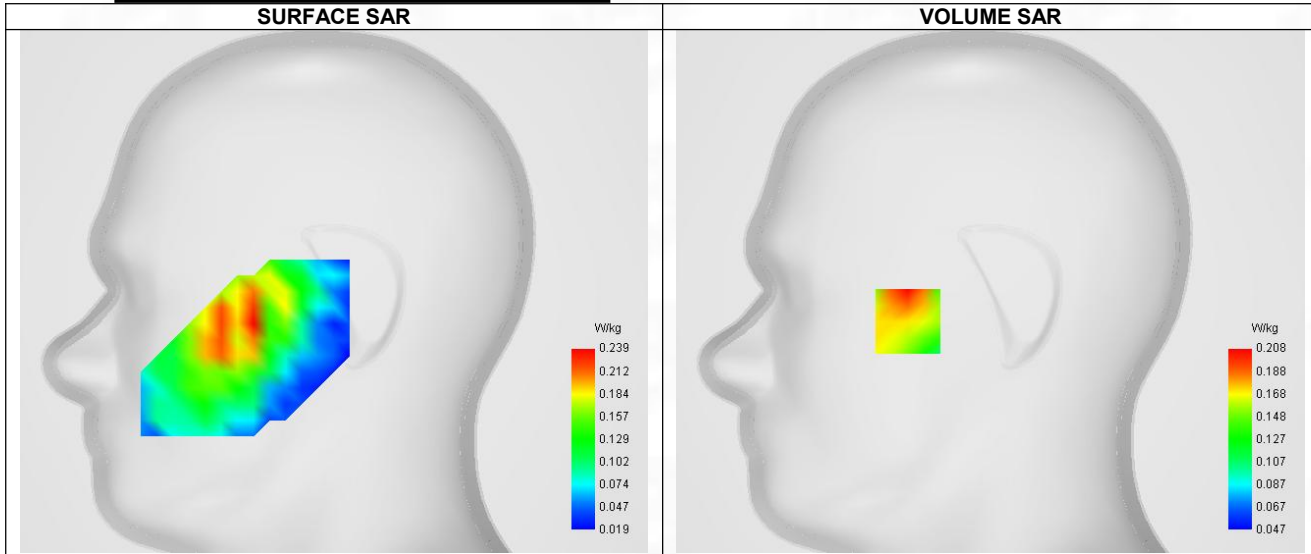
Maximum location: X=-41.00, Y=-15.00 ; SAR Peak: 0.29 W/kg
