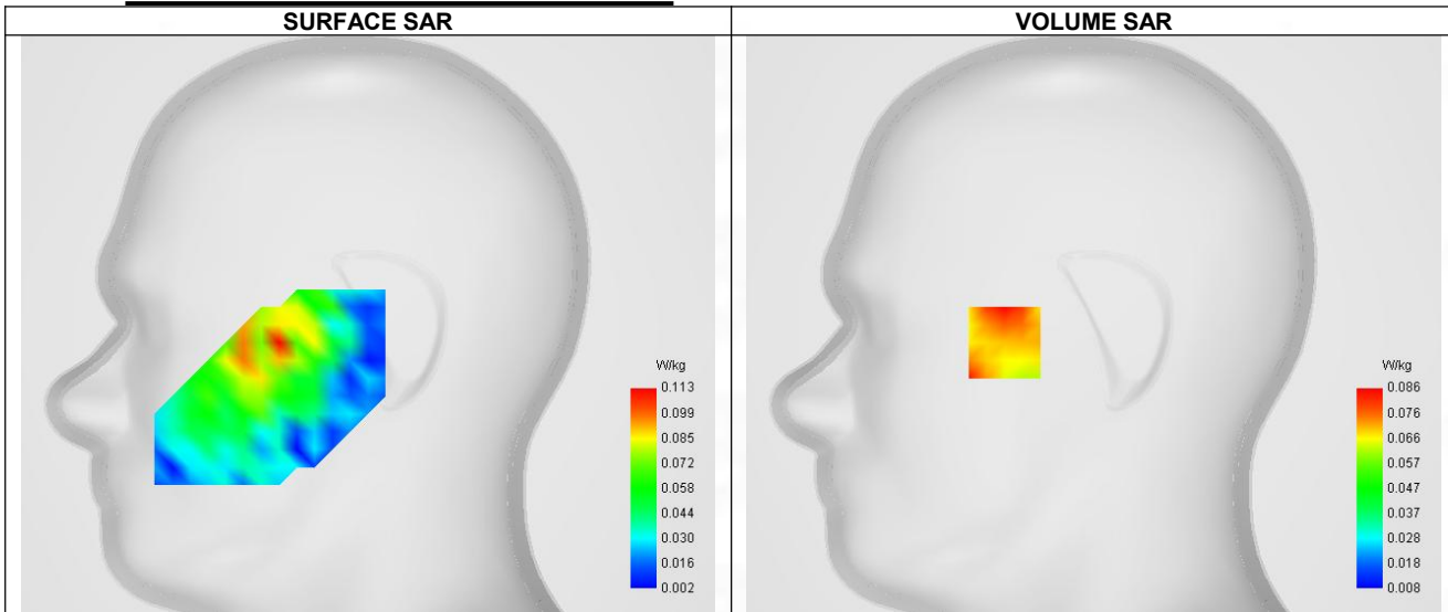
Maximum location: X=-40.00, Y=-8.00 ; SAR Peak: 0.12 W/kg
