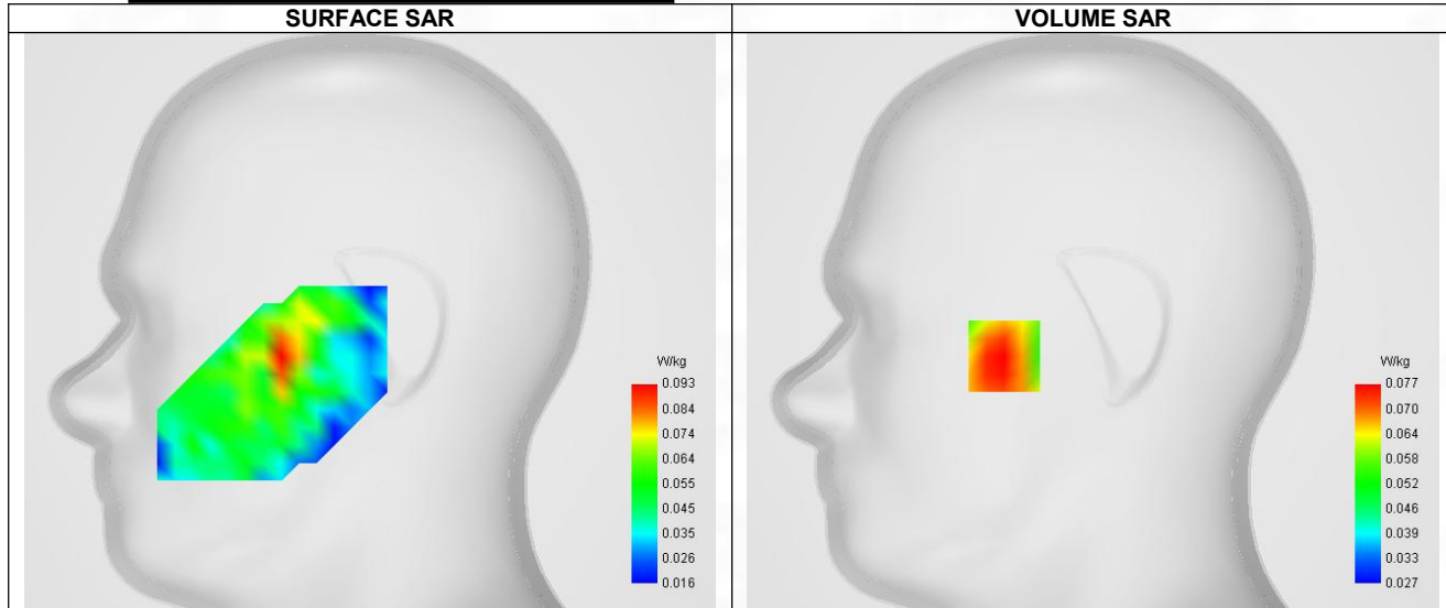
Maximum location: X=-40.00, Y=-16.00 ; SAR Peak: 0.14 W/kg
