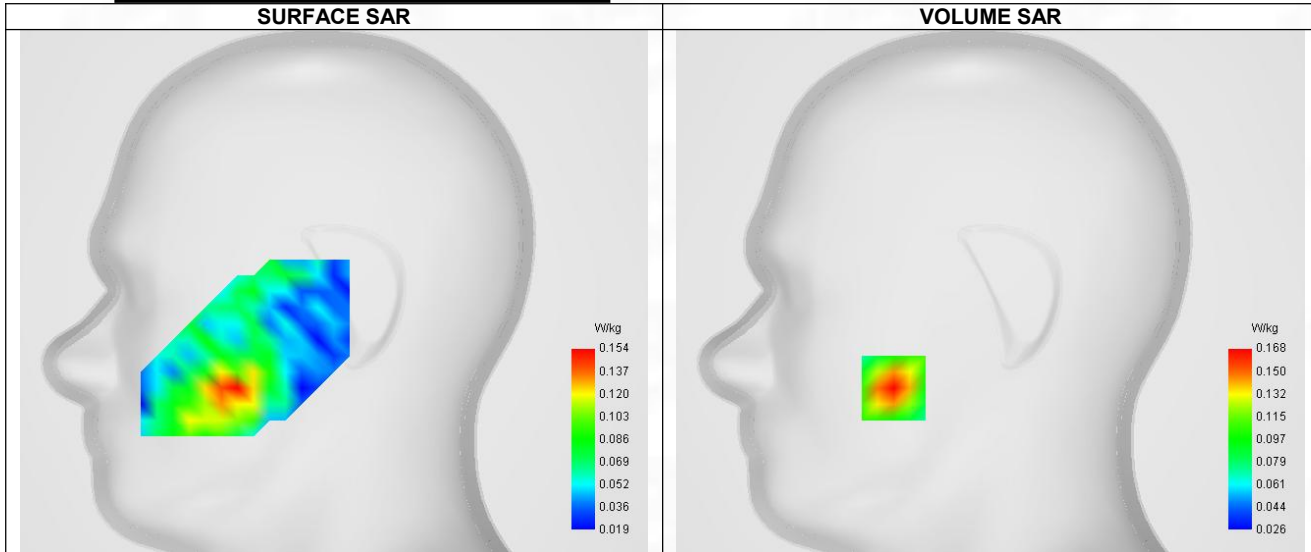
Maximum location: X=-48.00, Y=-48.00 ; SAR Peak: 0.28 W/kg
