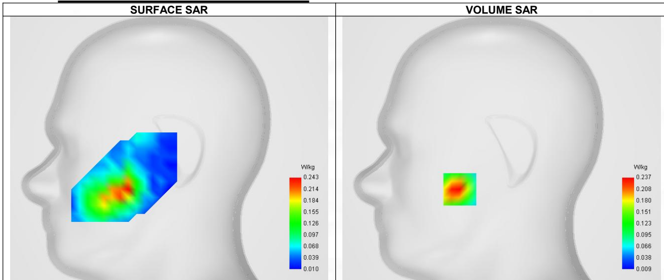
Maximum location: X=-41.00, Y=-40.00 ; SAR Peak: 0.37 W/kg
