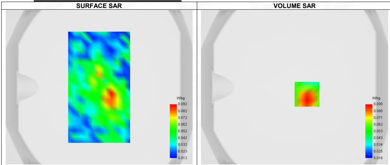
Maximum location: X=16.00, Y=-9.00 ; SAR Peak: 0.14 W/kg
