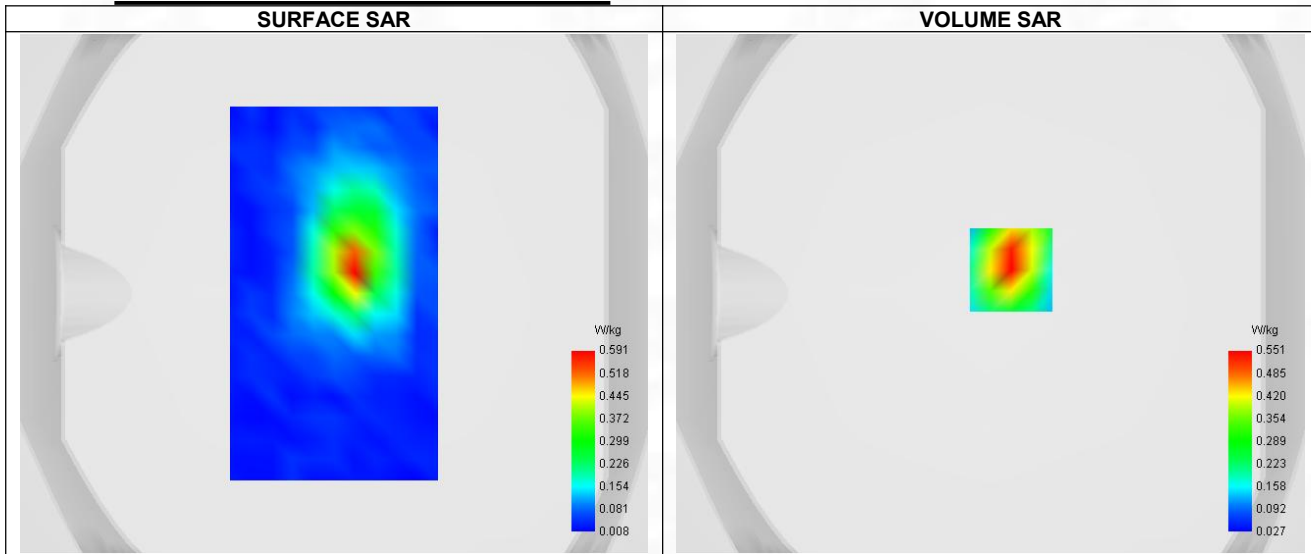
Maximum location: X=8.00, Y=9.00 ; SAR Peak: 0.93 W/kg
