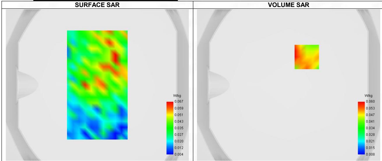
Maximum location: X=24.00, Y=37.00 ; SAR Peak: 0.09 W/kg
