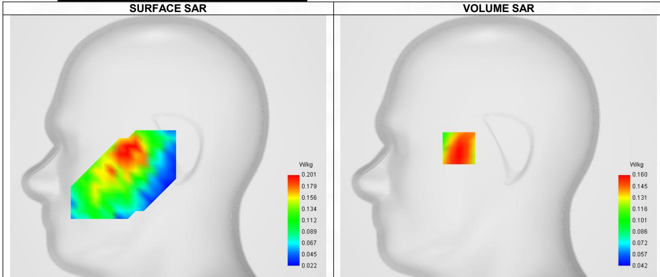
Maximum location: X=-39.00, Y=-2.00 ; SAR Peak: 0.22 W/kg
