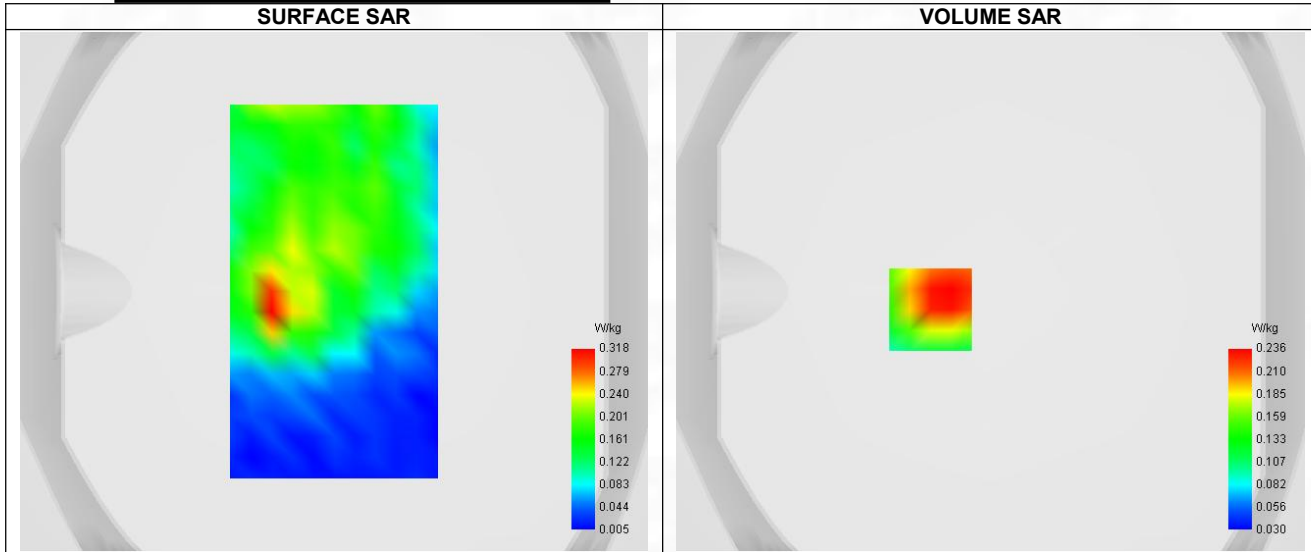
Maximum location: X=-23.00, Y=-7.00 ; SAR Peak: 0.41 W/kg
