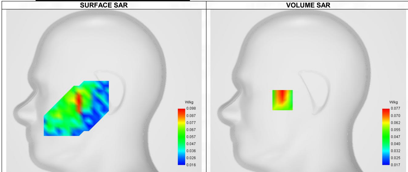
Maximum location: X=-41.00, Y=-15.00 ; SAR Peak: 0.11 W/kg
