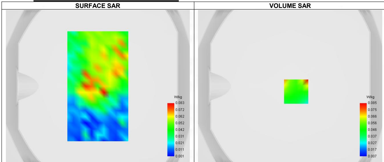
Maximum location: X=8.00, Y=-7.00 ; SAR Peak: 0.16 W/kg
