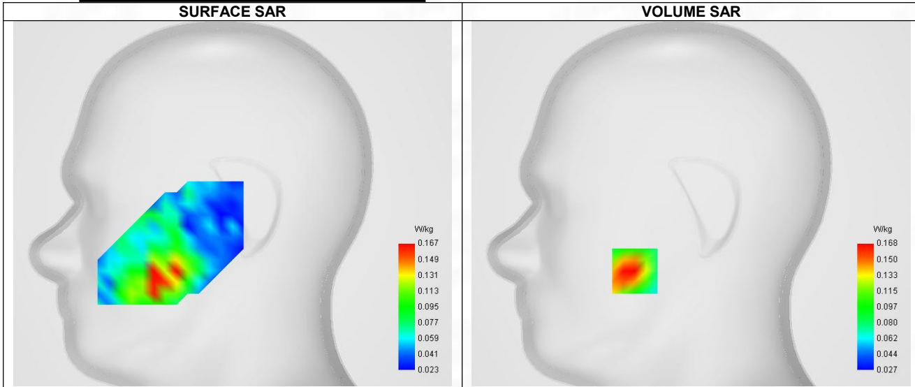
Maximum location: X=-40.00, Y=-48.00 ; SAR Peak: 0.26 W/kg
