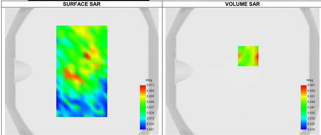
Maximum location: X=9.00, Y=24.00 ; SAR Peak: 0.09 W/kg
