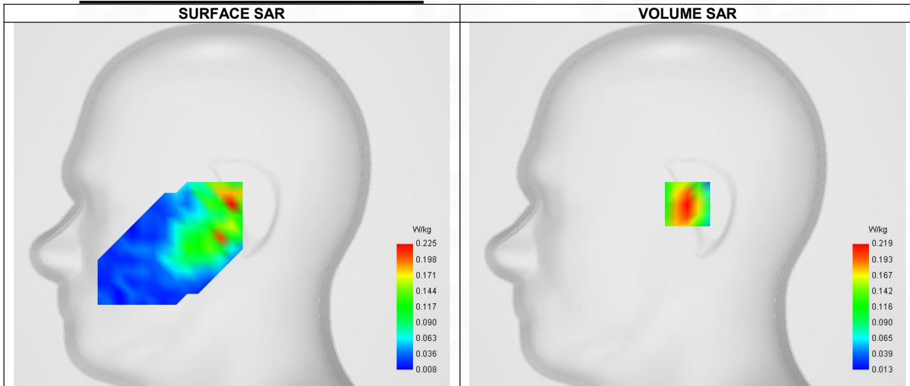
Maximum location: X=0.00, Y=0.00 ; SAR Peak: 0.41 W/kg
