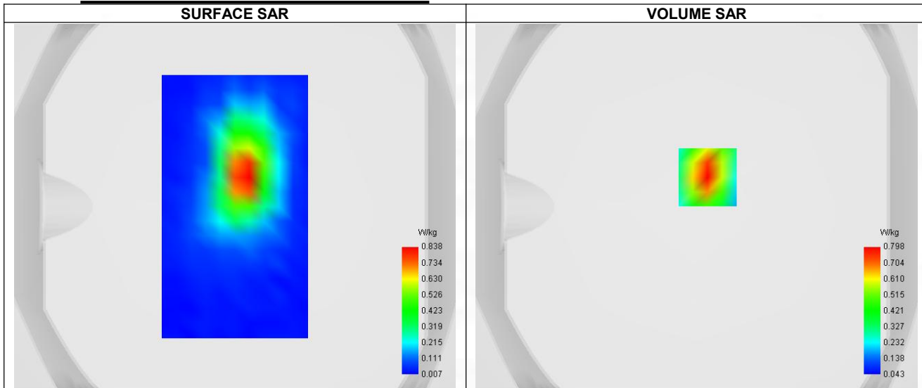
Maximum location: X=6.00, Y=16.00 ; SAR Peak: 1.17 W/kg
