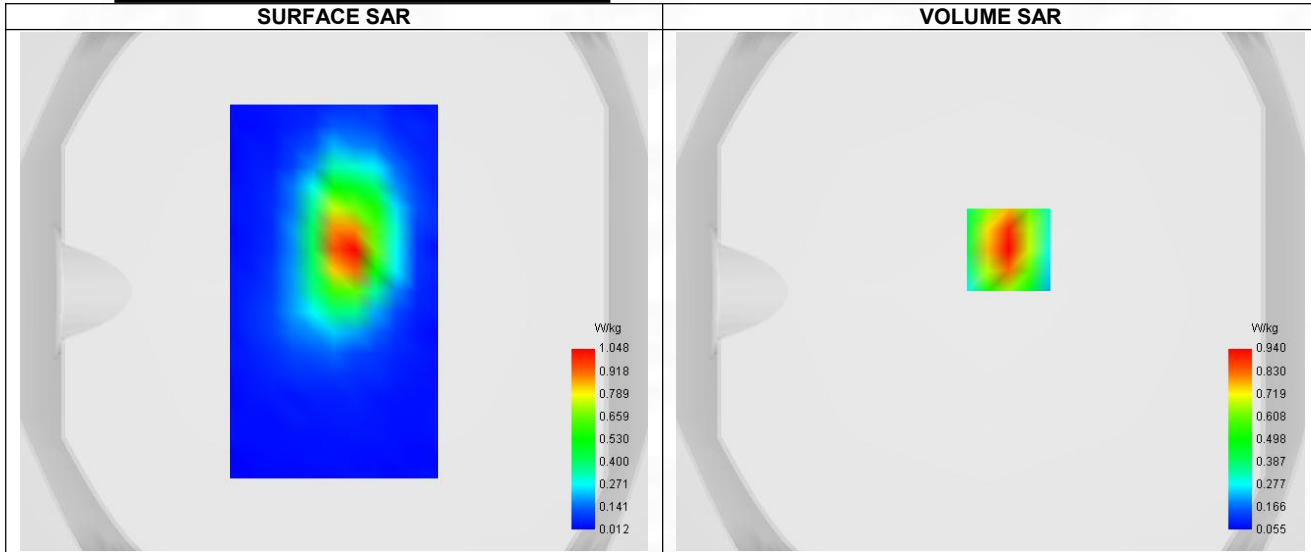
Maximum location: X=7.00, Y=16.00 ; SAR Peak: 1.24 W/kg
