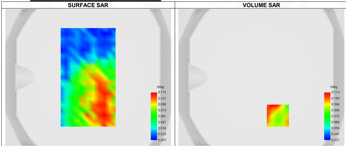
Maximum location: X=24.00, Y=-56.00 ; SAR Peak: 0.16 W/kg
