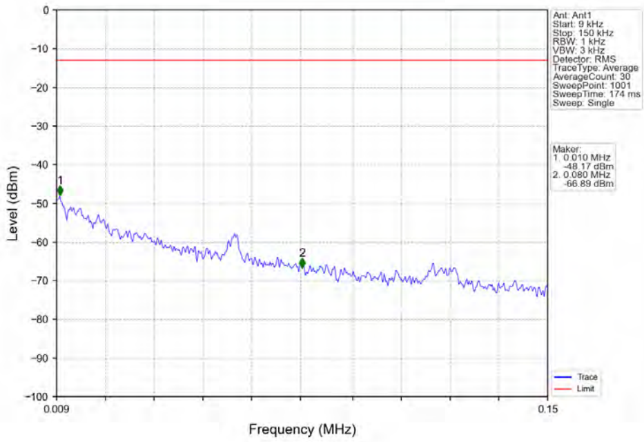
Band66_3MHz_16QAM_MCH_1745MHz_RB_1_0_NTNV
