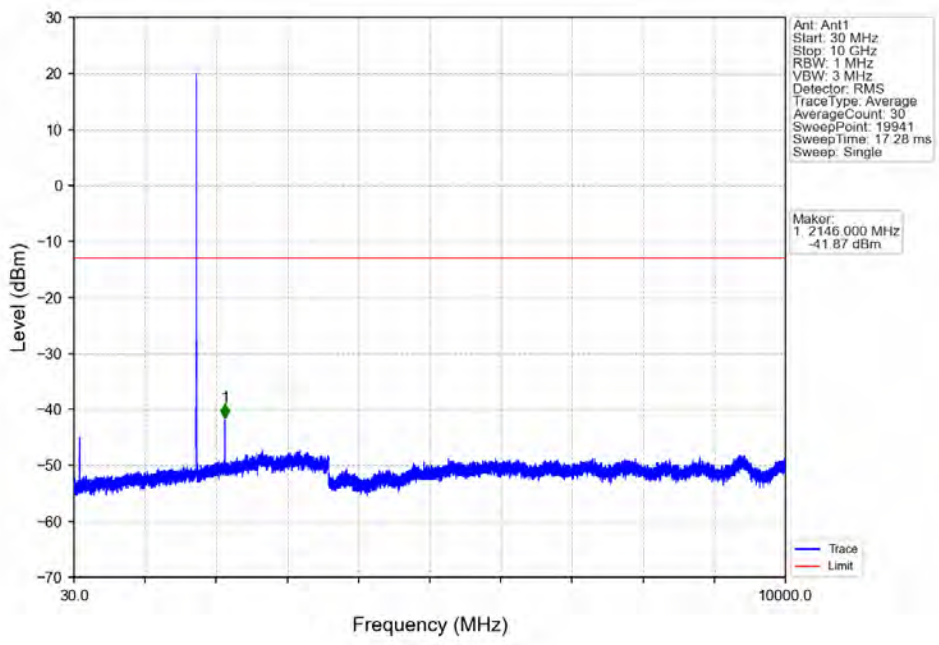
Band66_3MHz_16QAM_MCH_1745MHz_RB_1_0_NTNV
