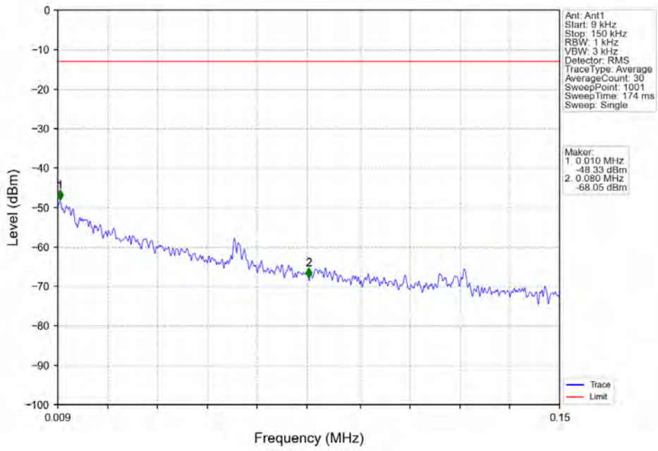
Band66_3MHz_16QAM_LCH_1711.5MHz_RB_1_0_NTNV
