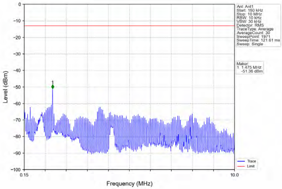
Band66_5MHz_QPSK_LCH_1712.5MHz_RB_1_0_NTNV
