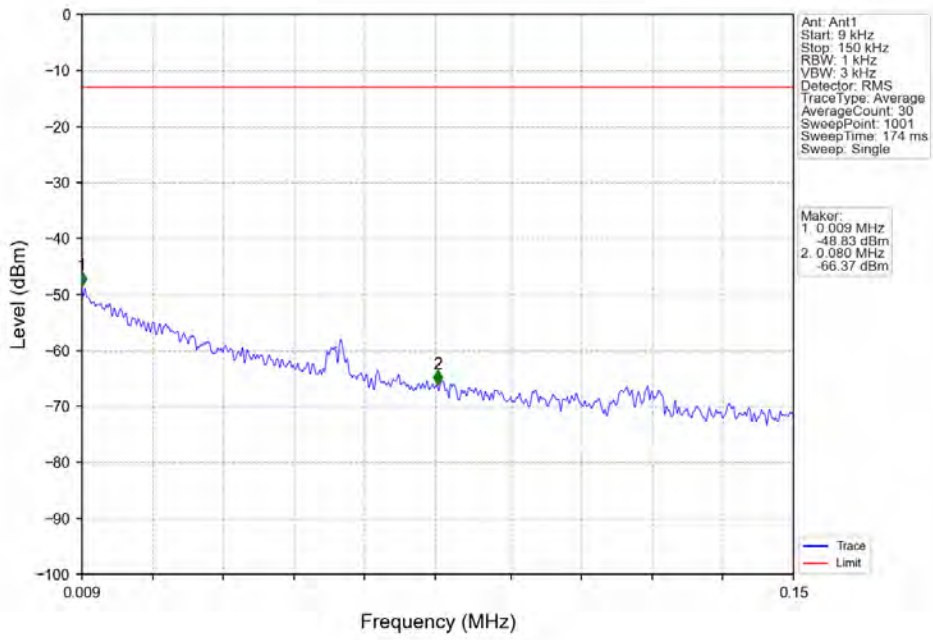
Band66_10MHz_16QAM_LCH_1715MHz_RB_1_0_NTNV
