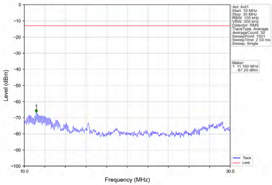
Band66_5MHz_16QAM_MCH_1745MHz_RB_1_0_NTNV
