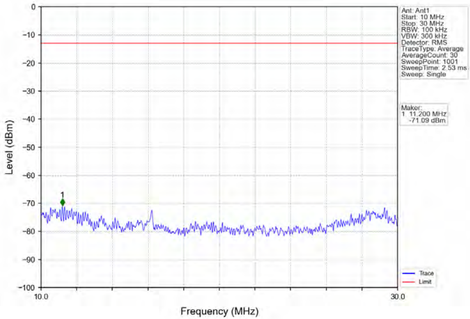
Band66_15MHz_QPSK_LCH_1717.5MHz_RB_1_0_NTV
