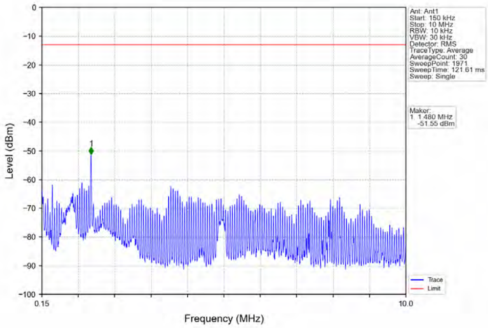
Band66_15MHz_QPSK_LCH_1717.5MHz_RB_1_0_NTV
