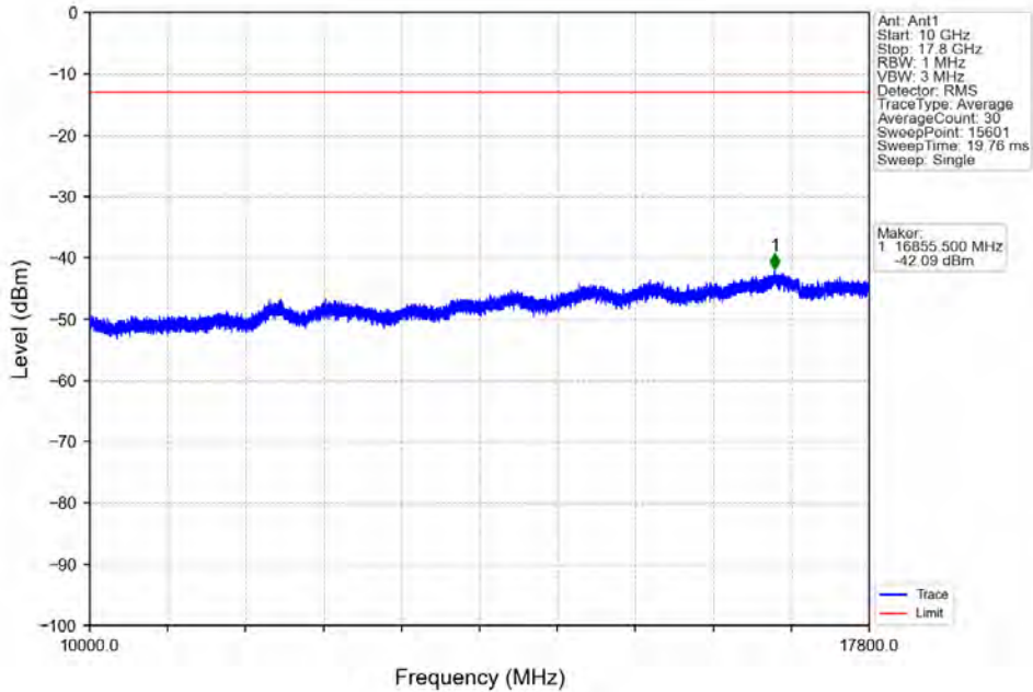
Band66_5MHz_QPSK_LCH_1712.5MHz_RB_1_0_NTNV
