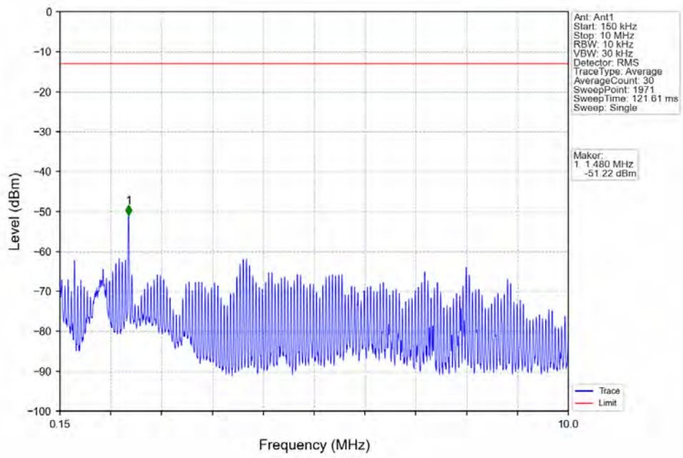
Band66_15MHz_16QAM_HCH_1772.5MHz_RB_1_0_NTNV
