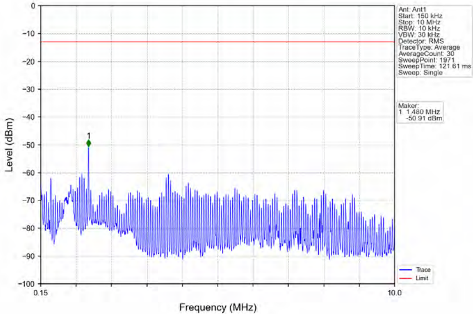
Band66_3MHz_16QAM_MCH_1745MHz_RB_1_0_NTNV
