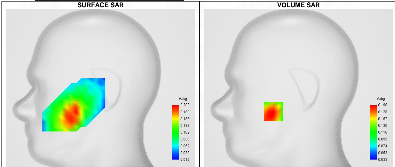
Maximum location: X=-41.00, Y=-39.00 ; SAR Peak: 0.25 W/kg
