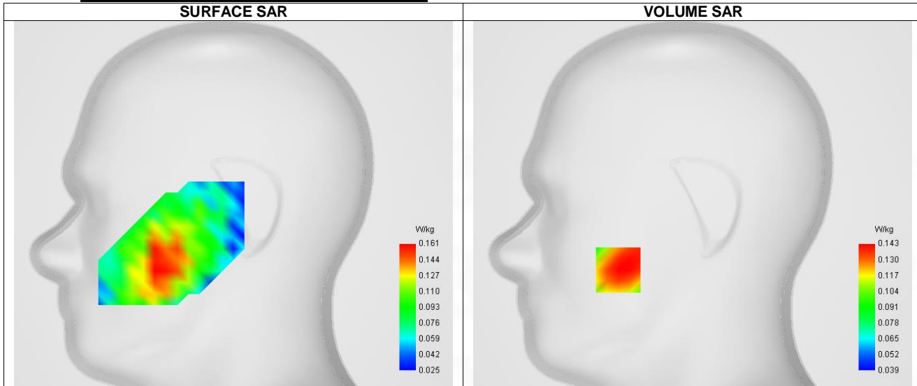
Maximum location: X=-53.00, Y=-47.00 ; SAR Peak: 0.17 W/kg
