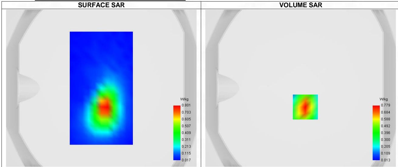
Maximum location: X=6.00, Y=-24.00 ; SAR Peak: 1.26 W/kg
