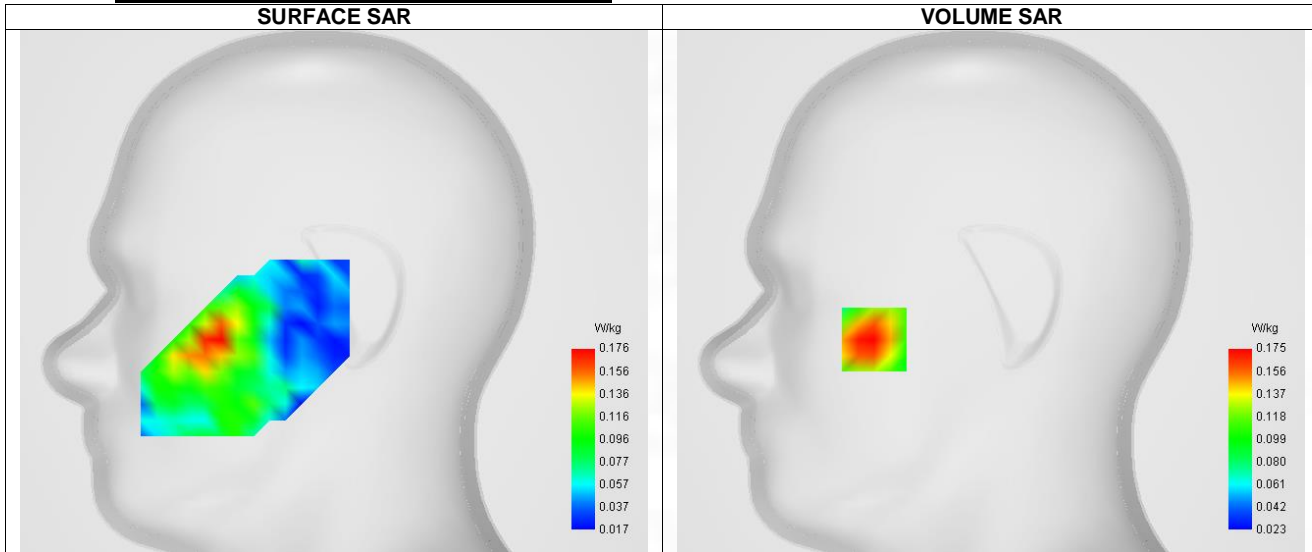
Maximum location: X=-58.00, Y=-24.00 ; SAR Peak: 0.23 W/kg
