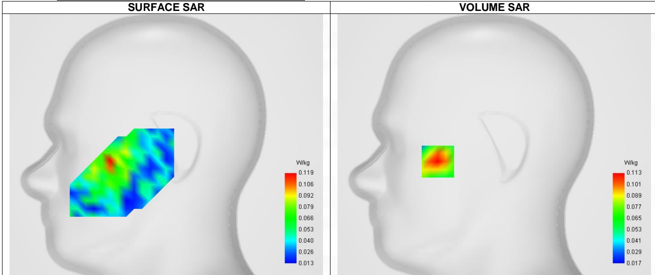
Maximum location: X=-56.00, Y=-17.00 ; SAR Peak: 0.22 W/kg
