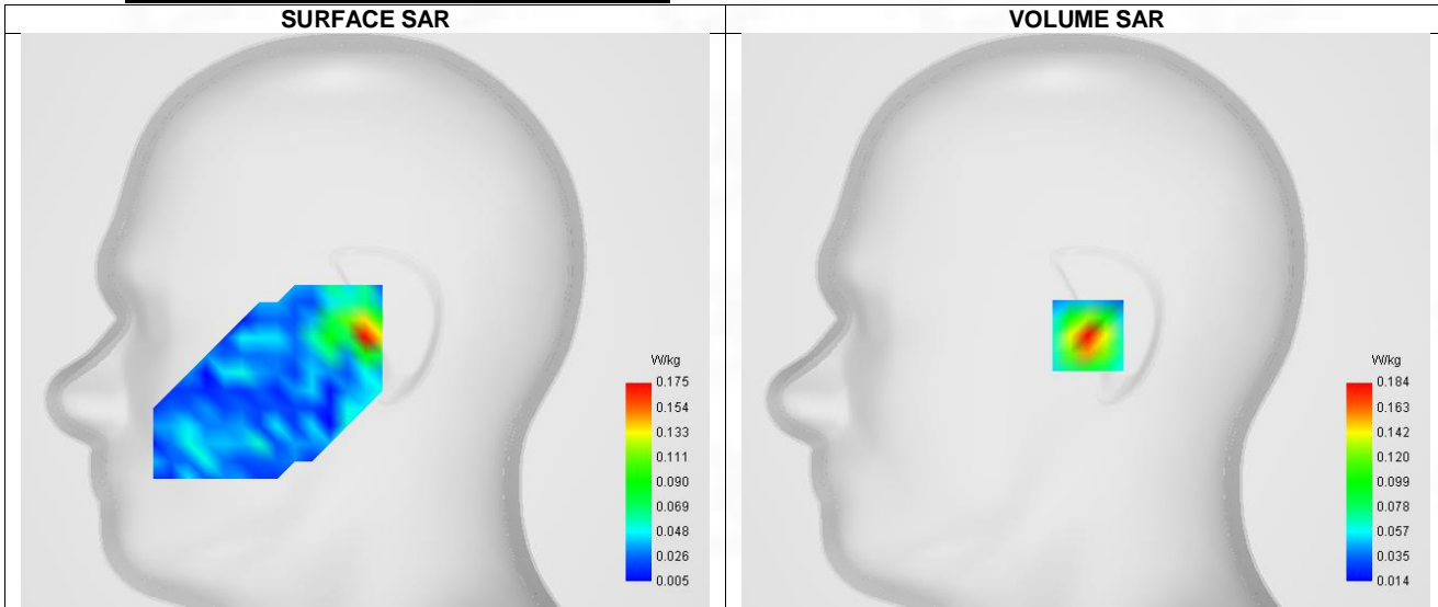
Maximum location: X=1.00, Y=-7.00 ; SAR Peak: 0.34 W/kg
