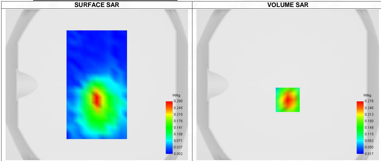
Maximum location: X=0.00, Y=-20.00 ; SAR Peak: 0.45 W/kg
