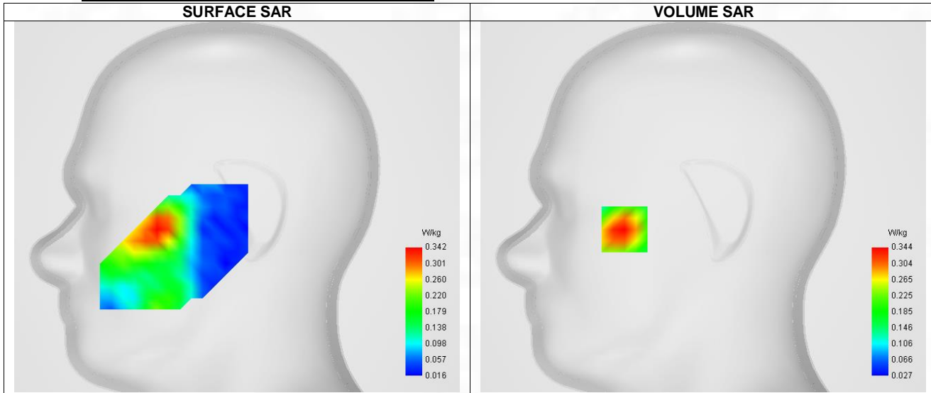
Maximum location: X=-55.00, Y=-16.00 ; SAR Peak: 0.49 W/kg
