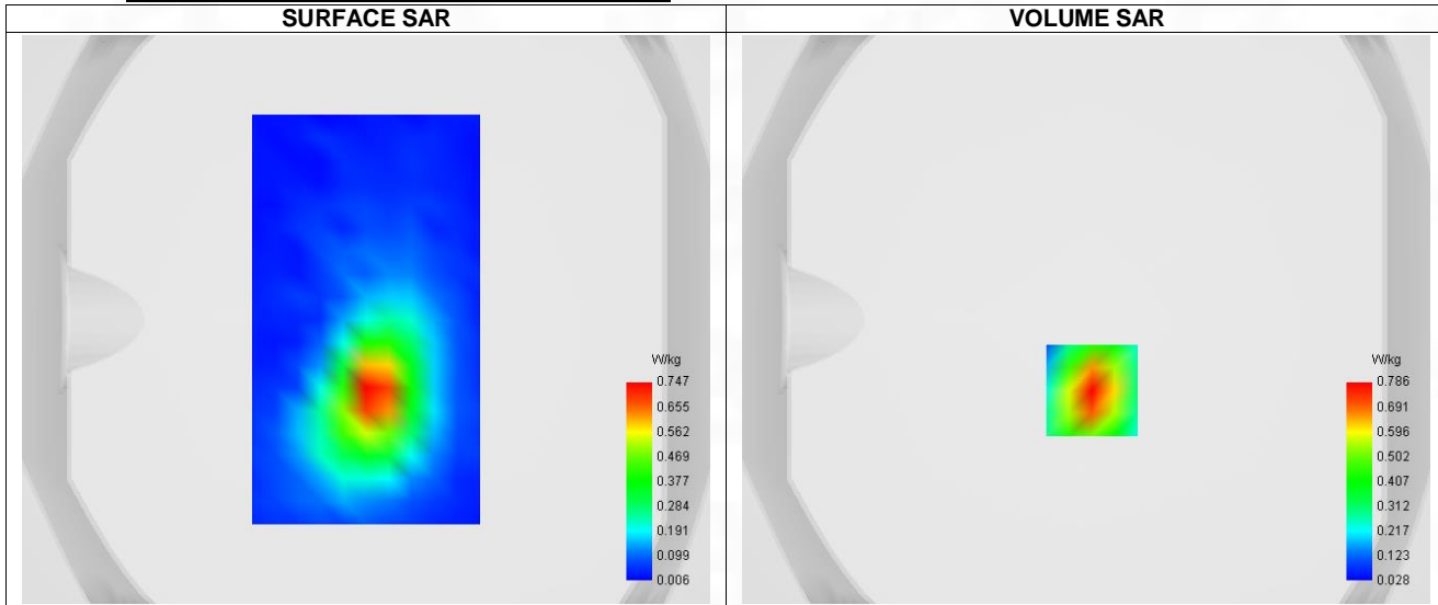
Maximum location: X=2.00, Y=-25.00 ; SAR Peak: 1.32 W/kg
