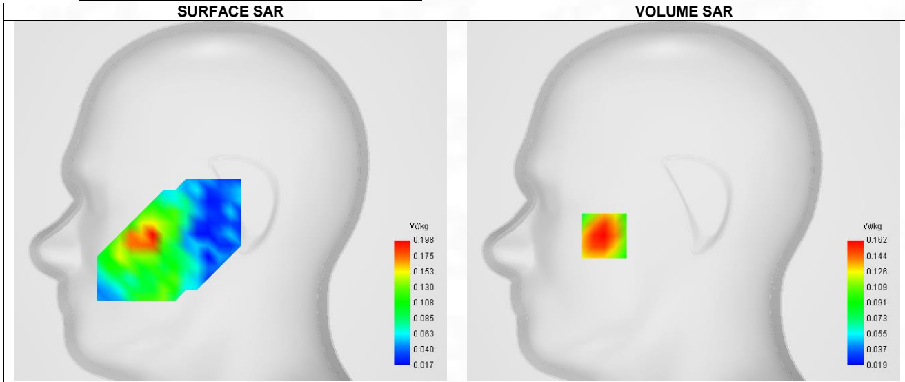
Maximum location: X=-57.00, Y=-25.00 ; SAR Peak: 0.18 W/kg
