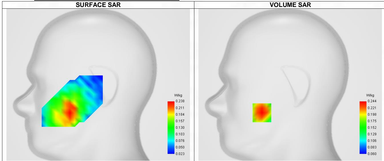
Maximum location: X=-48.00, Y=-48.00 ; SAR Peak: 0.30 W/kg
