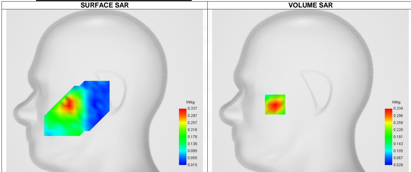
Maximum location: X=-56.00, Y=-22.00 ; SAR Peak: 0.49 W/kg
