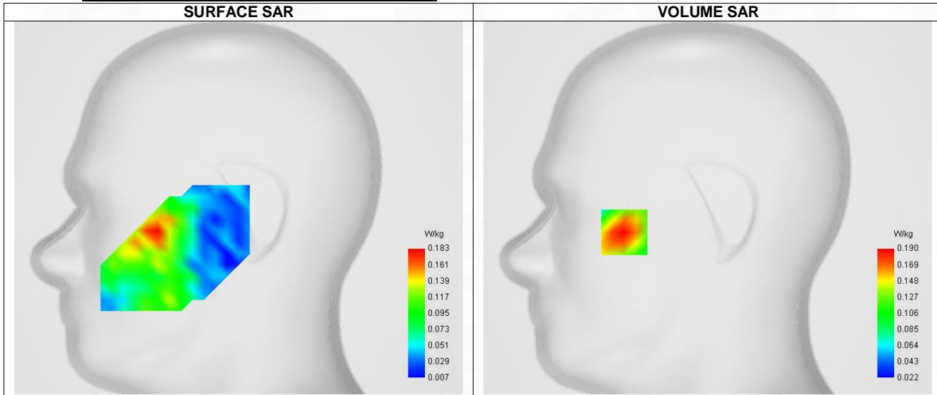
Maximum location: X=-58.00, Y=-17.00 ; SAR Peak: 0.29 W/kg
