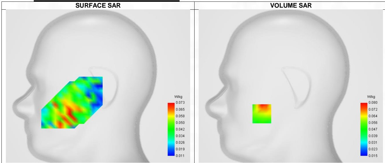
Maximum location: X=-49.00, Y=-47.00 ; SAR Peak: 0.18 W/kg
