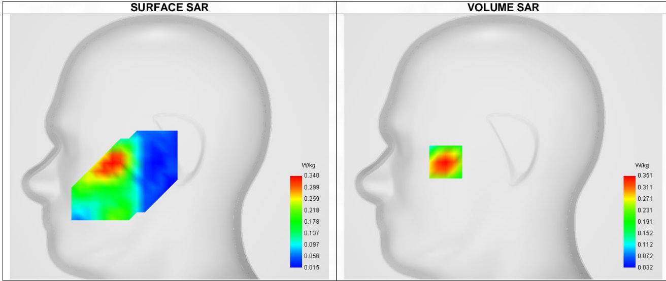
Maximum location: X=-56.00, Y=-15.00 ; SAR Peak: 0.50 W/kg
