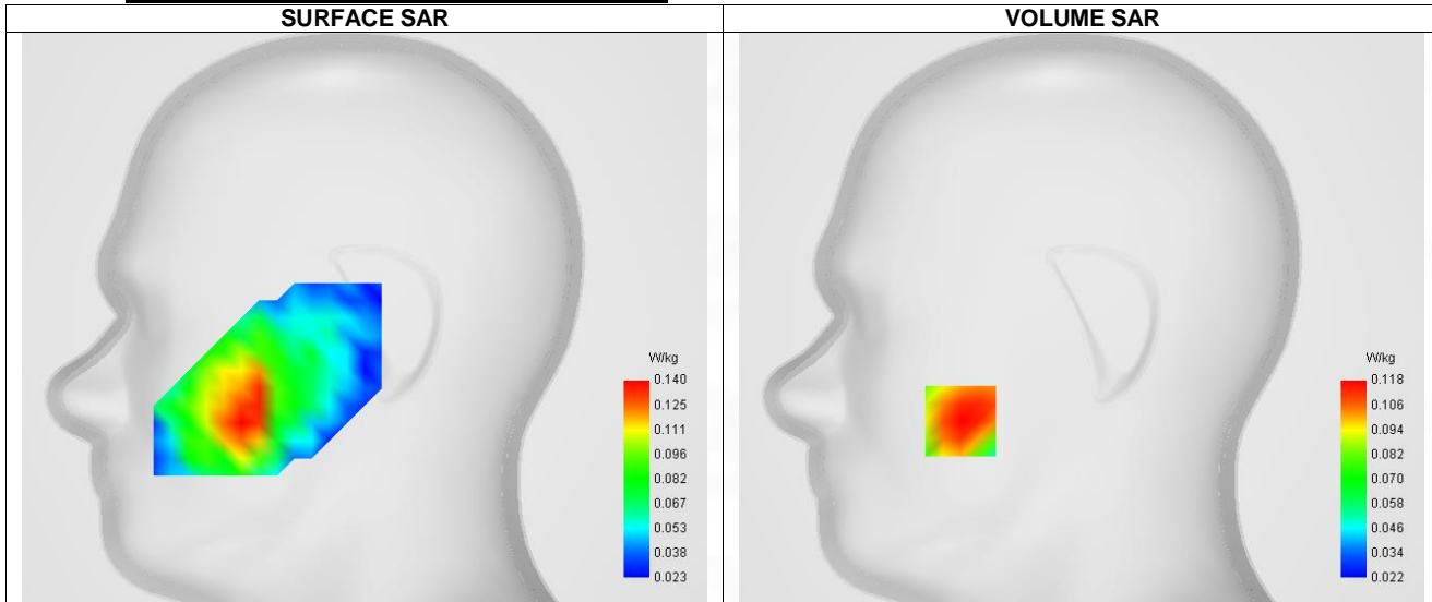
Maximum location: X=-55.00, Y=-47.00 ; SAR Peak: 0.16 W/kg
