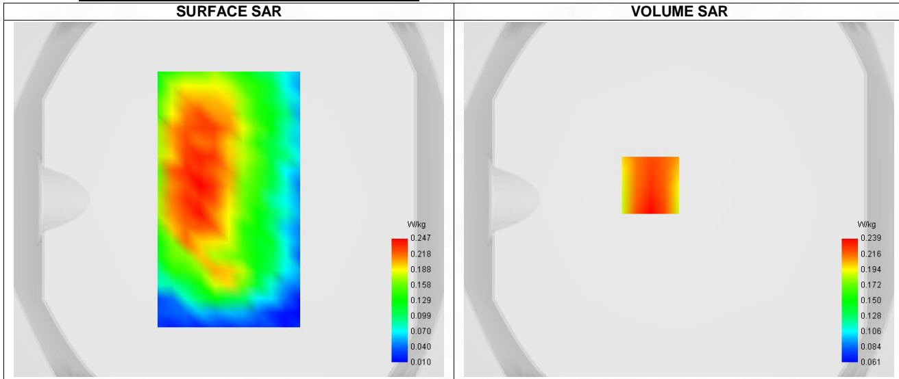
Maximum location: X=-16.00, Y=8.00 ; SAR Peak: 0.30 W/kg
