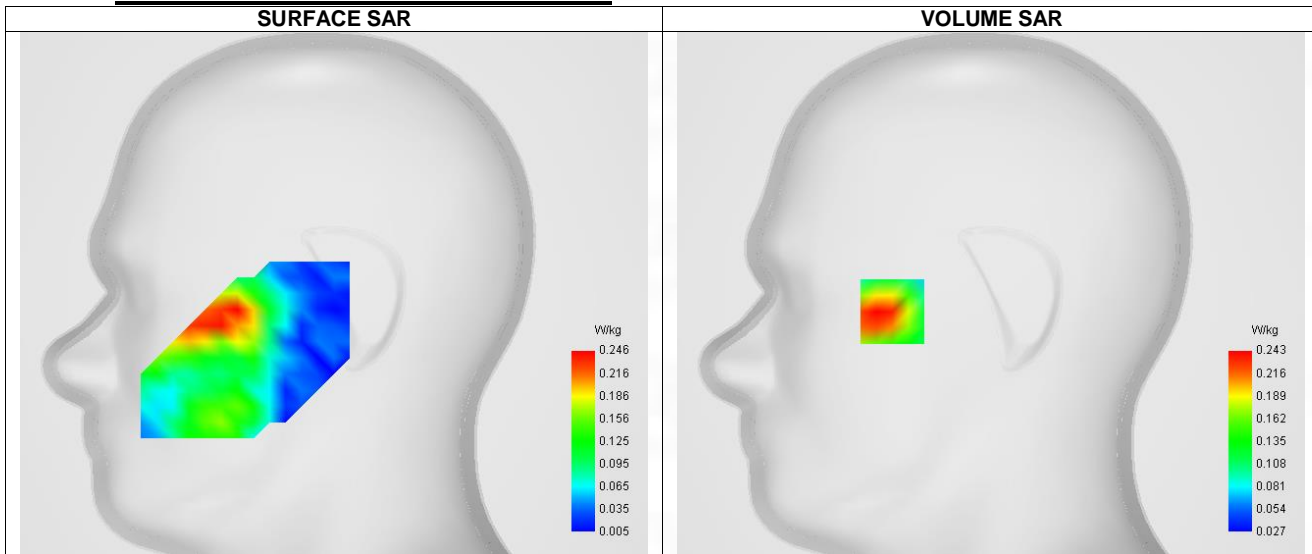
Maximum location: X=-49.00, Y=-9.00 ; SAR Peak: 0.36 W/kg
