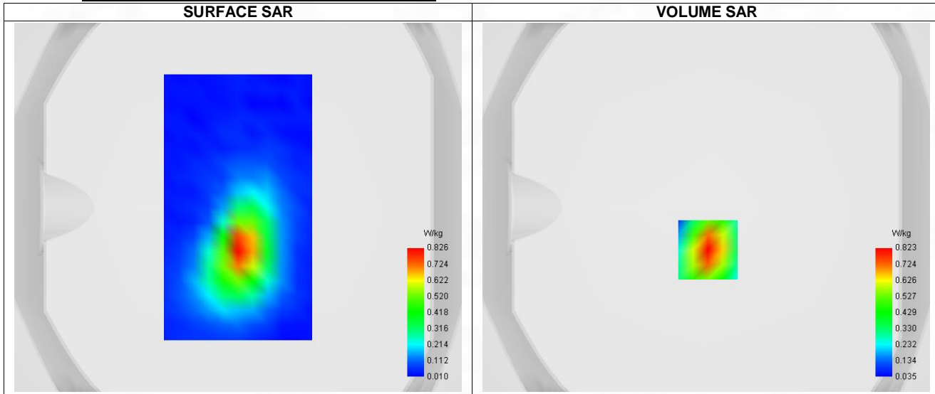
Maximum location: X=1.00, Y=-23.00 ; SAR Peak: 1.29 W/kg
