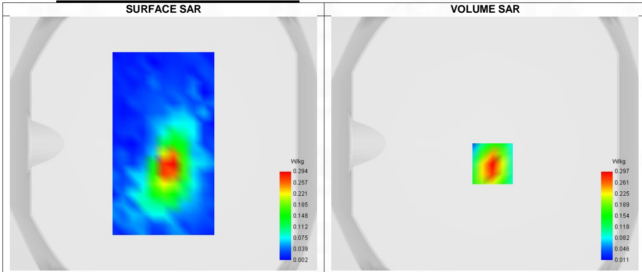
Maximum location: X=6.00, Y=-16.00 ; SAR Peak: 0.47 W/kg
