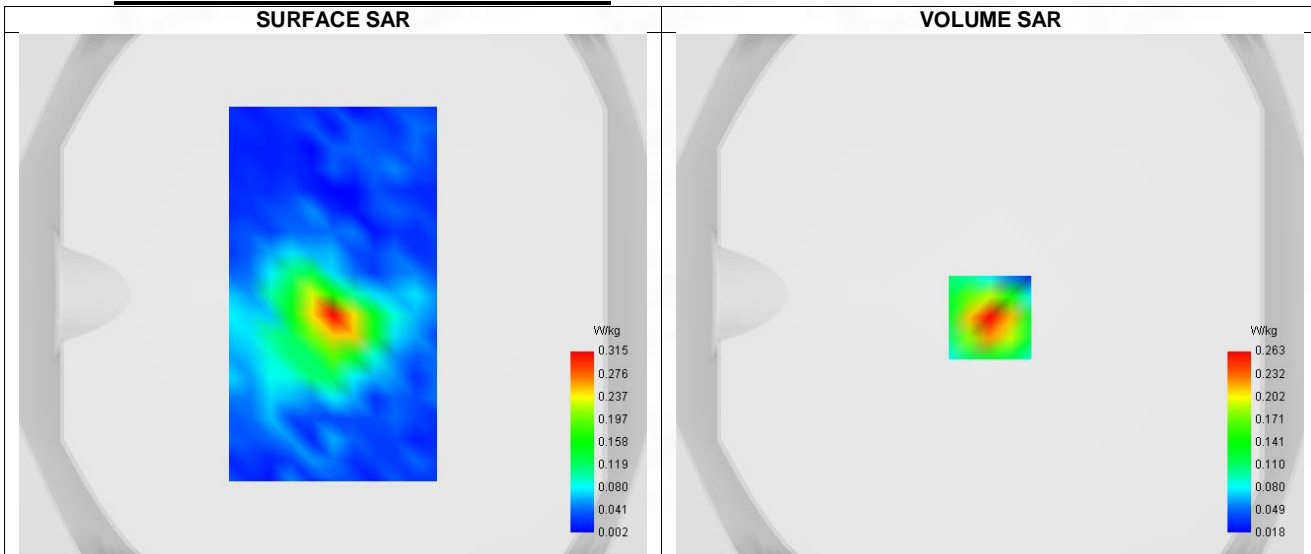
Maximum location: X=0.00, Y=-9.00 ; SAR Peak: 0.48 W/kg
