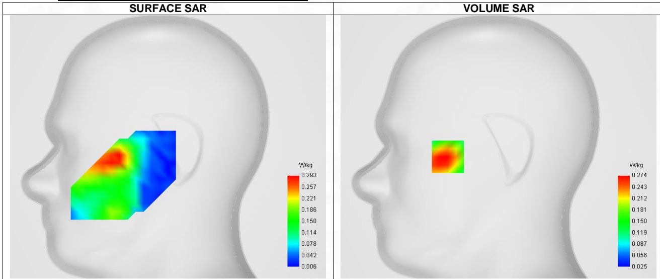
Maximum location: X=-50.00, Y=-10.00 ; SAR Peak: 0.39 W/kg
