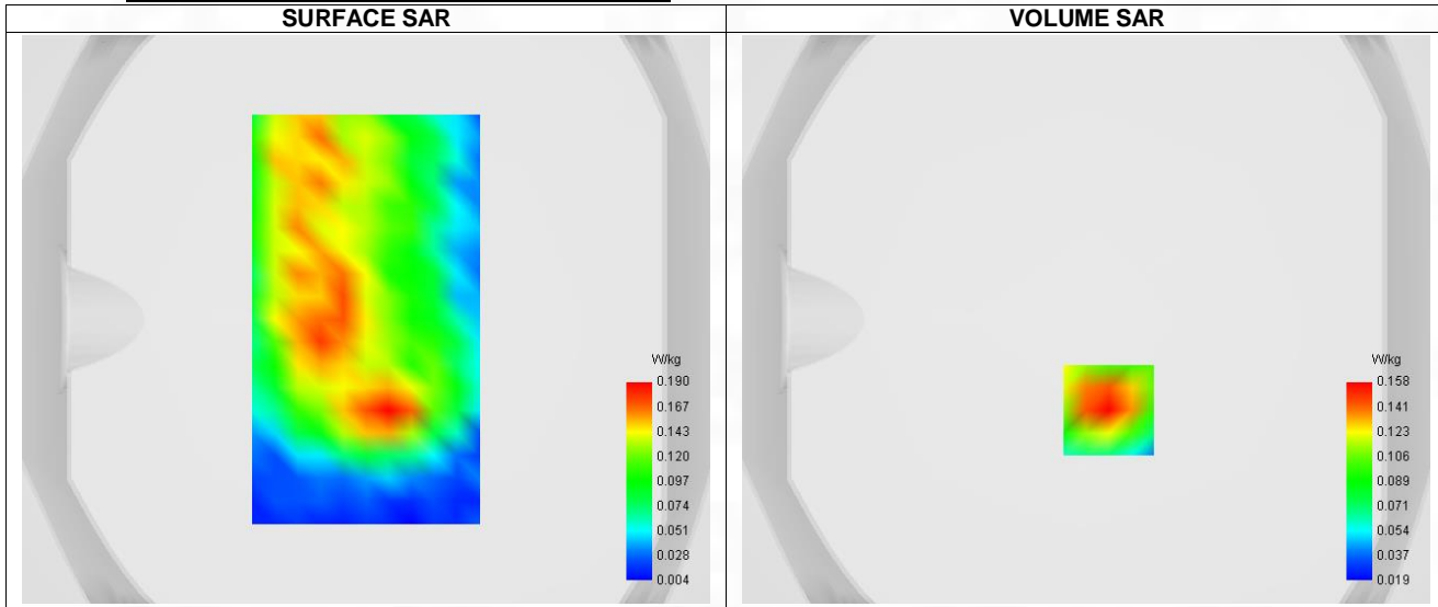
Maximum location: X=8.00, Y=-32.00 ; SAR Peak: 0.24 W/kg
