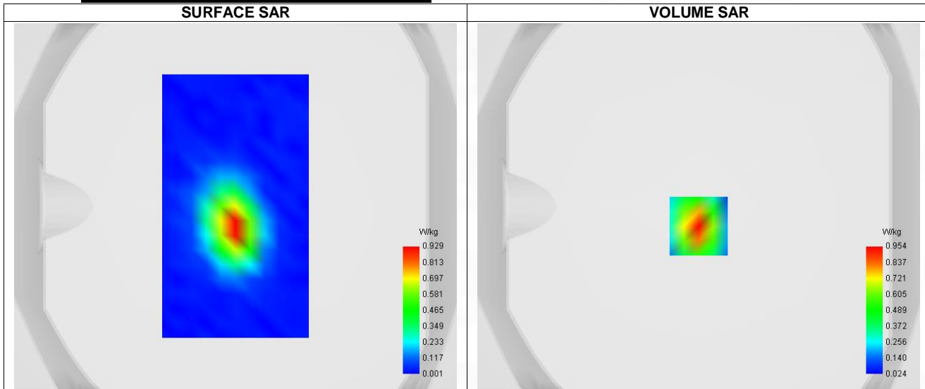
Maximum location: X=0.00, Y=-11.00 ; SAR Peak: 1.55 W/kg
