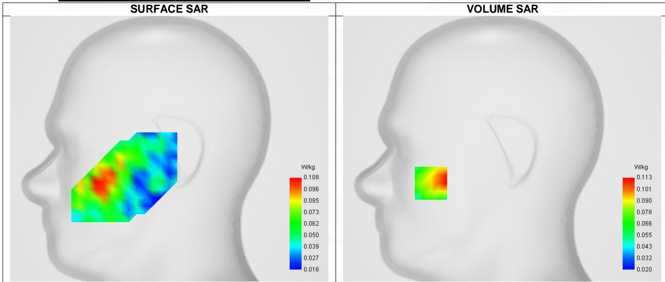
Maximum location: X=-70.00, Y=-34.00 ; SAR Peak: 0.18 W/kg
