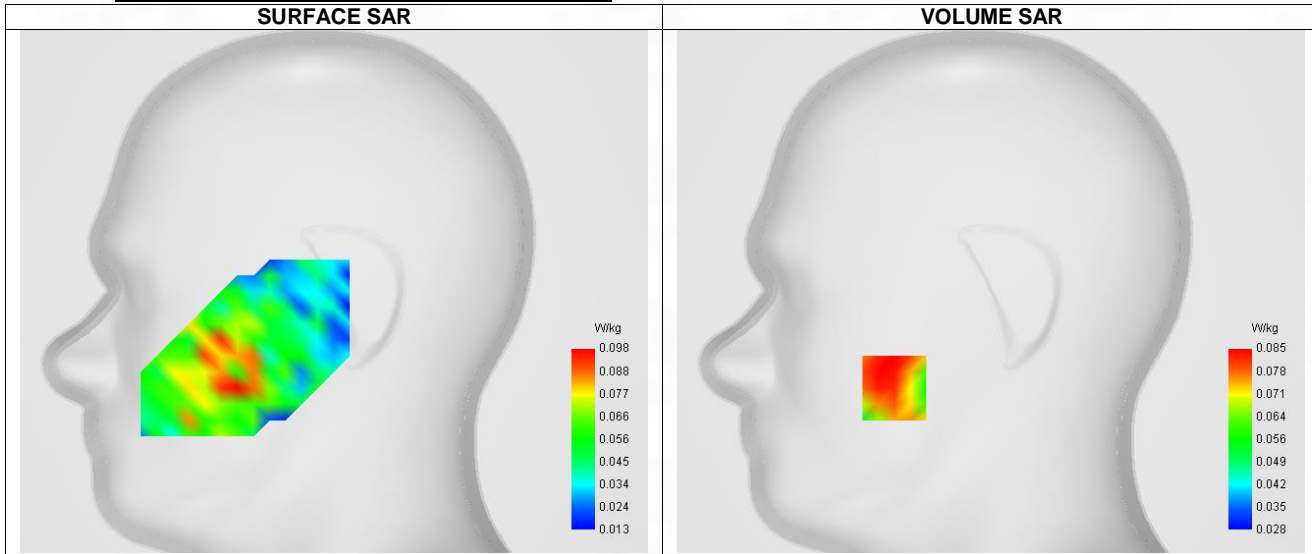
Maximum location: X=-48.00, Y=-48.00 ; SAR Peak: 0.12 W/kg
