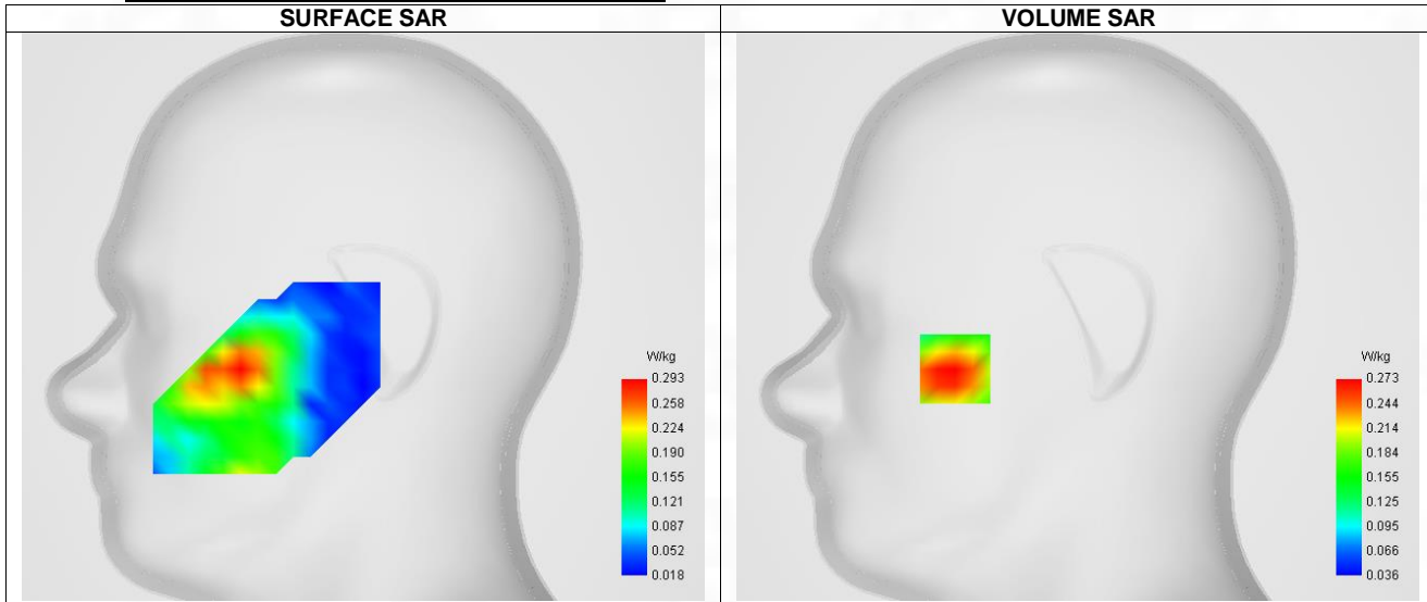
Maximum location: X=-56.00, Y=-24.00 ; SAR Peak: 0.38 W/kg
