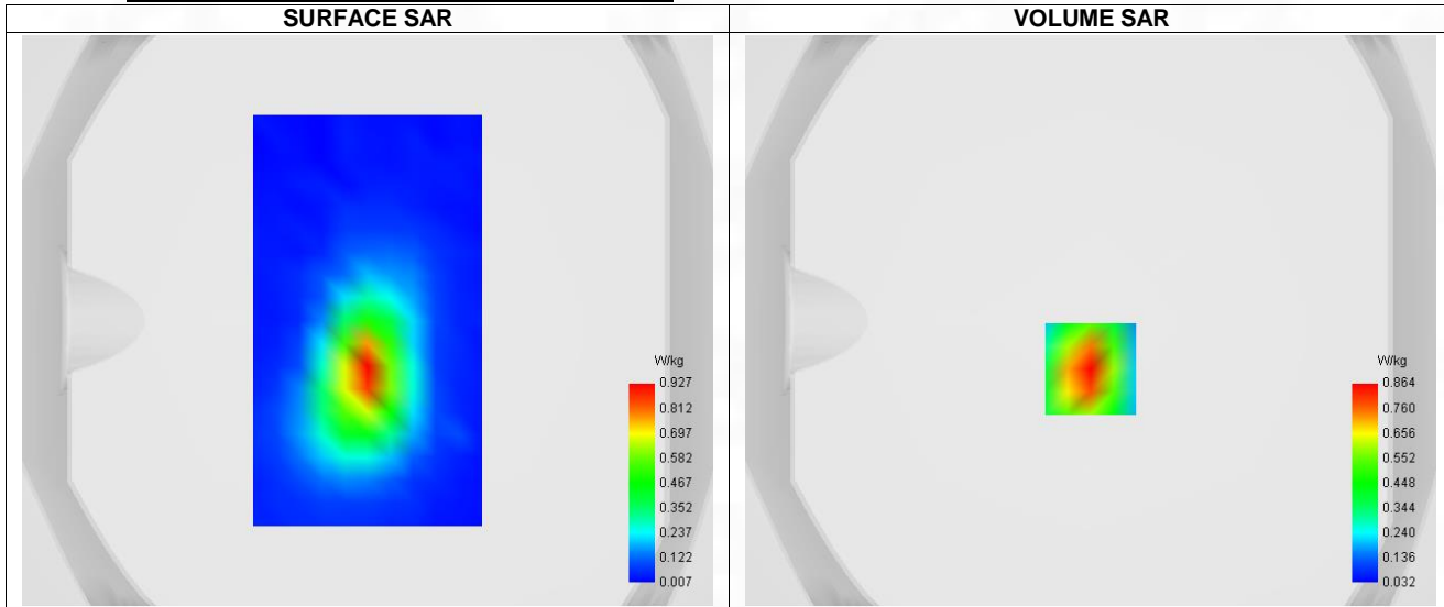
Maximum location: X=0.00, Y=-17.00 ; SAR Peak: 1.35 W/kg
