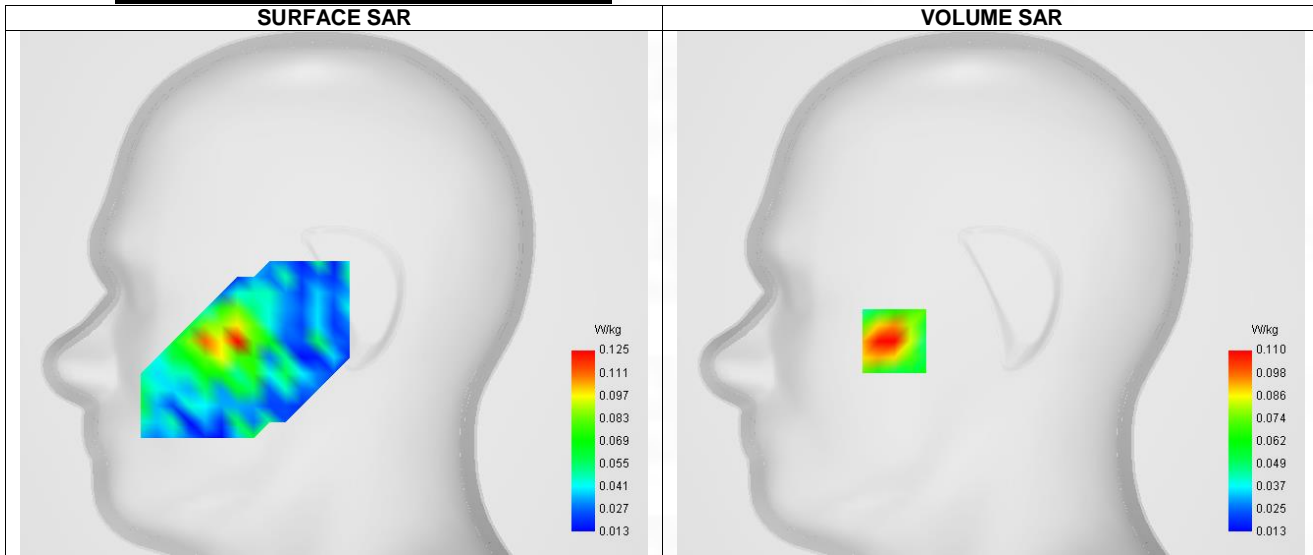
Maximum location: X=-48.00, Y=-24.00 ; SAR Peak: 0.15 W/kg
