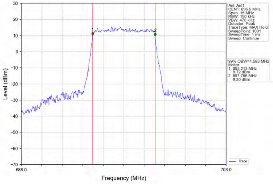
Band71_5MHz_16QAM_HCH_695.5MHz_RB_25_0_NTNV
