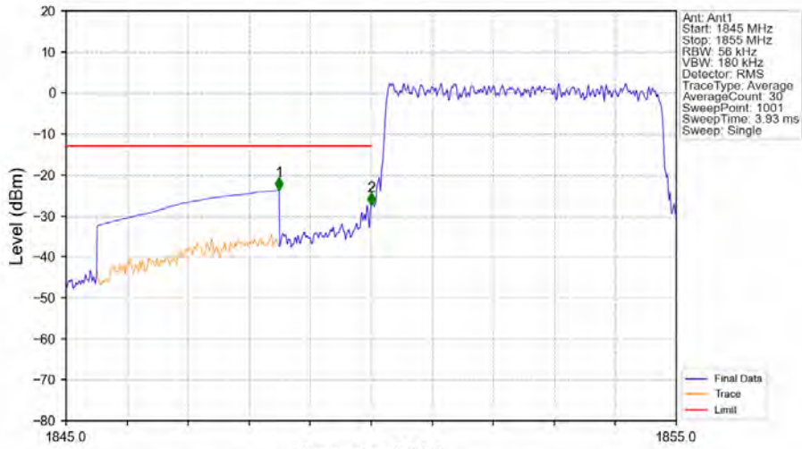
Band25_5MHz_16QAM_LCH_1852.5MHz_RB_25_0_NTNV
