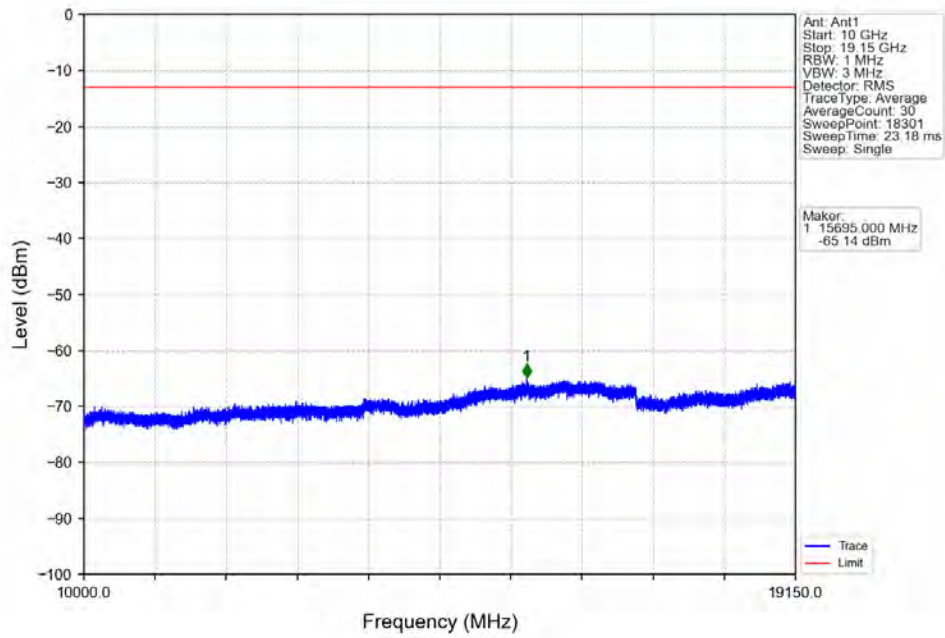
Band25_20MHz_16QAM_LCH_1860MHz_RB_100_0_NTNV
