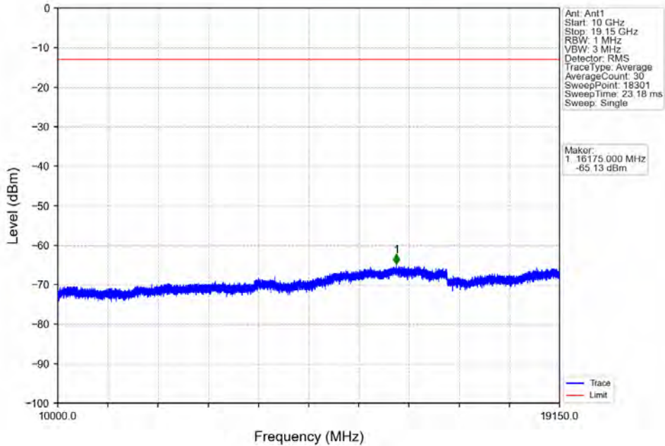
Band25_5MHz_QPSK_MCH_1882.5MHz_RB_1_0_NTNV
