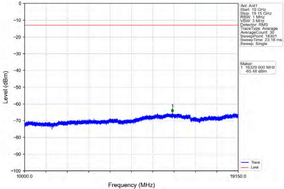
Band25_15MHz_16QAM_MCH_1882.5MHz_RB_1_0_NTNV
