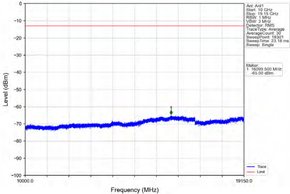
Band25_5MHz_16QAM_MCH_1882.5MHz_RB_1_0_NTNV
