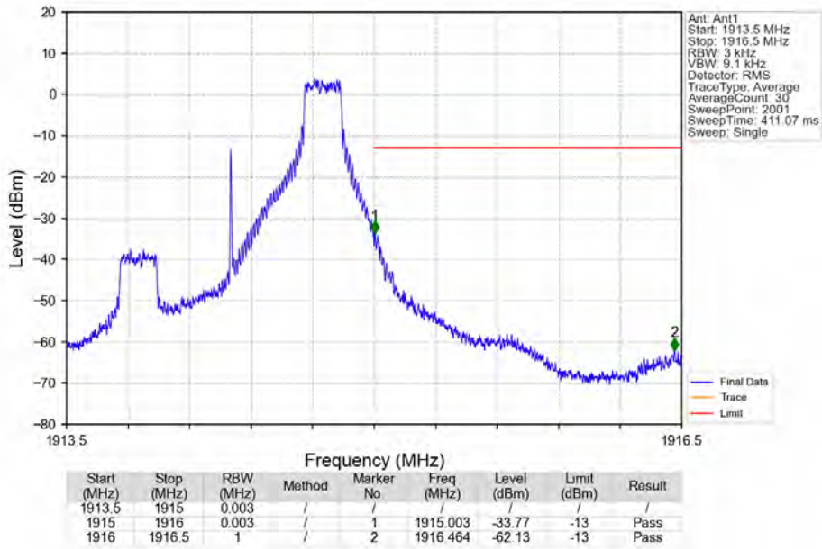
Band25_1.4MHz_16QAM_HCH_1914.3MHz_RB_1_5_NTNV
