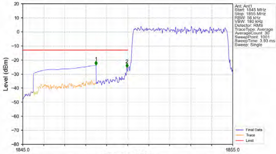
Band25_5MHz_QPSK_LCH_1852.5MHz_RB_25_0_NTNV
