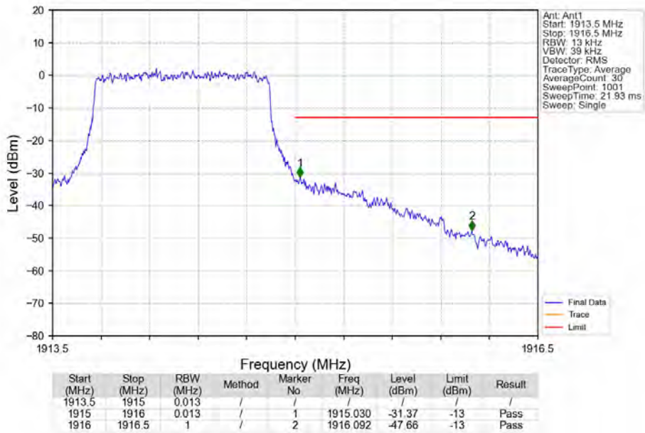
Band25_1.4MHz_16QAM_HCH_1914.3MHz_RB_6_0_NTNV
