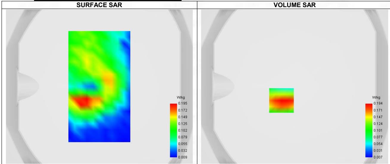
Maximum location: X=-17.00, Y=-18.00 ; SAR Peak: 0.30 W/kg
