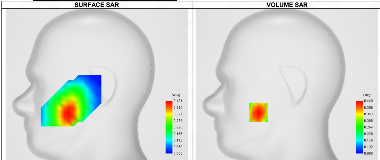
Maximum location: X=-49.00, Y=-48.00 ; SAR Peak: 0.50 W/kg
