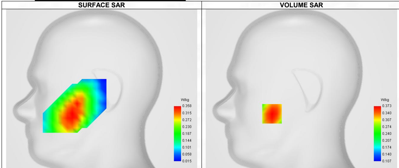
Maximum location: X=-48.00, Y=-41.00 ; SAR Peak: 0.48 W/kg
