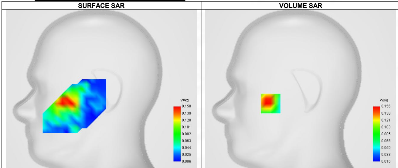
Maximum location: X=-49.00, Y=-24.00 ; SAR Peak: 0.24 W/kg
