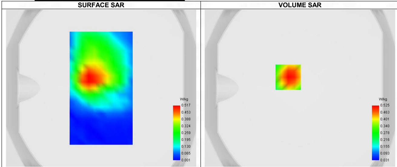
Maximum location: X=-15.00, Y=14.00 ; SAR Peak: 0.70 W/kg
