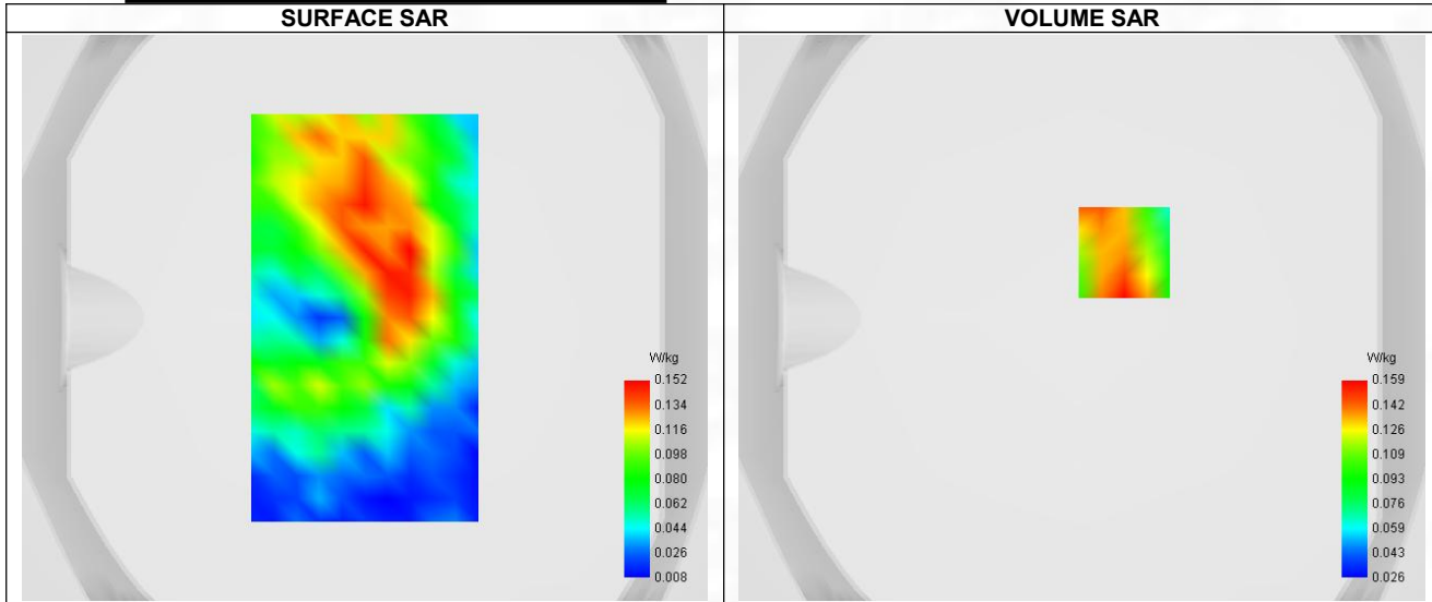
Maximum location: X=15.00, Y=23.00 ; SAR Peak: 0.22 W/kg
