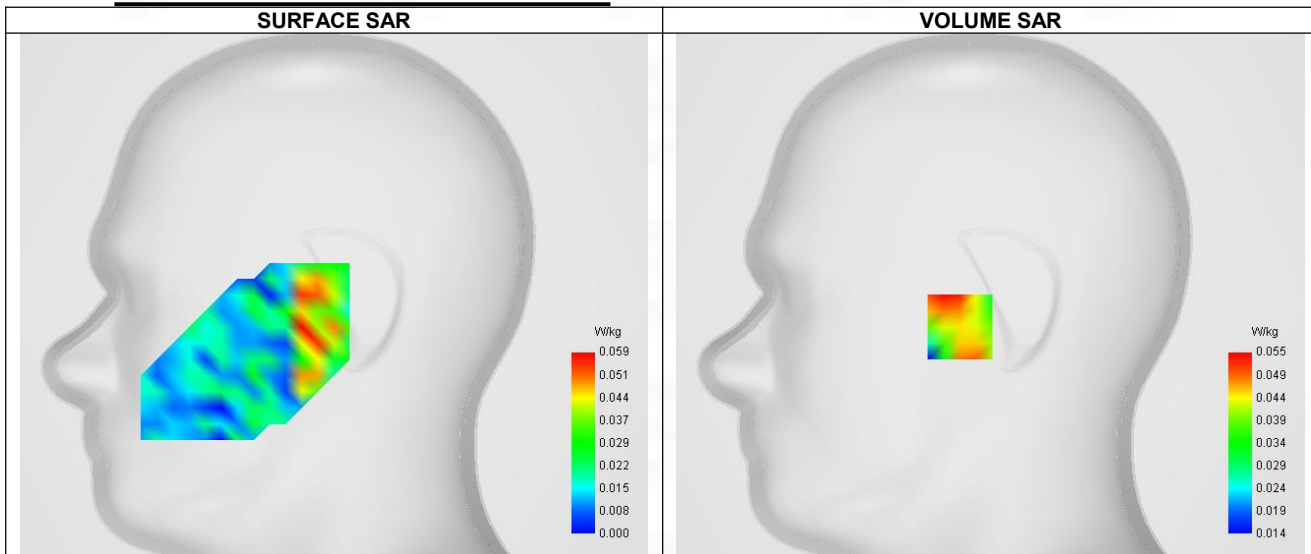
Maximum location: X=-15.00, Y=-16.00 ; SAR Peak: 0.08 W/kg
