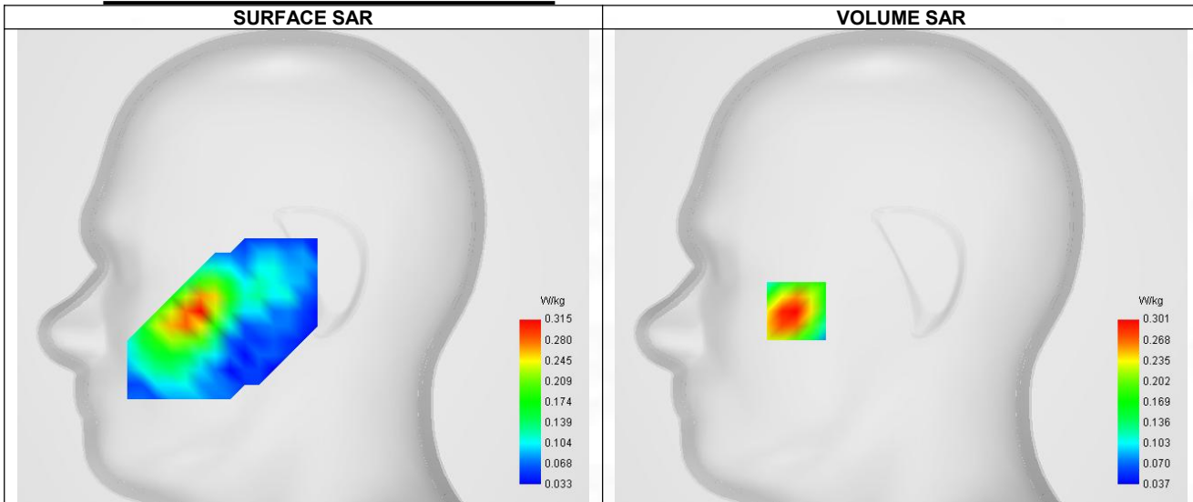
Maximum location: X=-57.00, Y=-24.00 ; SAR Peak: 0.41 W/kg
