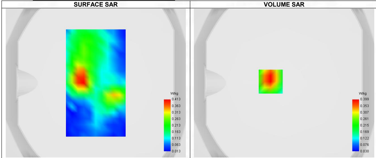
Maximum location: X=-18.00, Y=2.00 ; SAR Peak: 0.56 W/kg
