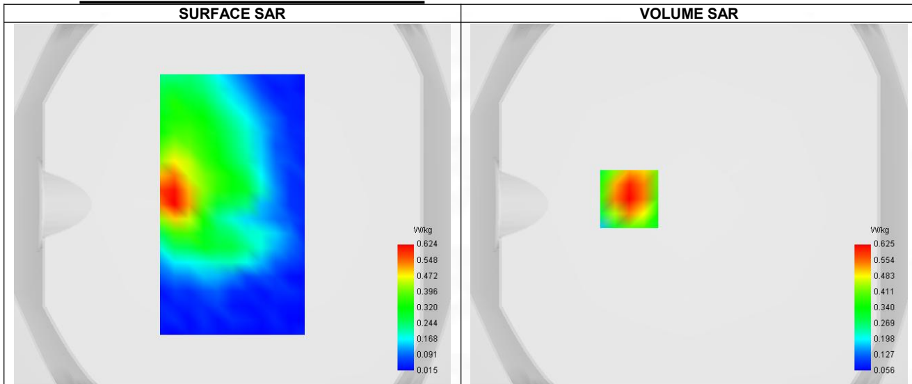
Maximum location: X=-33.00, Y=3.00 ; SAR Peak: 0.86 W/kg
