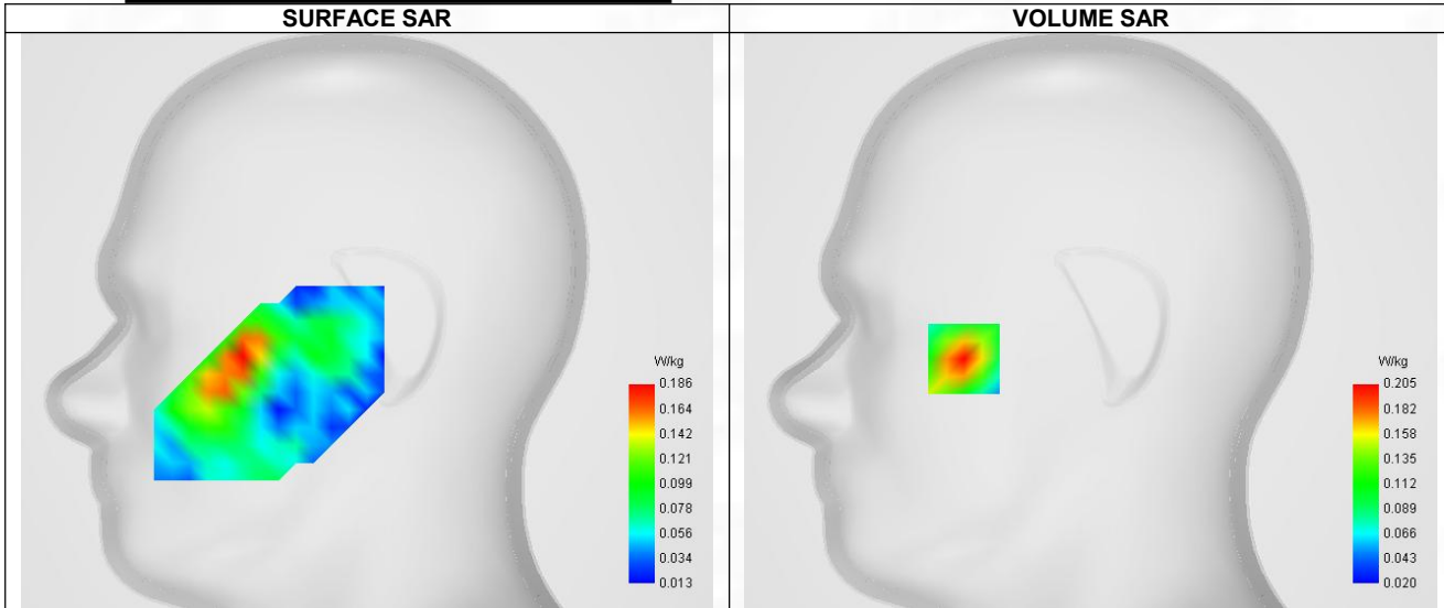
Maximum location: X=-57.00, Y=-17.00 ; SAR Peak: 0.34 W/kg
