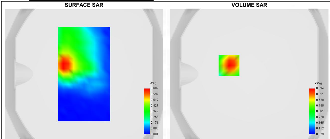
Maximum location: X=-31.00, Y=13.00 ; SAR Peak: 1.02 W/kg
