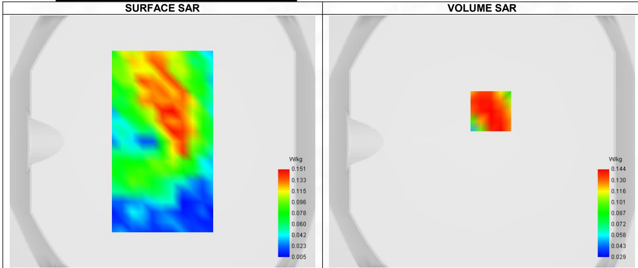
Maximum location: X=7.00, Y=24.00 ; SAR Peak: 0.20 W/kg
