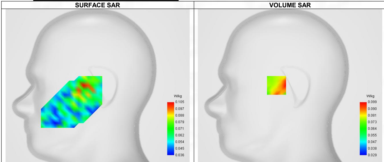
Maximum location: X=-23.00, Y=0.00 ; SAR Peak: 0.13 W/kg
