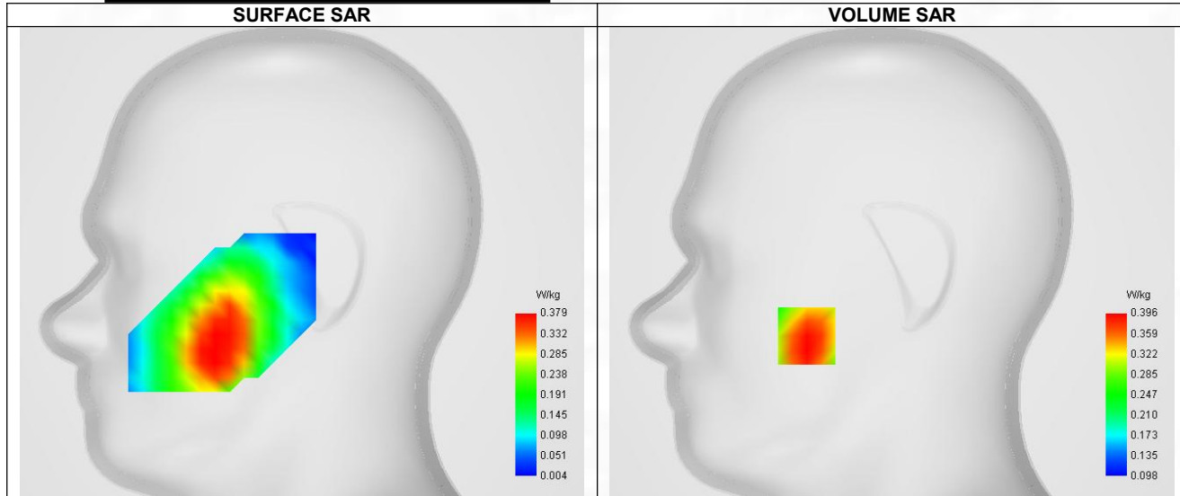
Maximum location: X=-47.00, Y=-41.00 ; SAR Peak: 0.47 W/kg
