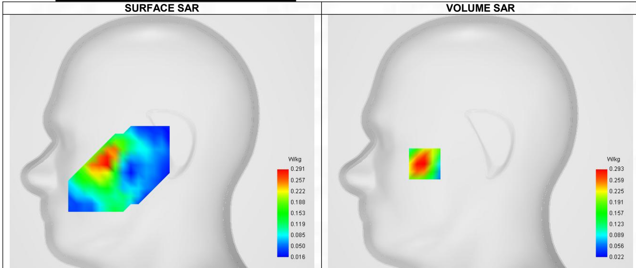
Maximum location: X=-57.00, Y=-23.00 ; SAR Peak: 0.42 W/kg
