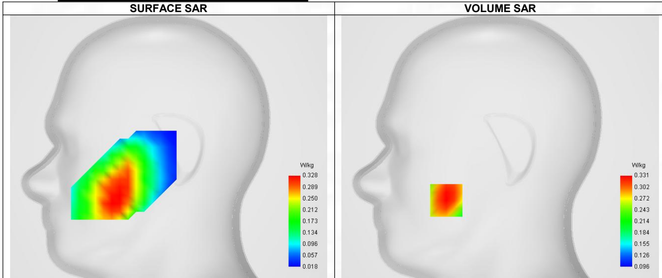
Maximum location: X=-53.00, Y=-53.00 ; SAR Peak: 0.39 W/kg
