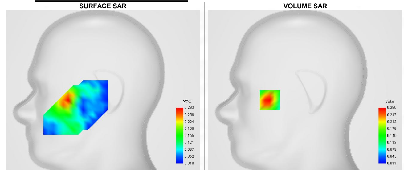
Maximum location: X=-57.00, Y=-16.00 ; SAR Peak: 0.42 W/kg
