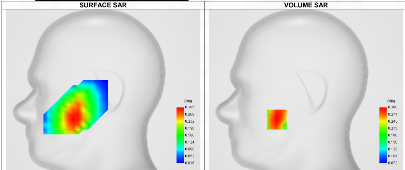
Maximum location: X=-47.00, Y=-48.00 ; SAR Peak: 0.38 W/kg
