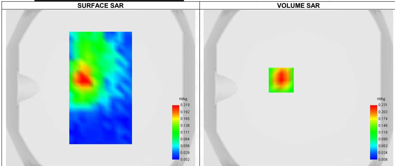
Maximum location: X=-22.00, Y=10.00 ; SAR Peak: 0.38 W/kg
