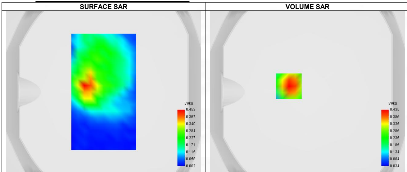
Maximum location: X=-23.00, Y=7.00 ; SAR Peak: 0.60 W/kg
