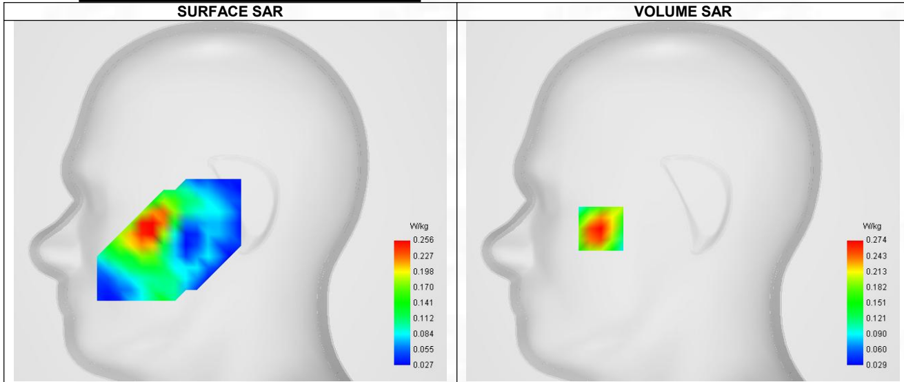
Maximum location: X=-59.00, Y=-20.00 ; SAR Peak: 0.38 W/kg
