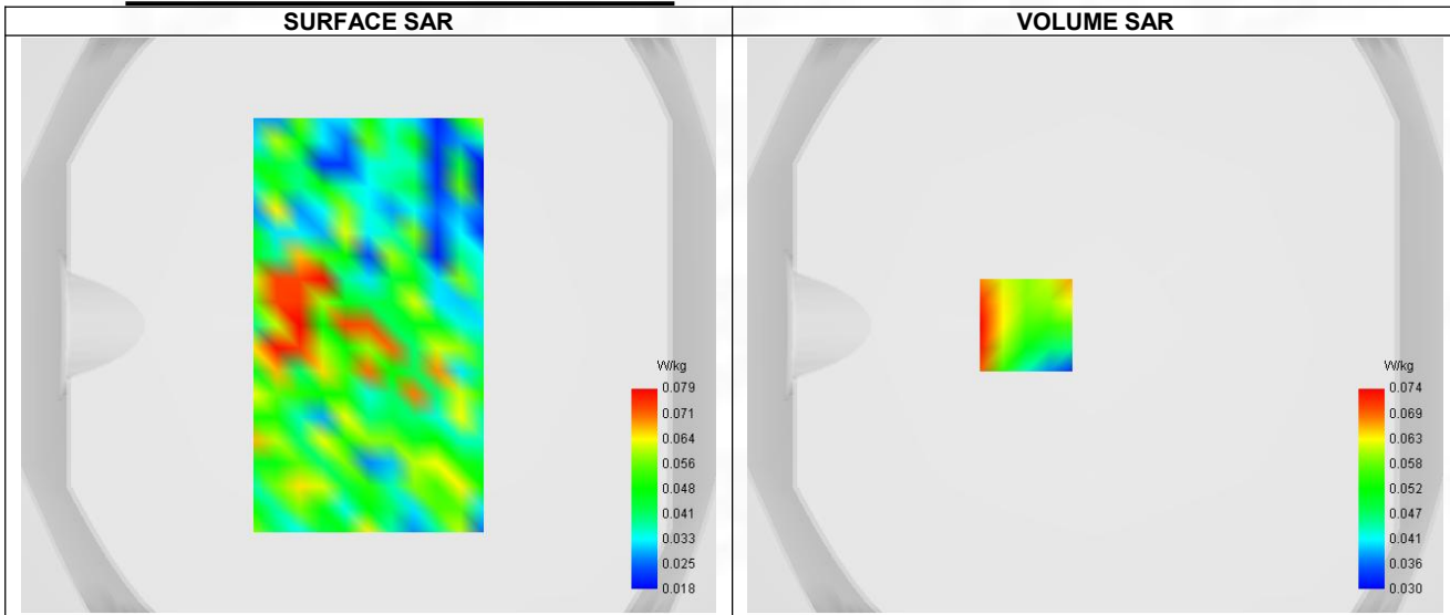
Maximum location: X=-24.00, Y=0.00 ; SAR Peak: 0.12 W/kg
