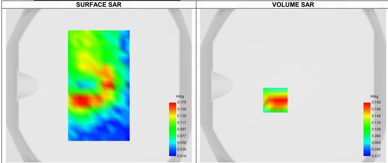
Maximum location: X=-23.00, Y=-19.00 ; SAR Peak: 0.28 W/kg
