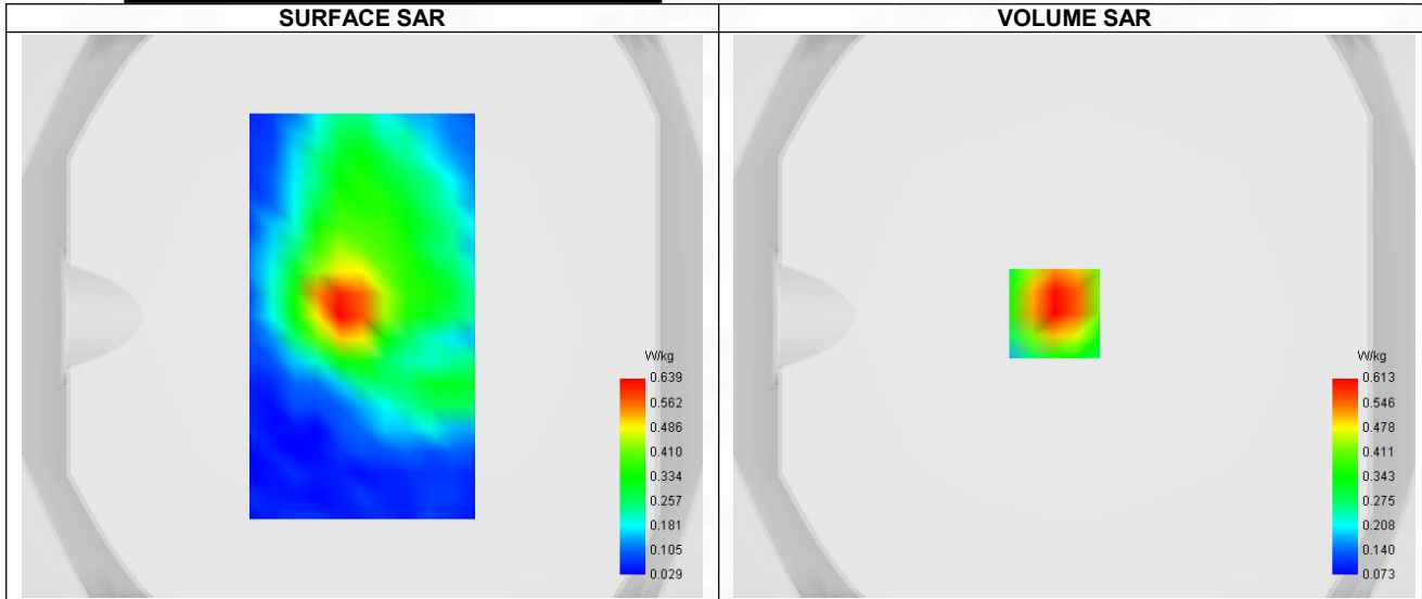
Maximum location: X=-7.00, Y=1.00 ; SAR Peak: 0.89 W/kg
