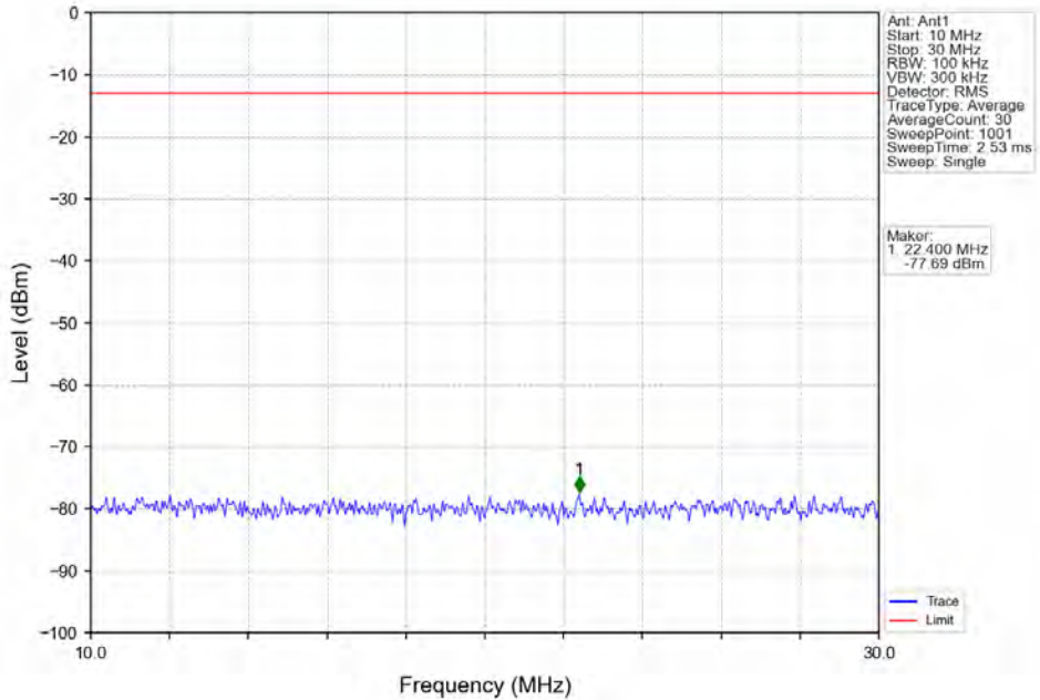
Band71_15MHz_16QAM_LCH_670.5MHz_RB_1_0_NTNV
