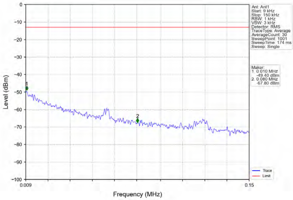
Band71_5MHz_16QAM_MCH_680.5MHz_RB_1_0_NTNV
