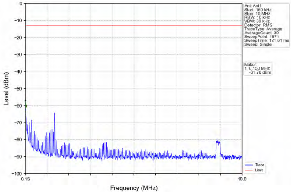
Band71_20MHz_16QAM_MCH_683MHz_RB_1_0_NTNV
