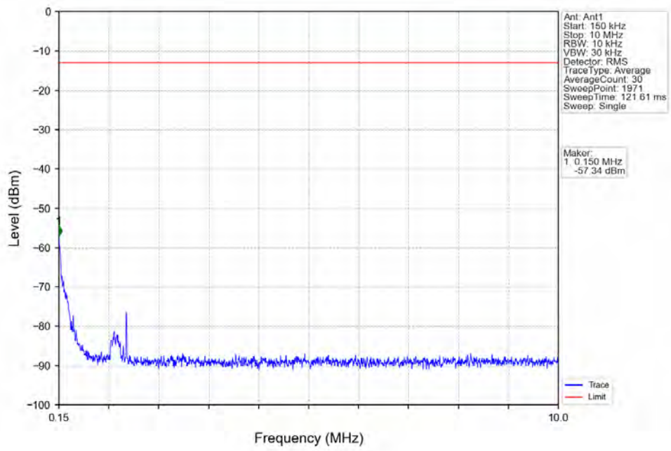
Band5_3MHz_QPSK_LCH_825.5MHz_RB_1_0_NTNV
