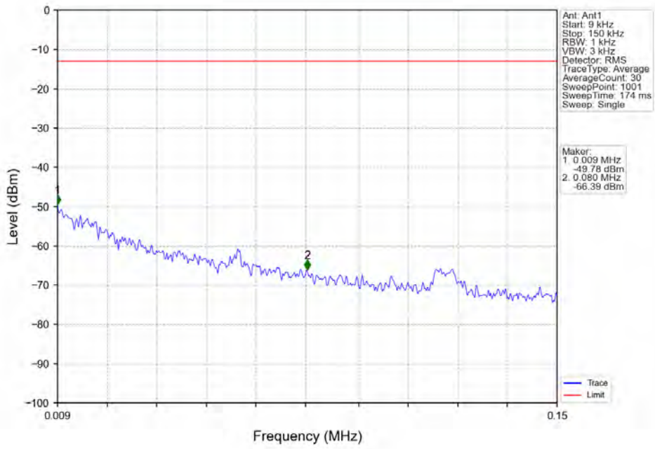
Band5_1.4MHz_16QAM_MCH_836.5MHz_RB_1_0_NTNV
