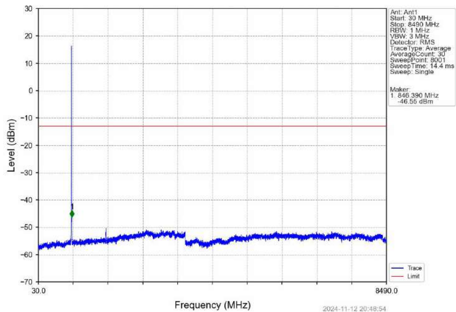
Band5_RMC_MCH_836.6MHz_12.2kbps RMC_NTNV
