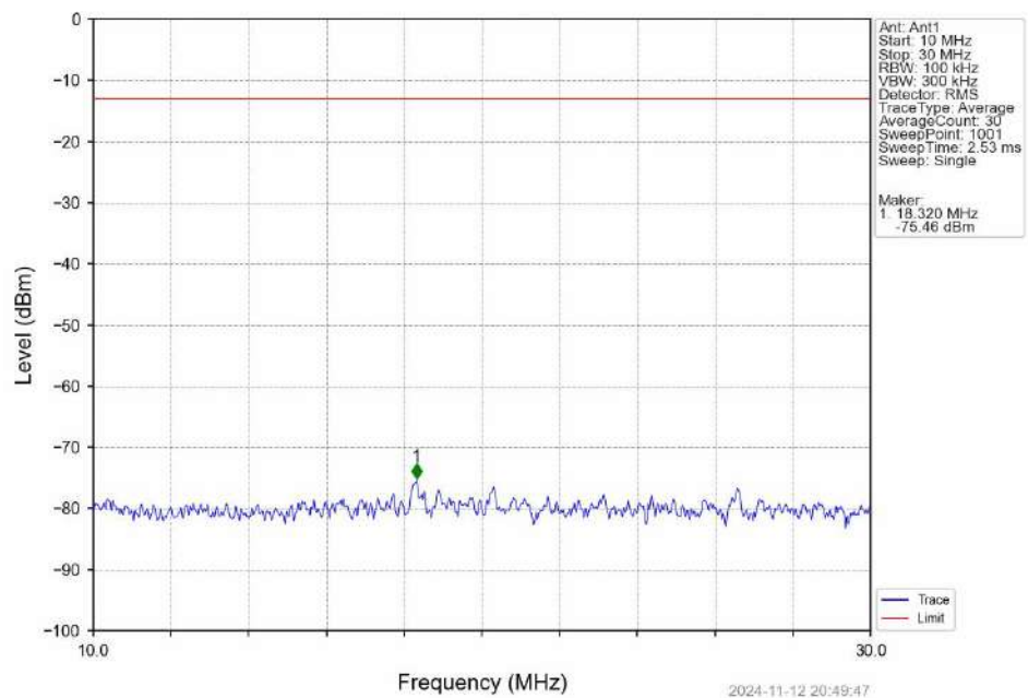
Band5_RMC_HCH_846.6MHz_12.2kbps RMC_NTNV
