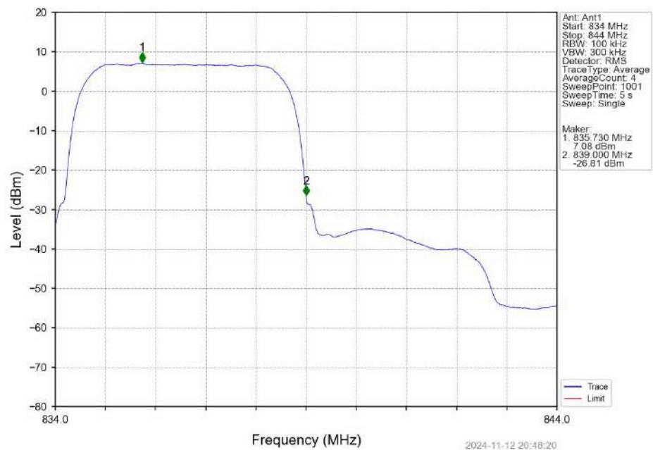
Band5_RMC_MCH_836.6MHz_12.2kbps RMC_NTNV
