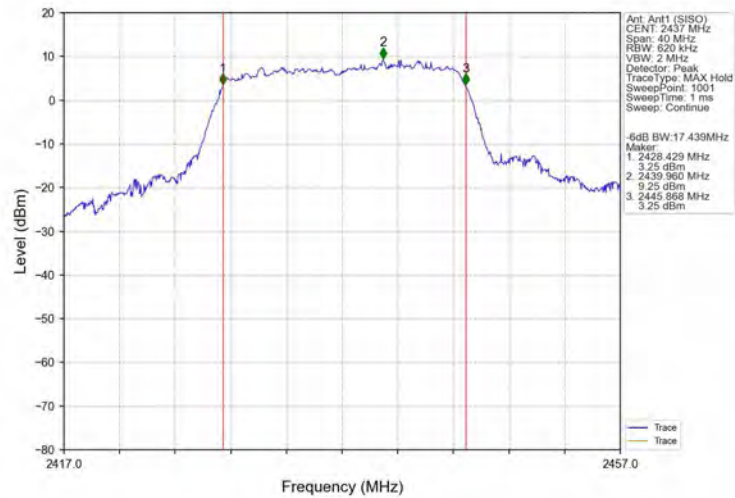
-6dB_Bandwidth_NVNT_ANT1_802_11n(HT20)_2437
