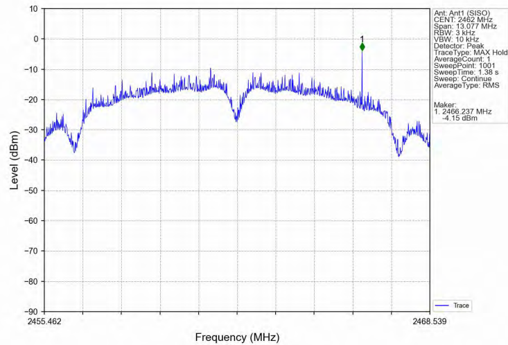
Power_Spectral_Density_NVNT_ANT1_802_11b_2462
