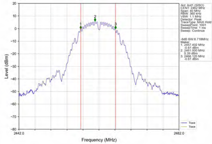
-6dB_Bandwidth_NVNT_ANT1_802_11b_2462
