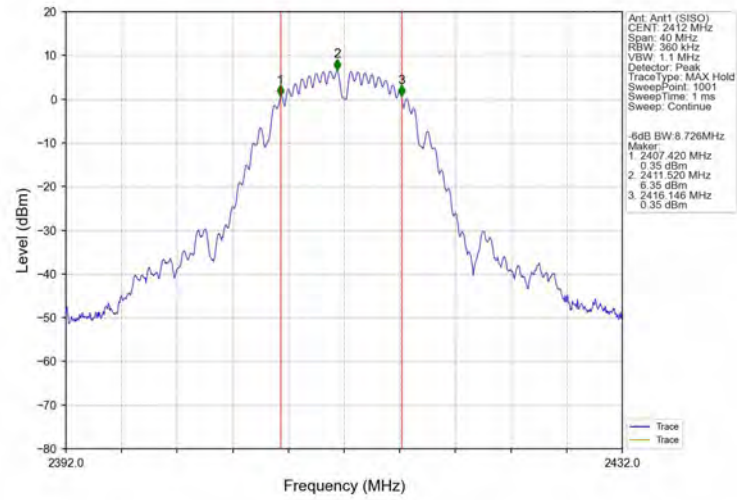
-6dB_Bandwidth_NVNT_ANT1_802_11b_2412
