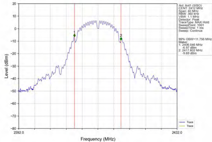
99%_Occupied_Bandwidth_NVNT_ANT1_802_11b_2412
