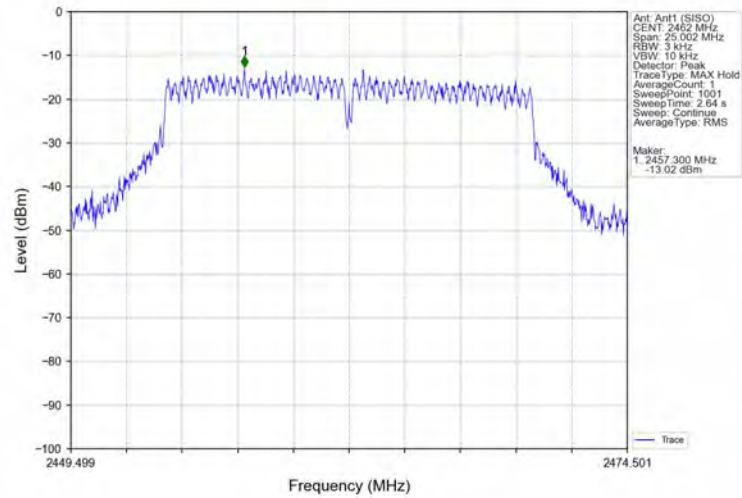
Power_Spectral_Density_NVNT_ANT1_802_11g_2462
