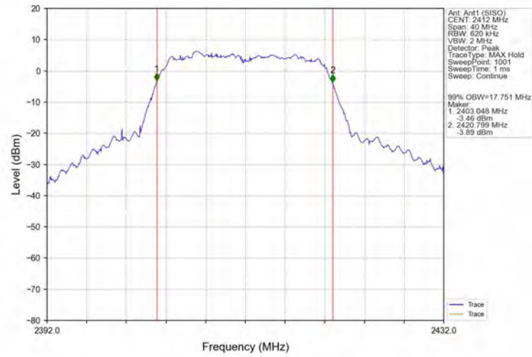
99%_Occupied_Bandwidth_NVNT_ANT1_802_11g_2412
