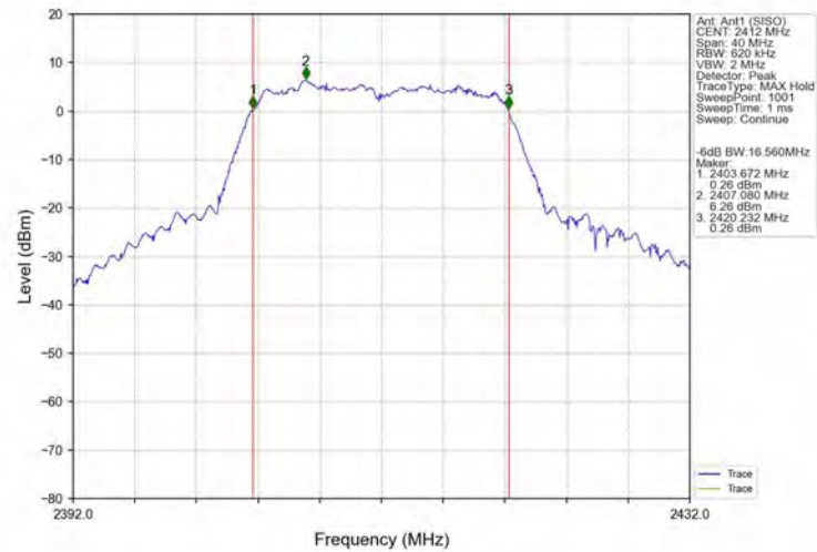
-6dB_Bandwidth_NVNT_ANT1_802_11g_2412
