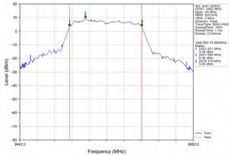
-6dB_Bandwidth_NVNT_ANT1_802_11g_2462
