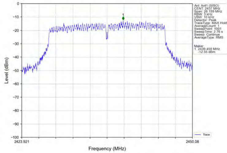
Power_Spectral_Density_NVNT_ANT1_802_11n(HT20)_2437
