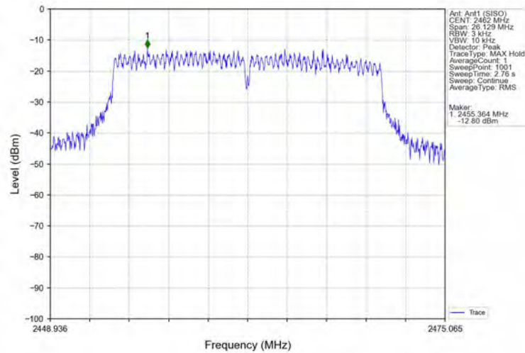
Power_Spectral_Density_NVNT_ANT1_802_11n(HT20)_2462
