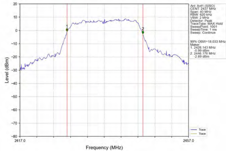
99%_Occupied_Bandwidth_NVNT_ANT1_802_11g_2437
