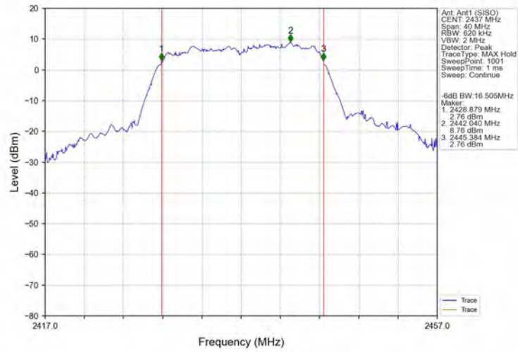
-6dB_Bandwidth_NVNT_ANT1_802_11g_2437
