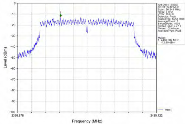
Power_Spectral_Density_NVNT_ANT1_802_11n(HT20)_2412
