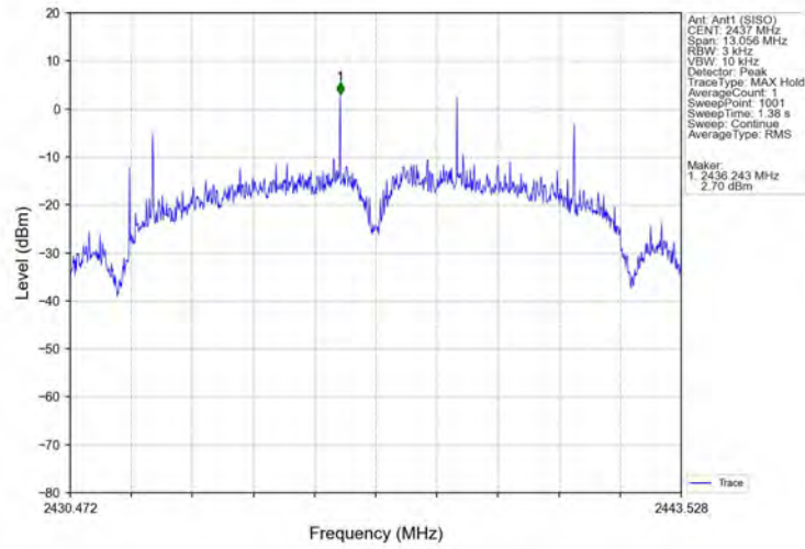
Power_Spectral_Density_NVNT_ANT1_802_11b_2437
