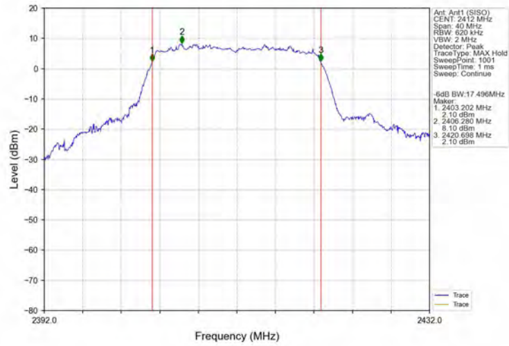
-6dB_Bandwidth_NVNT_ANT1_802_11n(HT20)_2412
