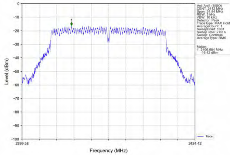
Power_Spectral_Density_NVNT_ANT1_802_11g_2412
