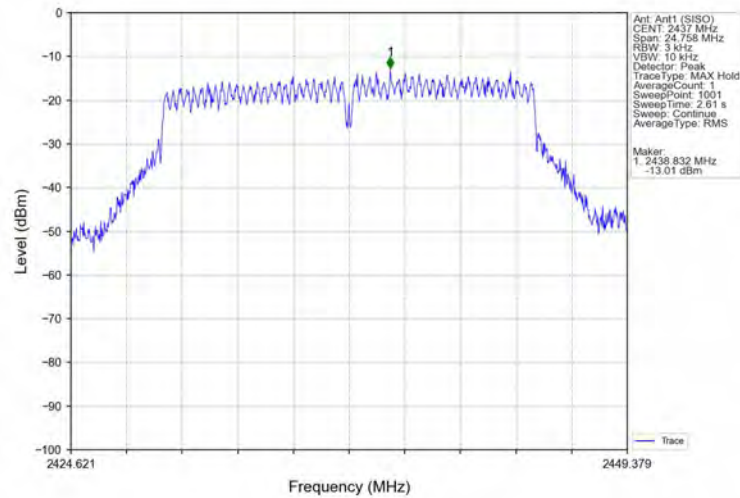
Power_Spectral_Density_NVNT_ANT1_802_11g_2437
