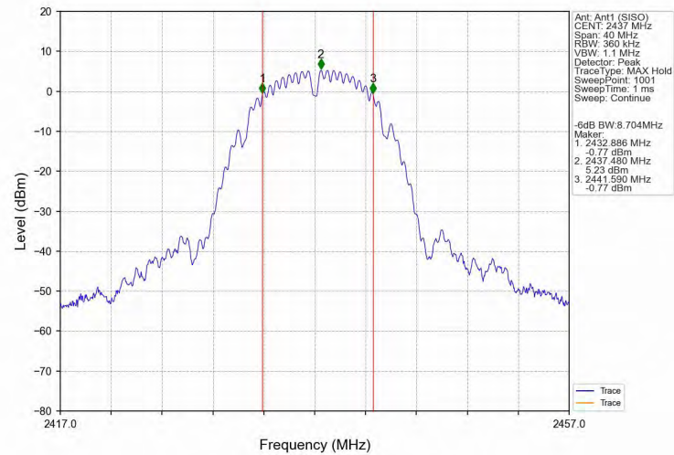
-6dB_Bandwidth_NVNT_ANT1_802_11b_2437
