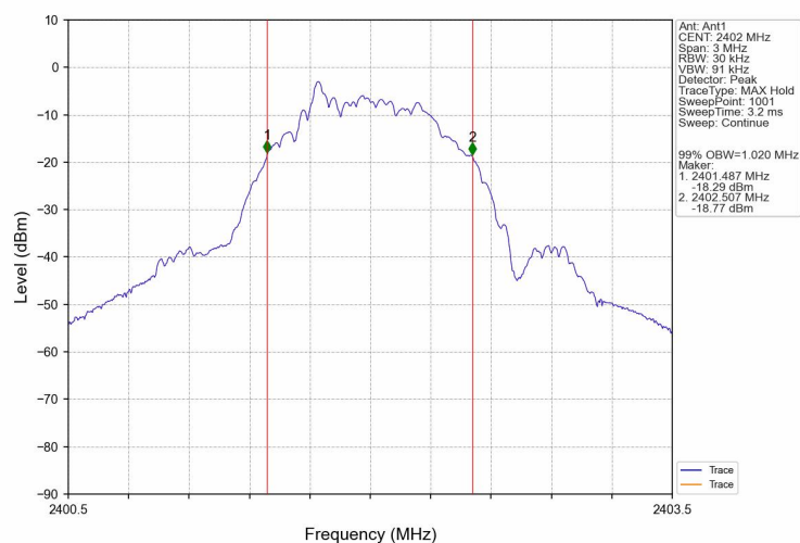
99%_Occupied_Bandwidth_NVNT_ANT1_1Mbps_2402
