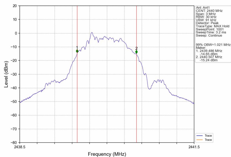
99%_Occupied_Bandwidth_NVNT_ANT1_1Mbps_2440
