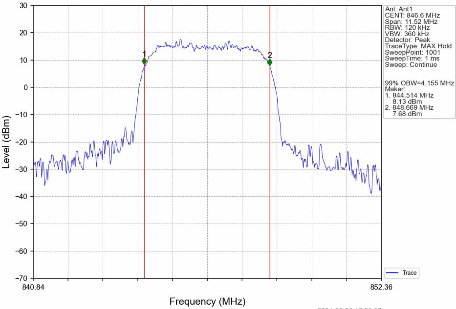
Band5_HSUPA_HCH_846.6MHz_Subtest 1_NTNV
