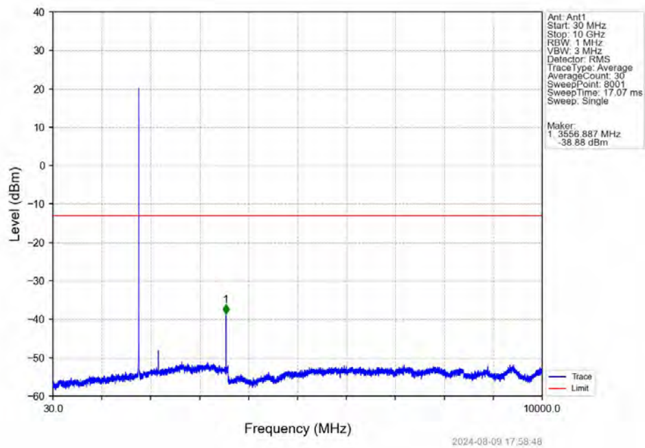
Band66_1.4MHz_16QAM_HCH_1779.3MHz_RB_1_0_NTNV
