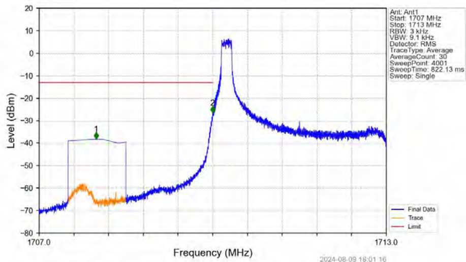
Band66_3MHz_16QAM_LCH_1711.5MHz_RB_1_0_NTNV
