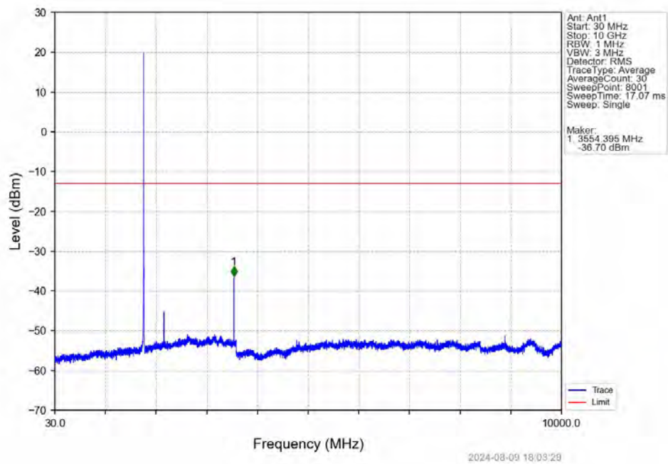
Band66_3MHz_16QAM_HCH_1778.5MHz_RB_1_0_NTNV
