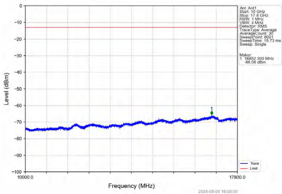
Band66_5MHz_QPSK_HCH_1777.5MHz_RB_1_0_NTNV
