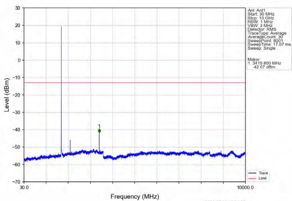
Band66_3MHz_16QAM_LCH_1711.5MHz_RB_1_0_NTNV
