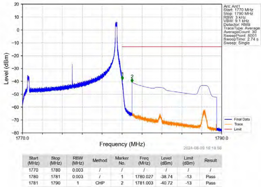
Band66_10MHz_16QAM_HCH_1775MHz_RB_50_0_NTNV
