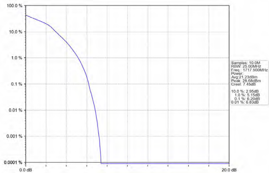
Band66_15MHz_16QAM_LCH_1717.5MHz_RB_75_0_NTNV
