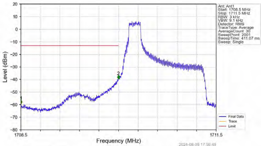
Band66_1.4MHz_16QAM_LCH_1710.7MHz_RB_1_0_NTNV
