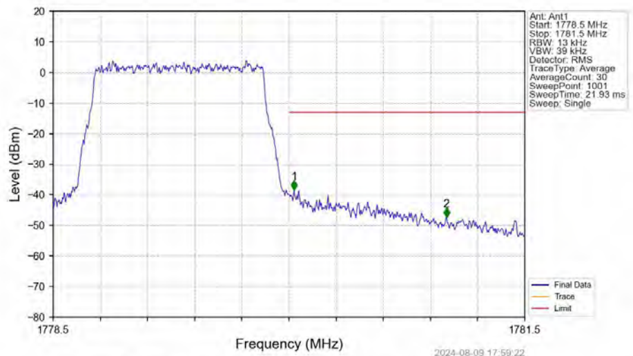
Band66_1.4MHz_16QAM_HCH_1779.3MHz_RB_6_0_NTNV
