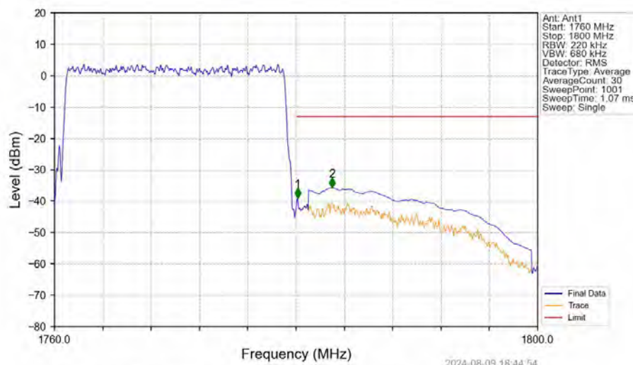
Band66_20MHz_16QAM_HCH_1770MHz_RB_100_0_NTNV
