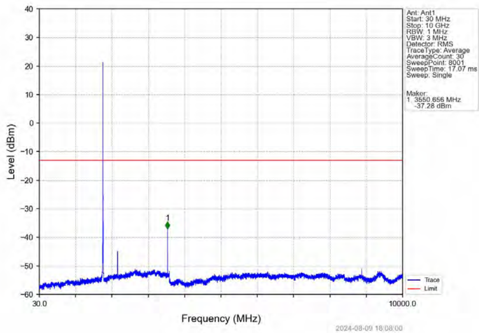
Band66_5MHz_QPSK_HCH_1777.5MHz_RB_1_0_NTNV
