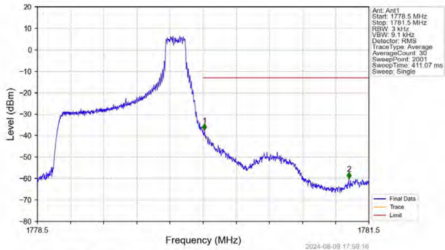
Band66_1.4MHz_16QAM_HCH_1779.3MHz_RB_1_5_NTNV
