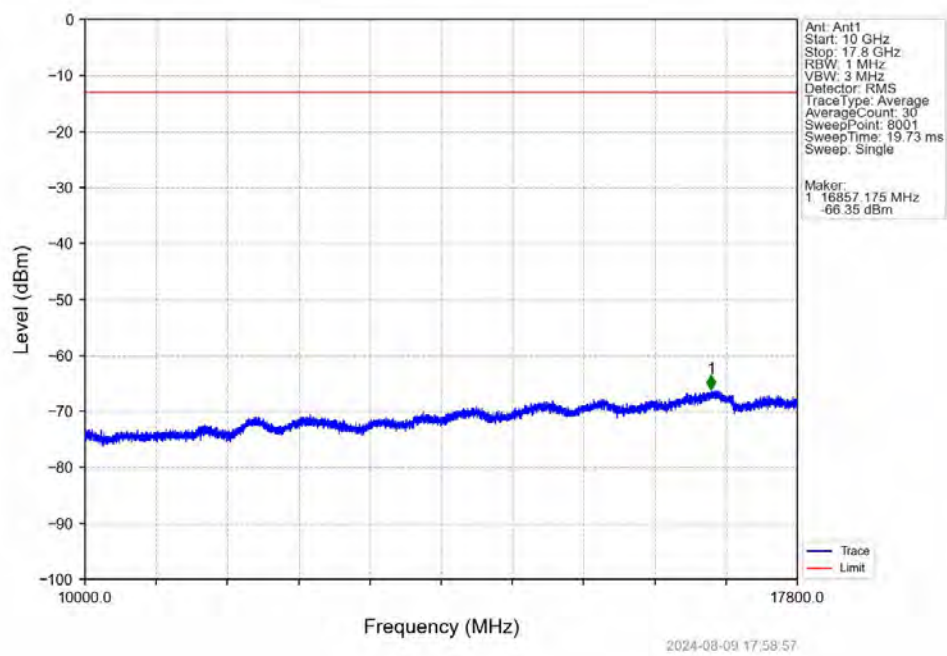
Band66_1.4MHz_16QAM_HCH_1779.3MHz_RB_1_0_NTNV
