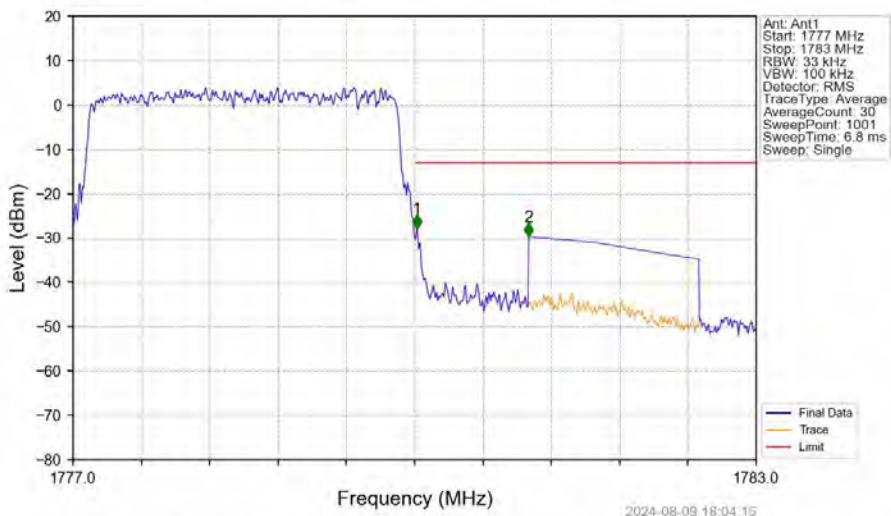
Band66_3MHz_16QAM_HCH_1778.5MHz_RB_15_0_NTNV
