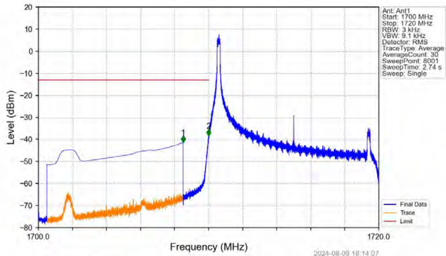
Band66_10MHz_16QAM_LCH_1715MHz_RB_1_0_NTNV
