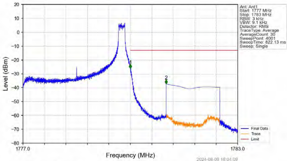
Band66_3MHz_16QAM_HCH_1778.5MHz_RB_1_14_NTNV
