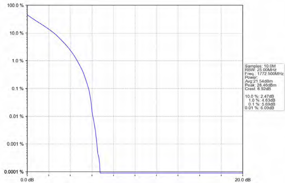
Band66_15MHz_QPSK_HCH_1772.5MHz_RB_75_0_NTNV
