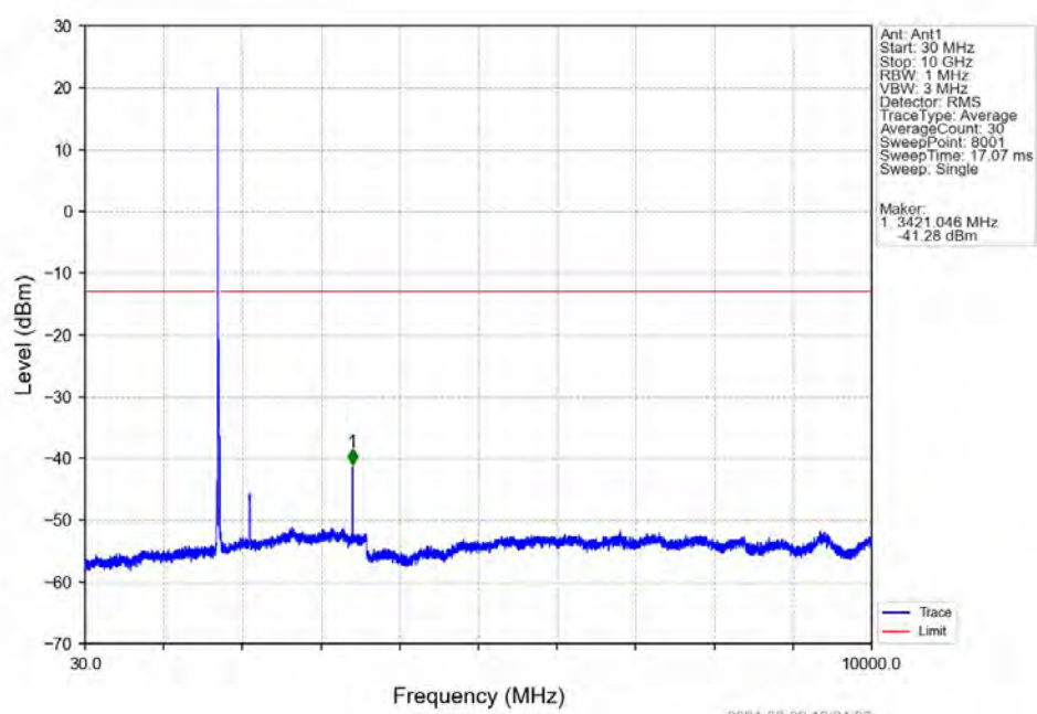
Band66_15MHz_16QAM_LCH_1717.5MHz_RB_1_0_NTNV
