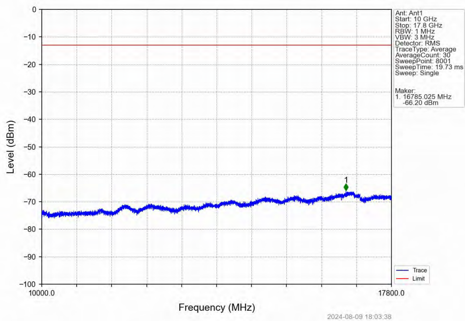
Band66_3MHz_16QAM_HCH_1778.5MHz_RB_1_0_NTNV
