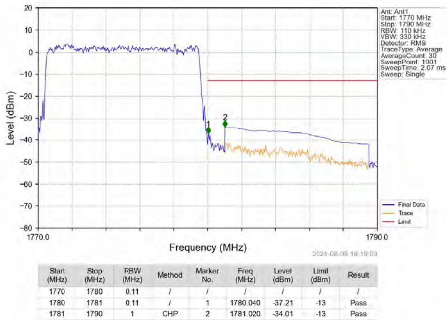
Band66_10MHz_16QAM_HCH_1775MHz_RB_50_0_NTNV
