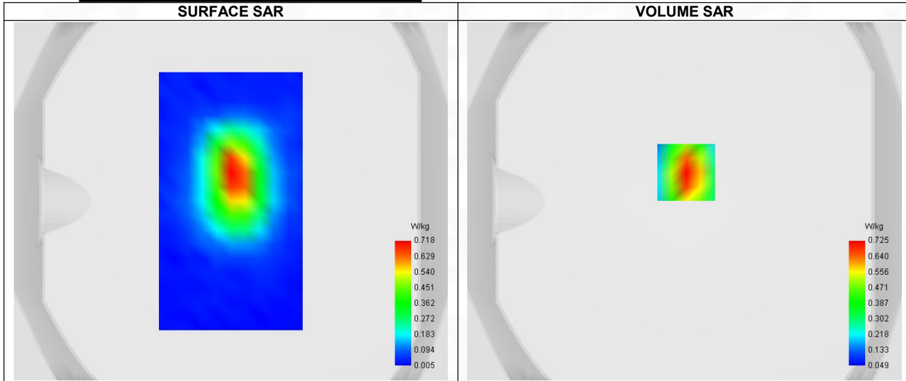
Maximum location: X=1.00, Y=16.00 ; SAR Peak: 1.05 W/kg
