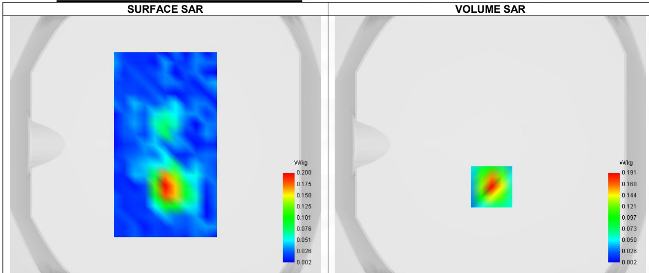
Maximum location: X=1.00, Y=-33.00 ; SAR Peak: 0.28 W/kg
