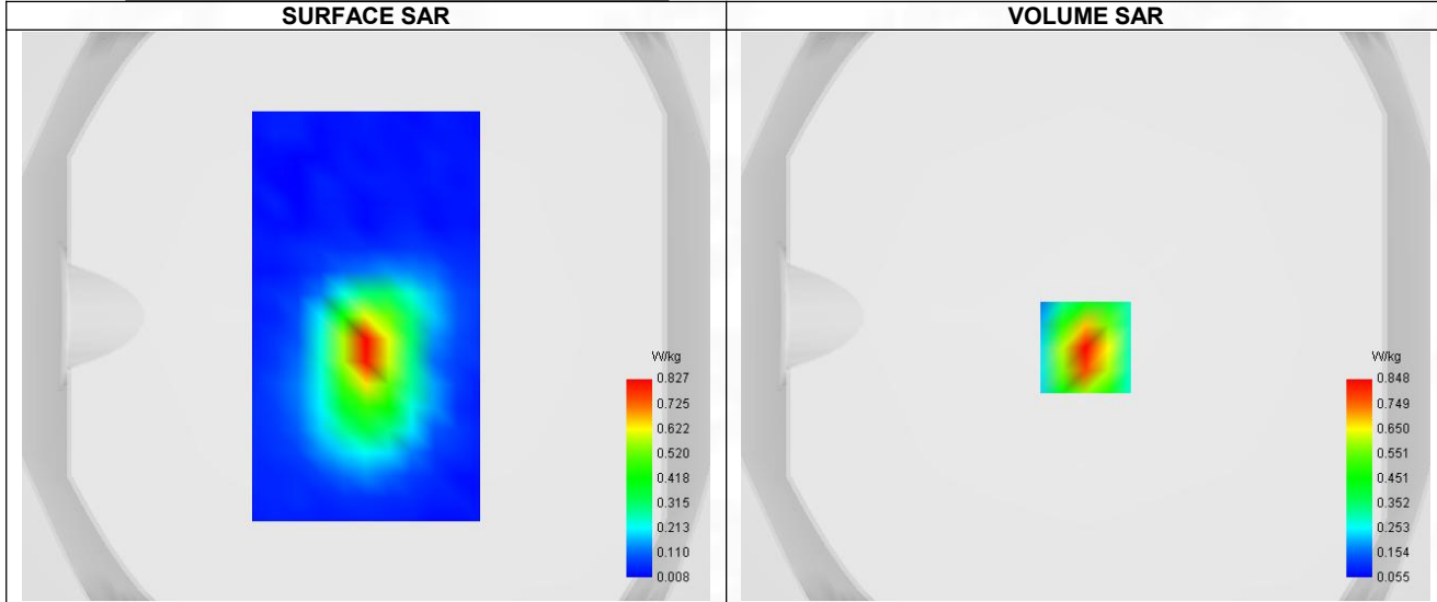
Maximum location: X=0.00, Y=-11.00 ; SAR Peak: 1.24 W/kg
