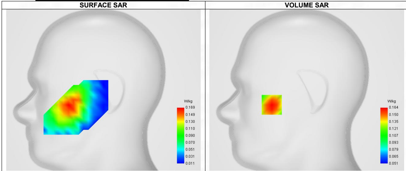
Maximum location: X=-56.00, Y=-24.00 ; SAR Peak: 0.19 W/kg
