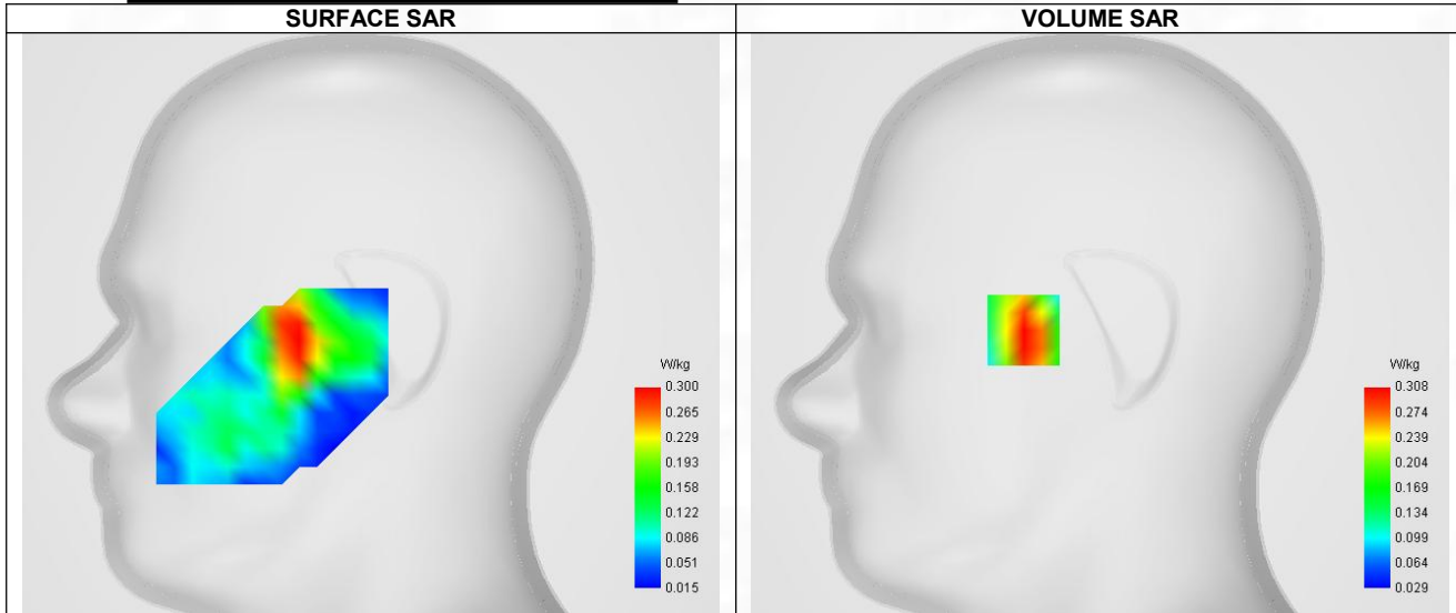
Maximum location: X=-34.00, Y=-3.00 ; SAR Peak: 0.36 W/kg
