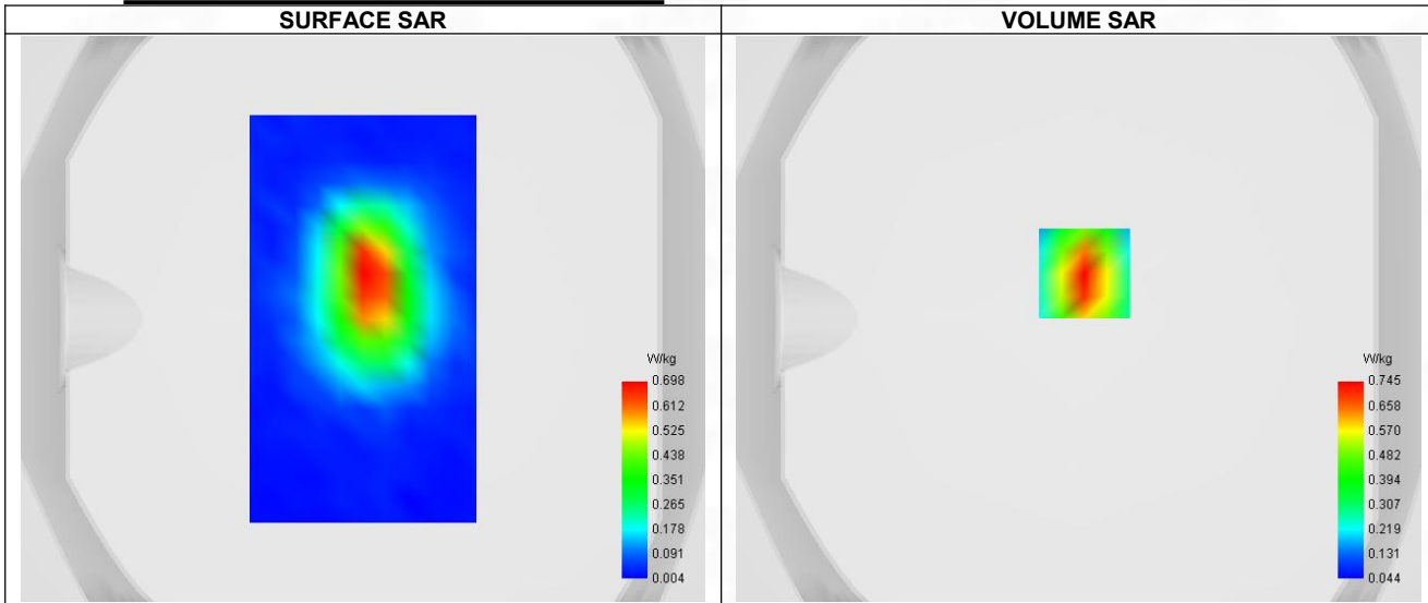
Maximum location: X=2.00, Y=16.00 ; SAR Peak: 1.09 W/kg
