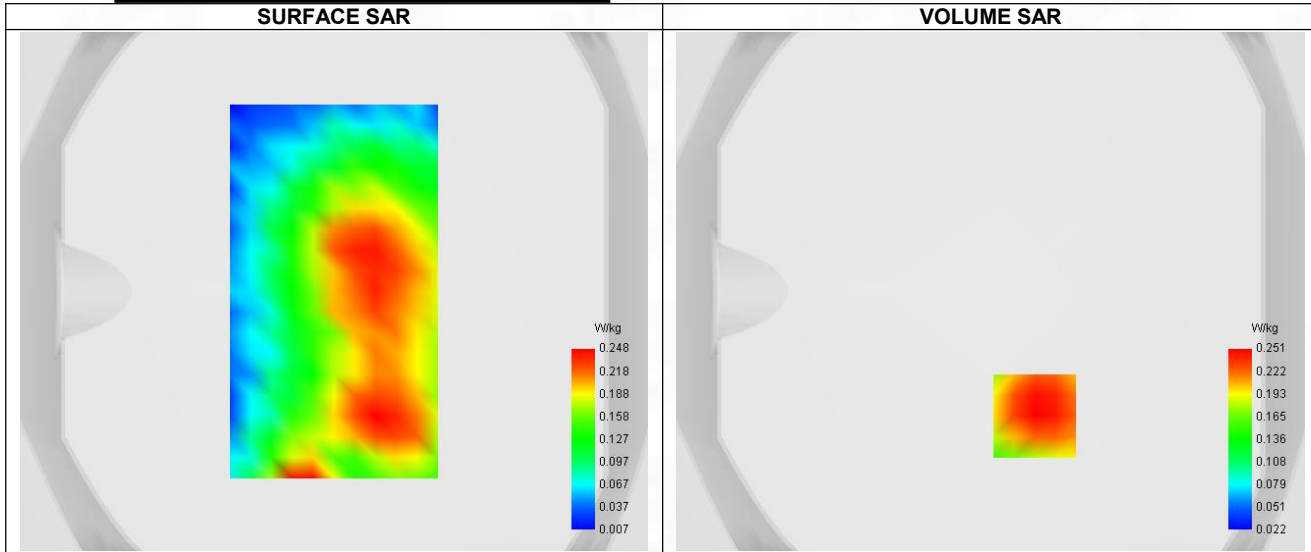
Maximum location: X=17.00, Y=-48.00 ; SAR Peak: 0.32 W/kg
