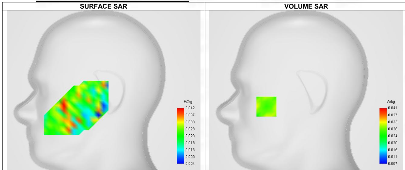
Maximum location: X=-64.00, Y=-26.00 ; SAR Peak: 0.07 W/kg
