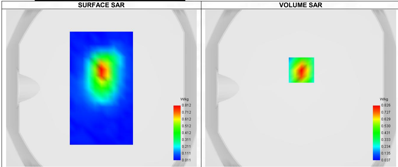
Maximum location: X=1.00, Y=23.00 ; SAR Peak: 1.21 W/kg
