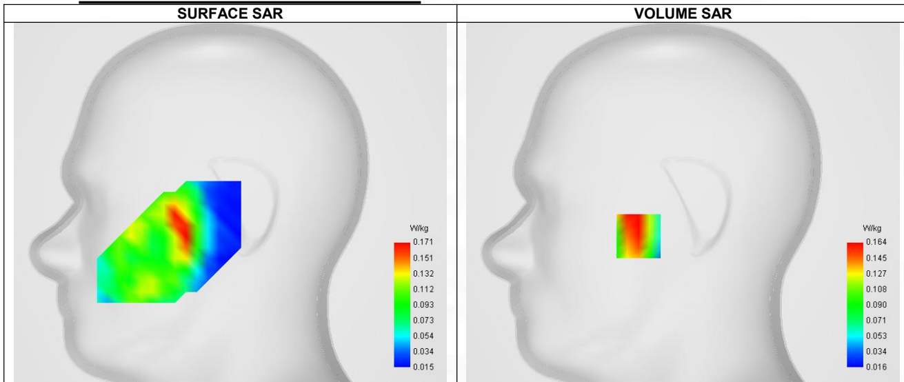
Maximum location: X=-32.00, Y=-24.00 ; SAR Peak: 0.22 W/kg
