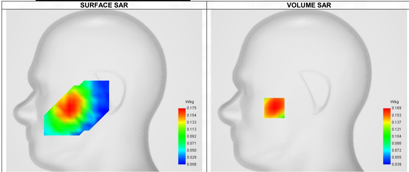
Maximum location: X=-55.00, Y=-28.00 ; SAR Peak: 0.21 W/kg
