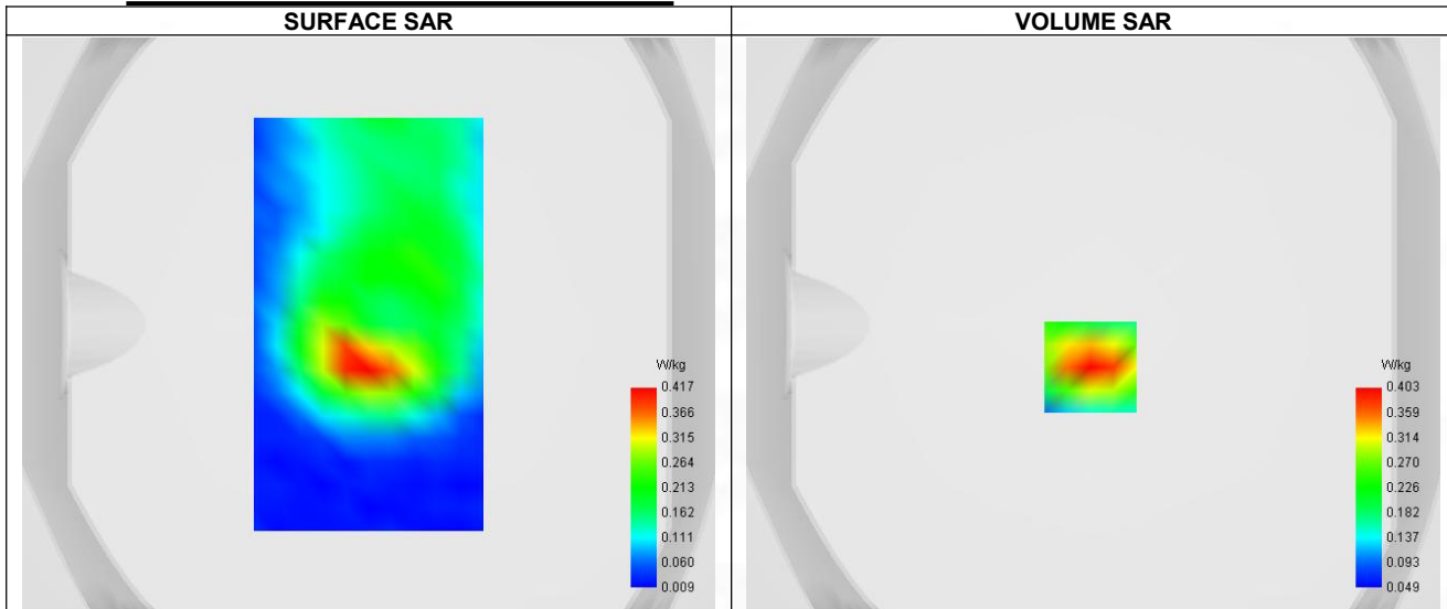
Maximum location: X=-1.00, Y=-15.00 ; SAR Peak: 0.54 W/kg
