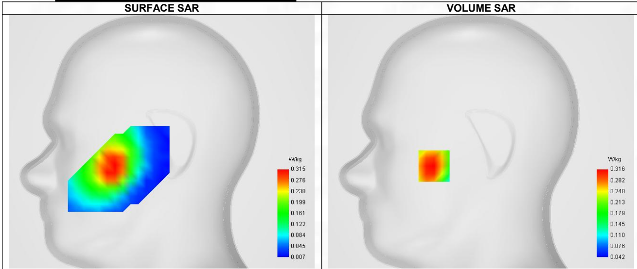
Maximum location: X=-48.00, Y=-25.00 ; SAR Peak: 0.38 W/kg
