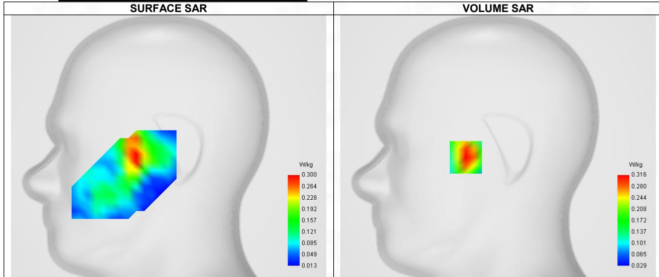
Maximum location: X=-32.00, Y=-11.00 ; SAR Peak: 0.41 W/kg
