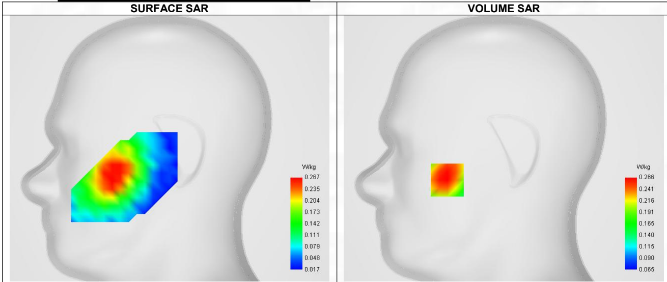
Maximum location: X=-55.00, Y=-31.00 ; SAR Peak: 0.32 W/kg
