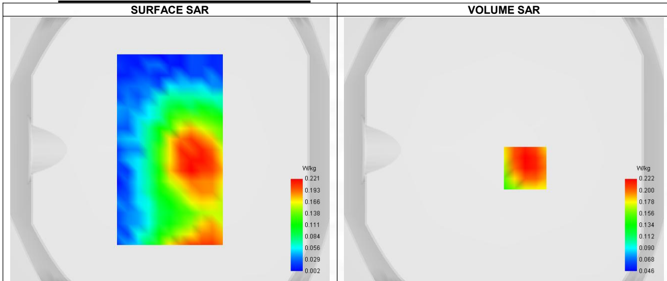
Maximum location: X=16.00, Y=-14.00 ; SAR Peak: 0.27 W/kg
