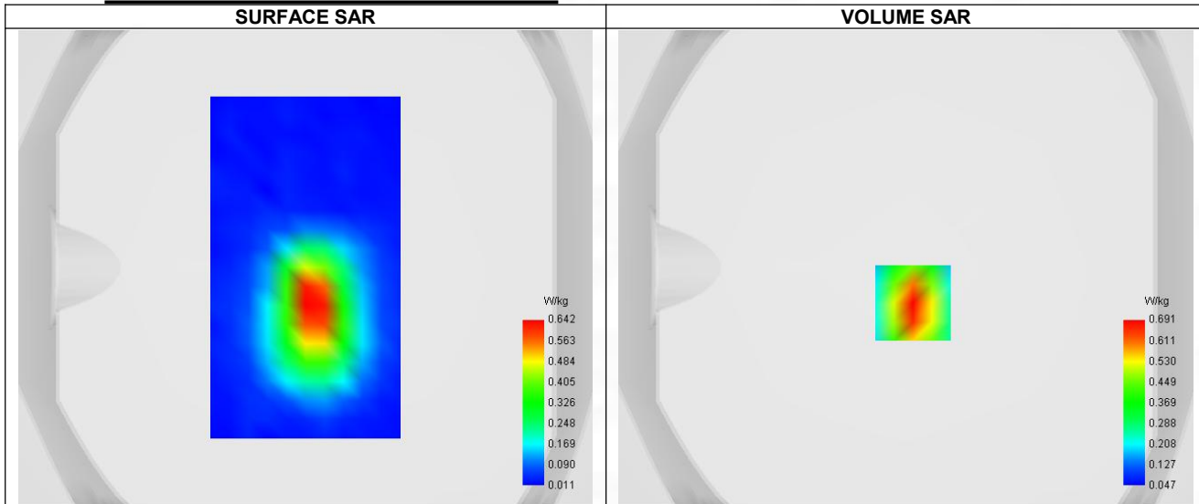
Maximum location: X=3.00, Y=-15.00 ; SAR Peak: 1.05 W/kg
