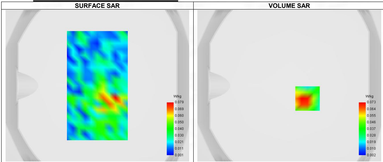
Maximum location: X=24.00, Y=-17.00 ; SAR Peak: 0.12 W/kg
