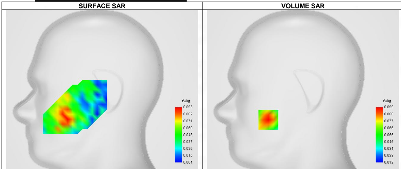
Maximum location: X=-56.00, Y=-49.00 ; SAR Peak: 0.14 W/kg
