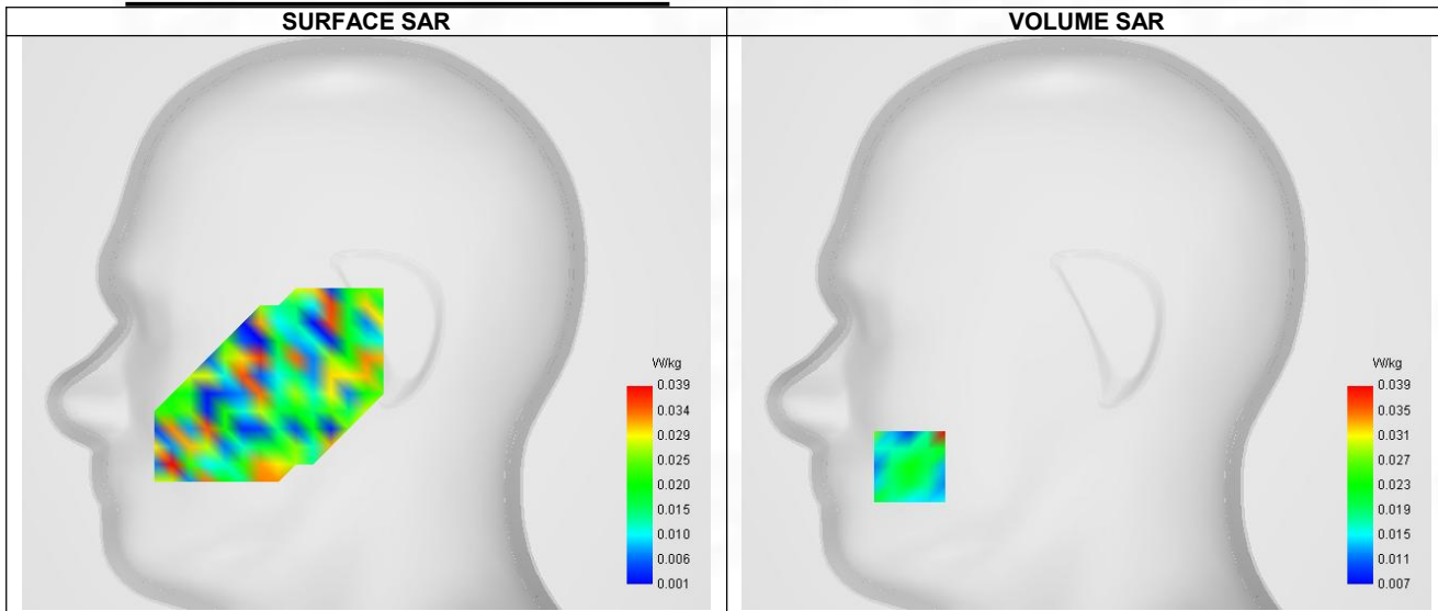
Maximum location: X=-80.00, Y=-65.00 ; SAR Peak: 0.07 W/kg
