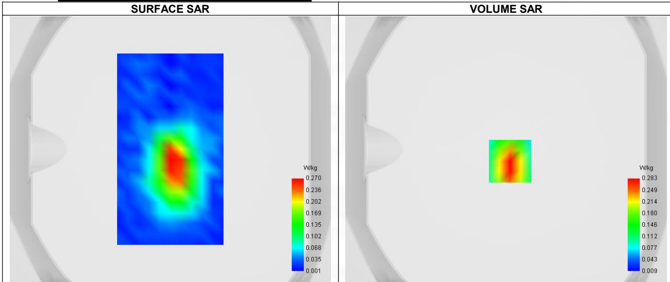
Maximum location: X=3.00, Y=-9.00 ; SAR Peak: 0.42 W/kg
