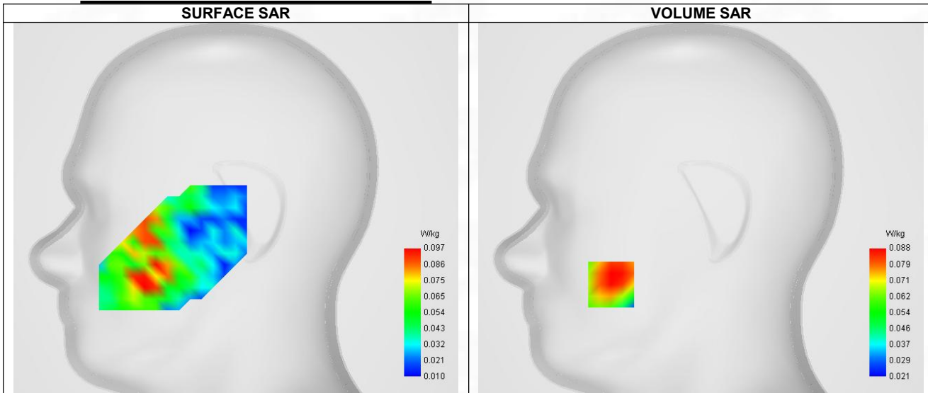
Maximum location: X=-63.00, Y=-54.00 ; SAR Peak: 0.13 W/kg
