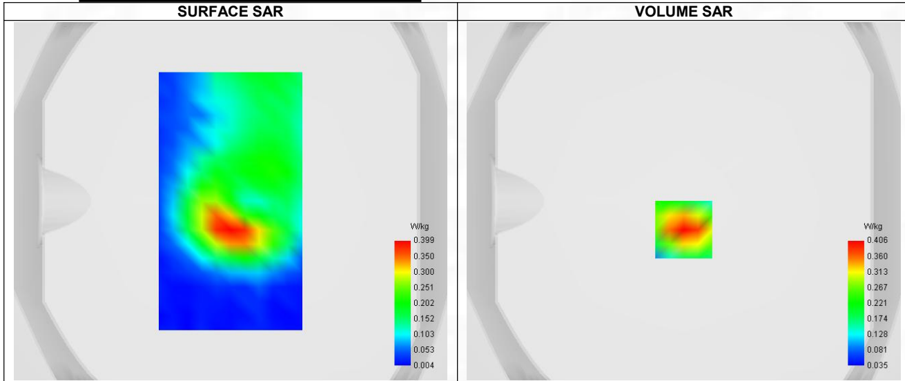
Maximum location: X=0.00, Y=-16.00 ; SAR Peak: 0.60 W/kg
