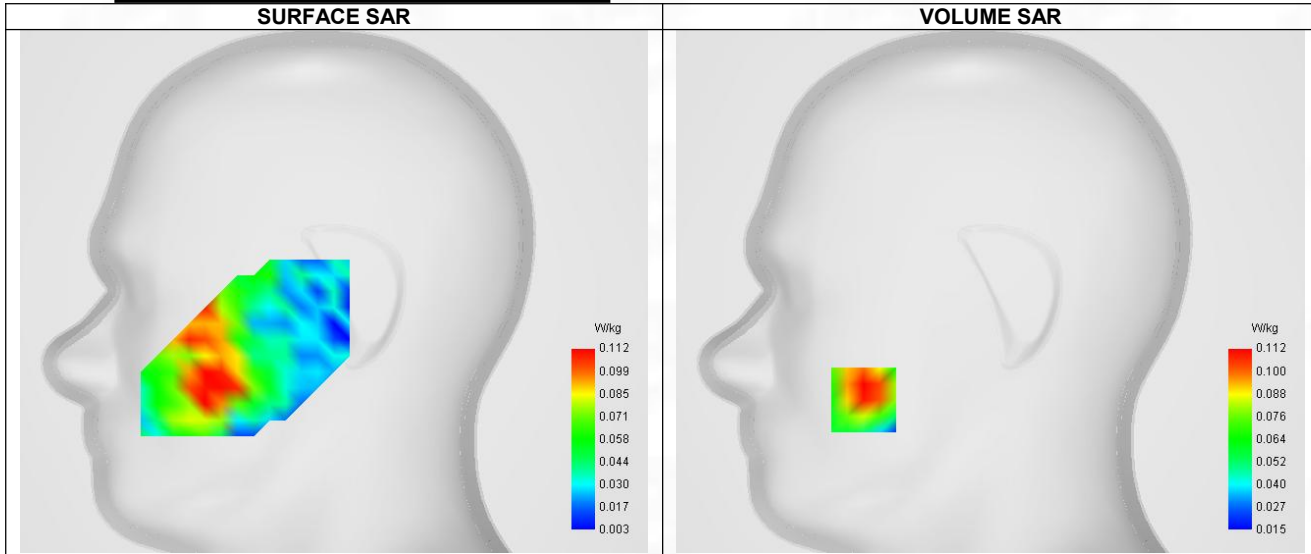
Maximum location: X=-63.00, Y=-54.00 ; SAR Peak: 0.17 W/kg
