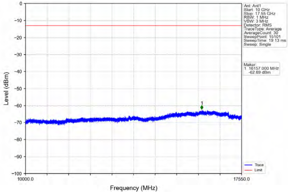
Band4_5MHz_16QAM_HCH_1752.5MHz_RB_1_0_NTNV
