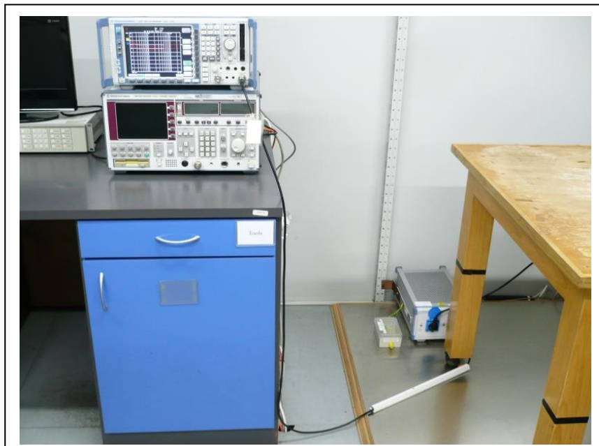
Measurement equipment
