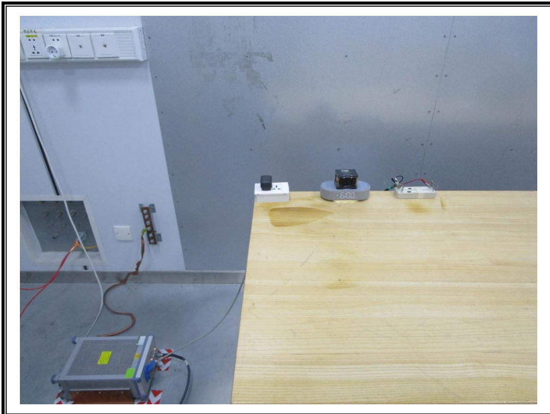
POWERLINE CONDUCTED EMISSIONS MEASUREMENT SETUP
