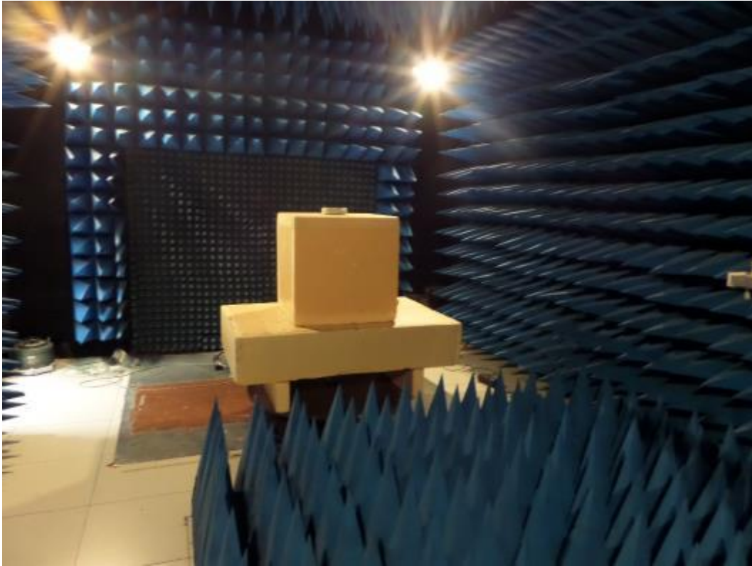
Anechoic room
