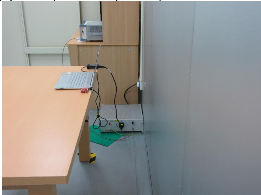
Photograph 8: Set-up for AC Mains (Back View)
