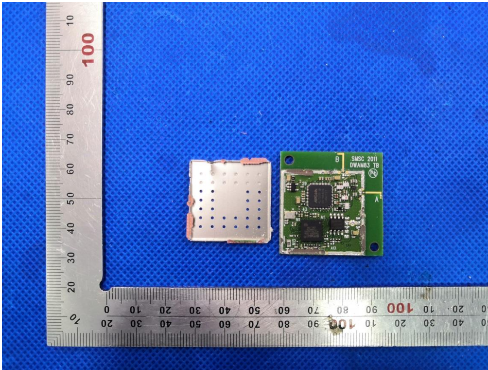
INTERNAL VIEW-10 OF EUT(WIFI MODULE)
