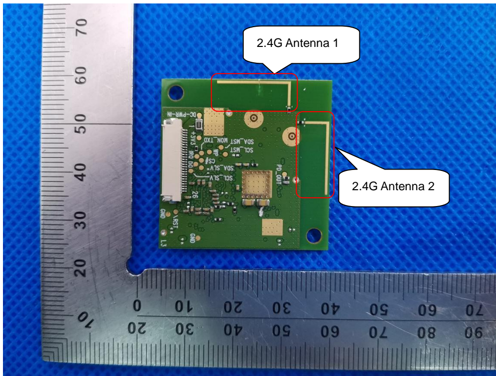
INTERNAL VIEW-12 OF EUT(WIFI MODULE)
