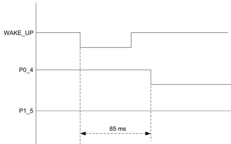
FIGURE 2-5: WAKE-UP TIME
