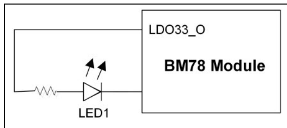
FIGURE 2-7: LED DRIVER
