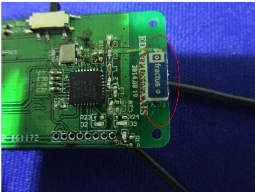
EUT –Chip Antenna View
