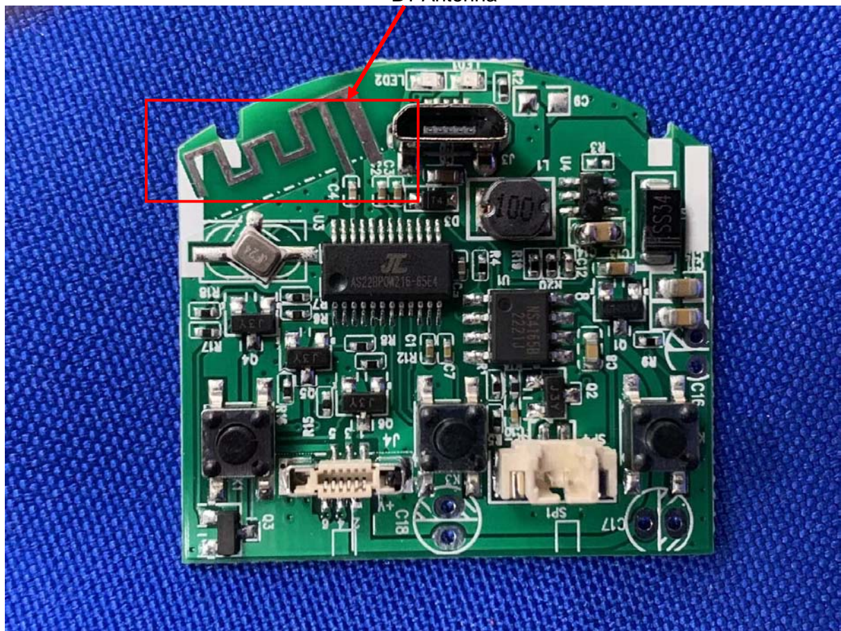
BT Antenna
