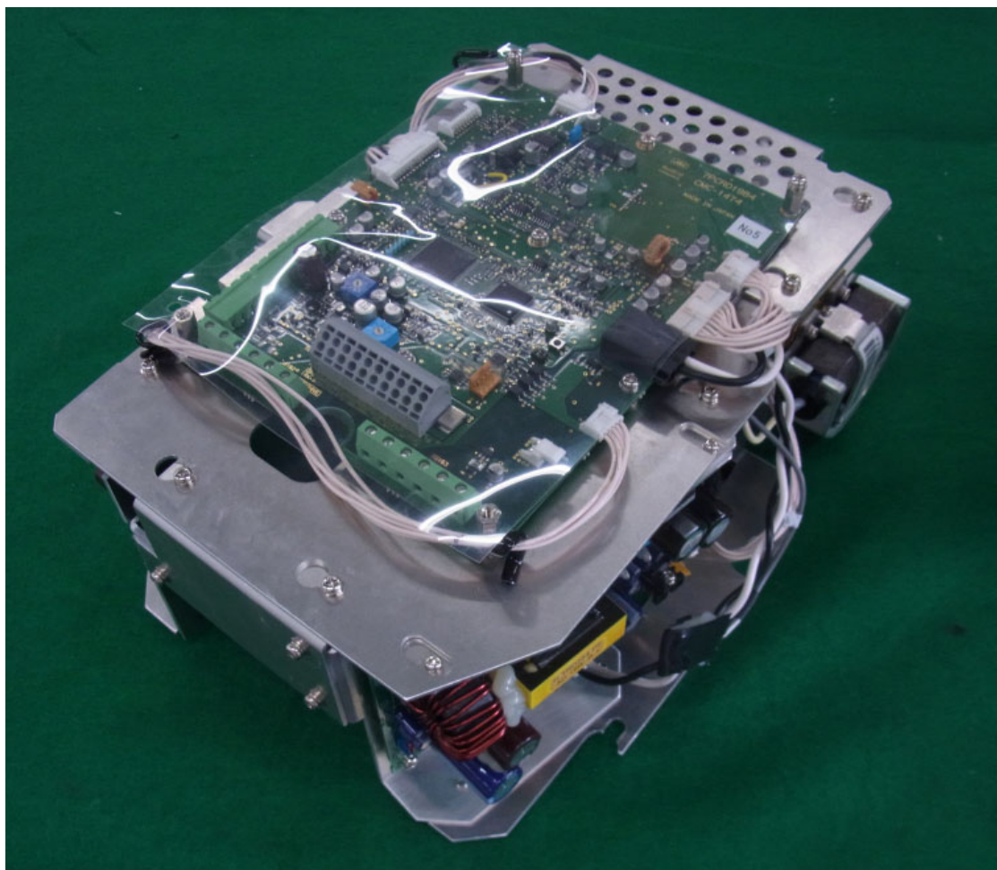
Transceiver Unit:NZT-18
