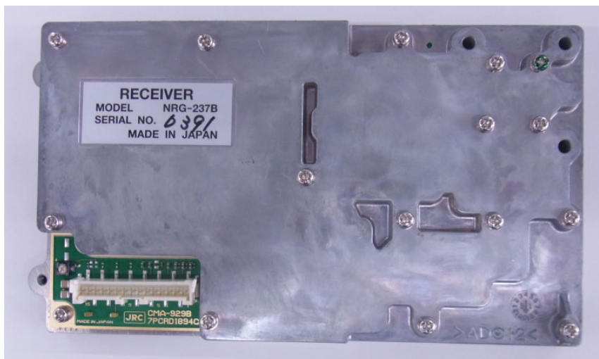
Receiver Unit:NRG-237B(including Receiver Circuit:CMA-929)
