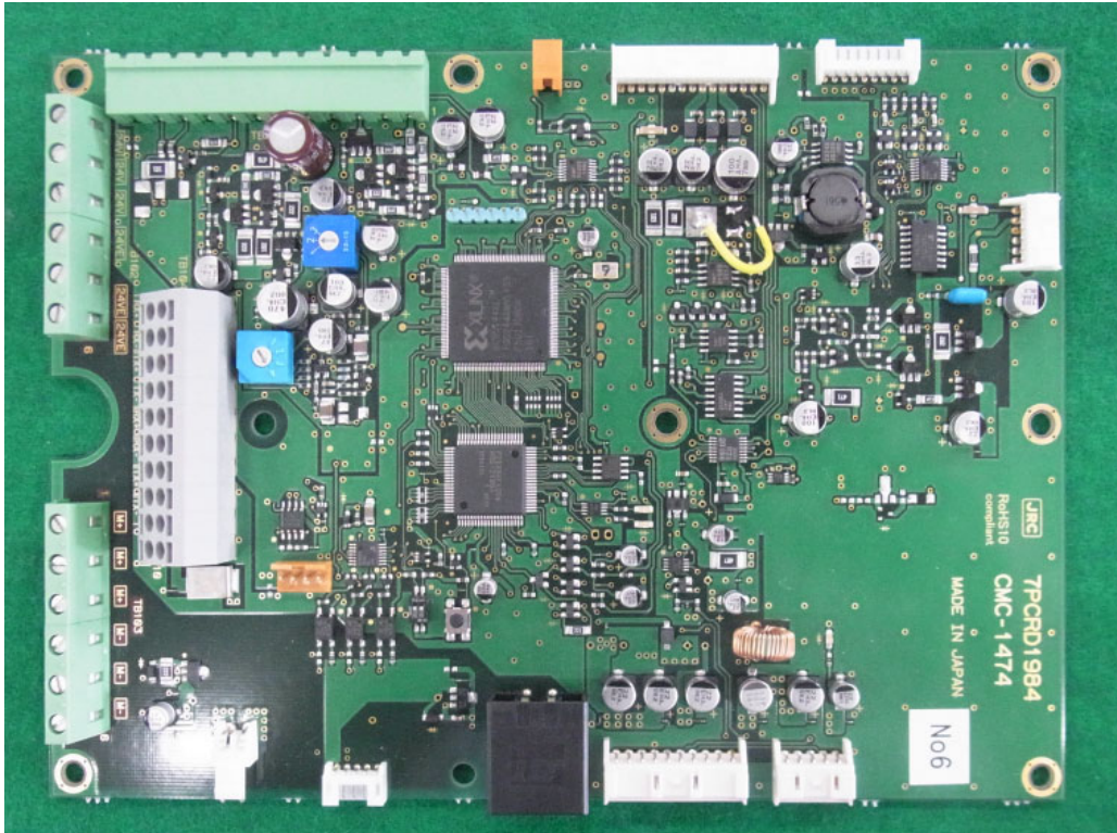
Control Circuit:CMC-1474
