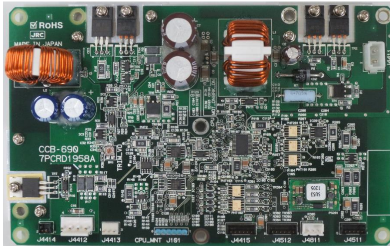
CCB-690 ( Motor Driver Circuit ) Parts Side
