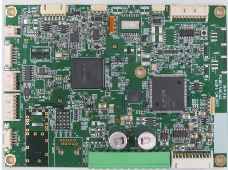
CMC-1429 ( Control Circuit ) Parts Side
