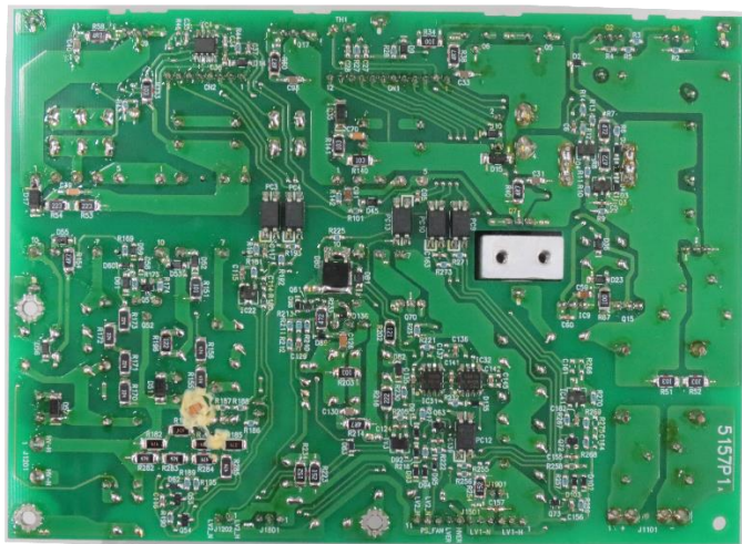
CBD-2682 ( Power Supply Circuit ) Solder Side
