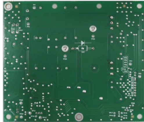
CME-406 ( Transmitter Circuit ) Parts and Solder Side
