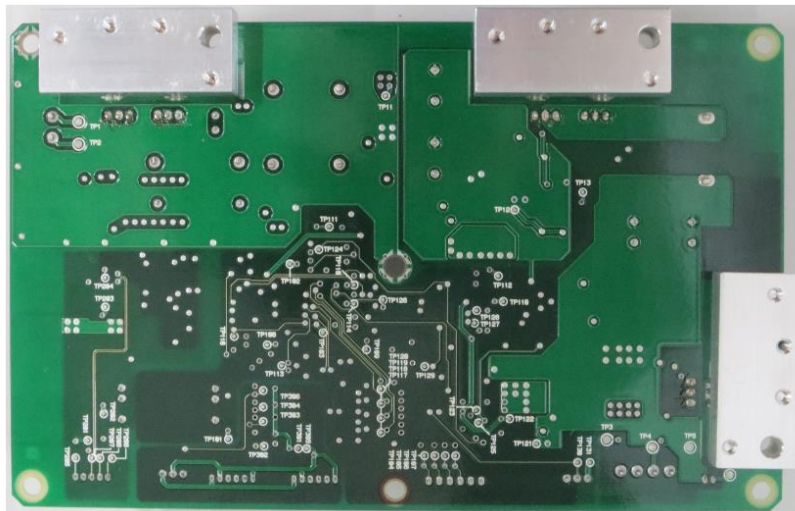
CCB-690 ( Motor Driver Circuit ) Solder Side
