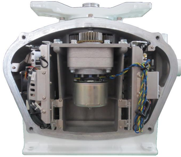
NKE-2255 without Starboard Side Cover
