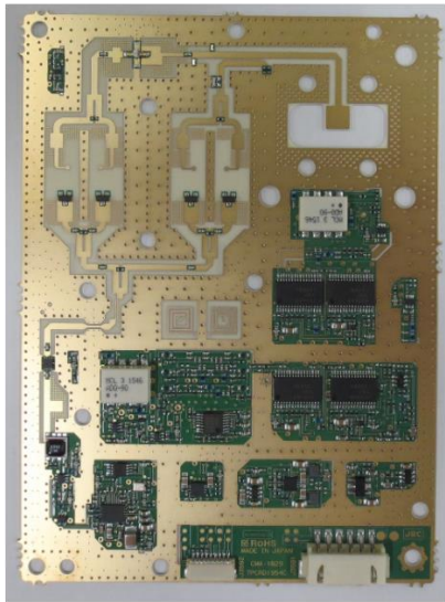
CMA-1029 ( Receiver Circuit ) Parts and Solder Side
