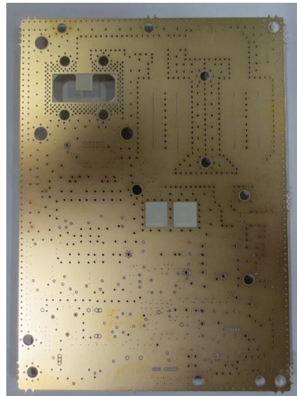
CMA-1029 ( Receiver Circuit ) Parts and Solder Side
