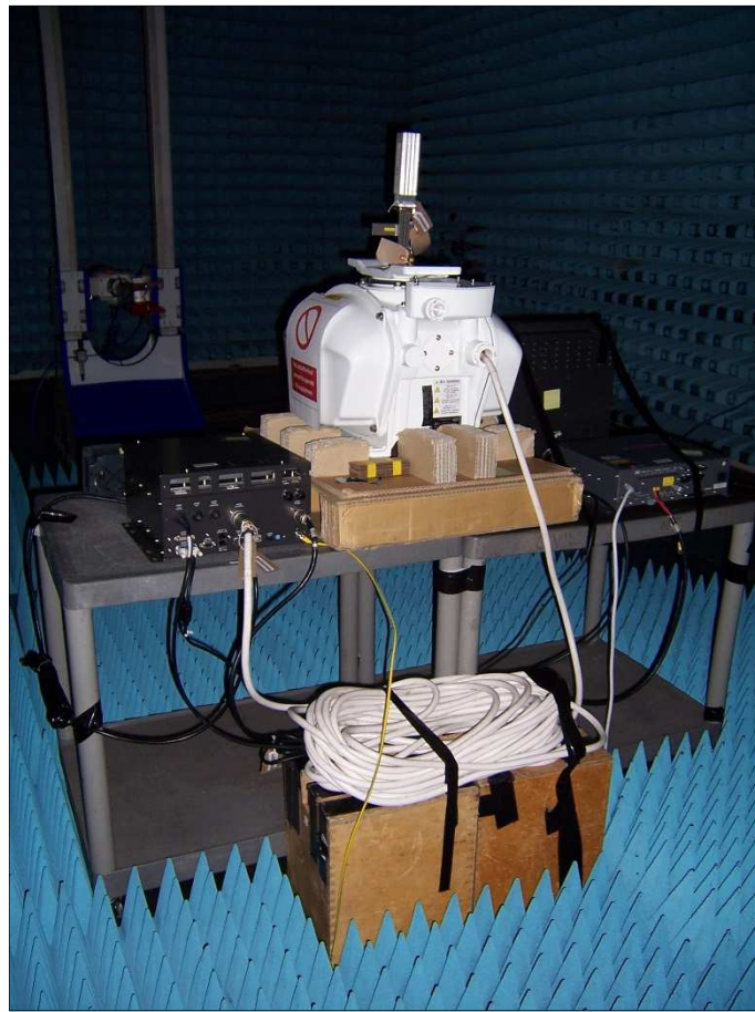
Figure 1 - Test Setup
