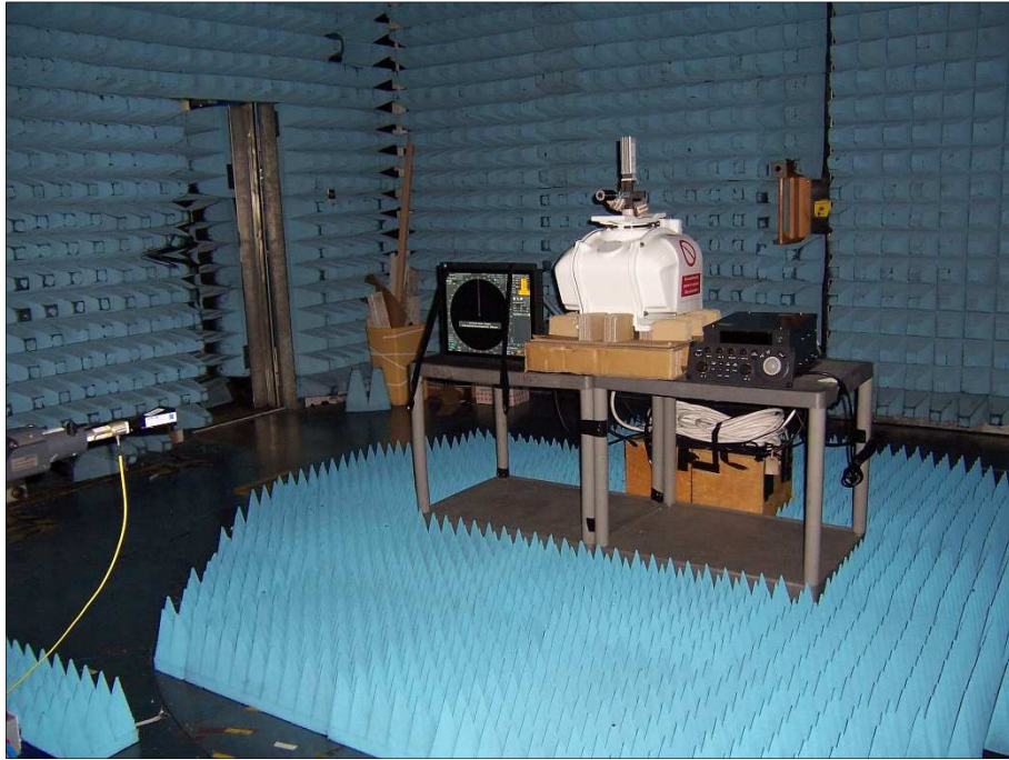
Figure 2 - Test Setup
