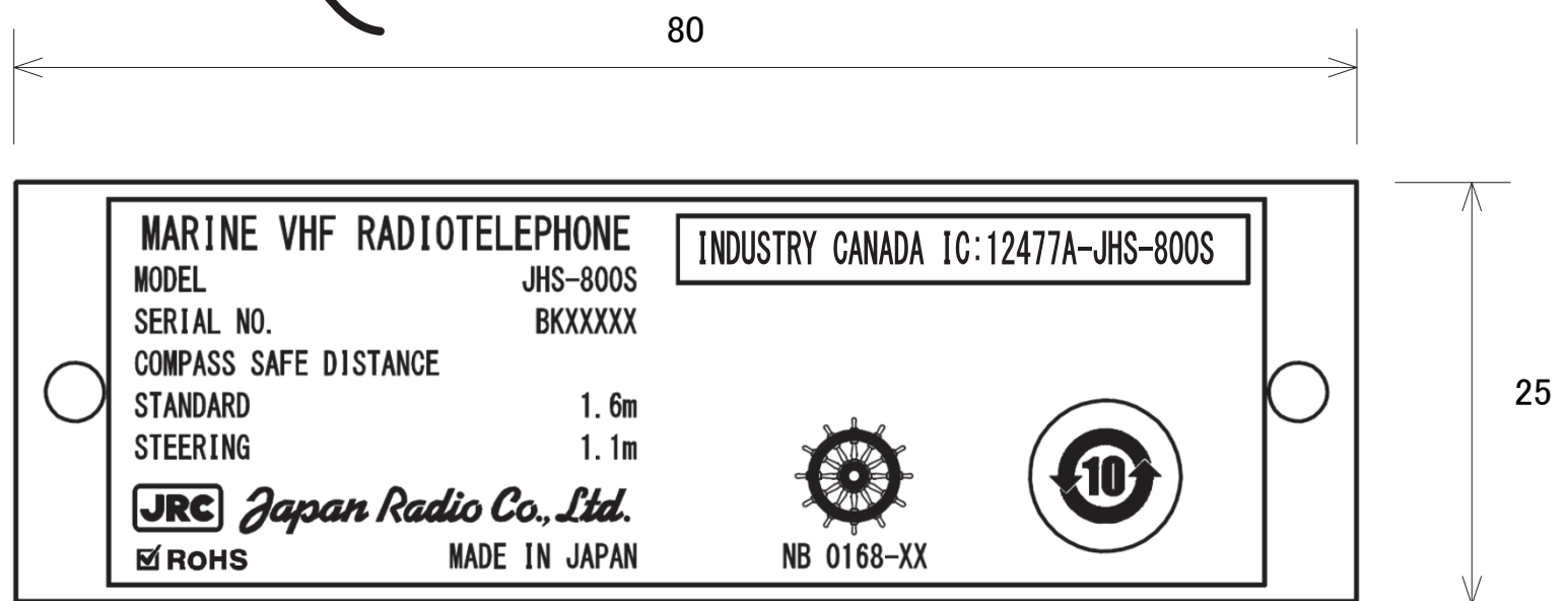
Name plate
